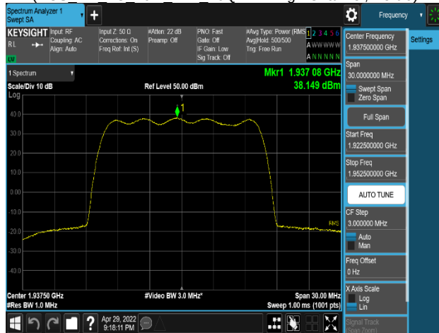
Plot 8-73. Power Spectral Density Plot (PCS DSS 2:8 1C 15M 2TX 16QAM - Low Channel, Port 0)
