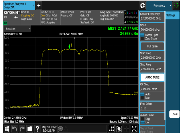
Plot 8-120. Power Spectral Density Plot
