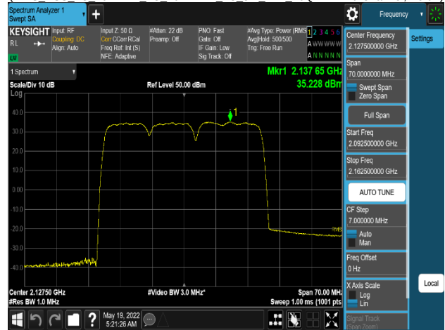
Plot 8-124. Power Spectral Density Plot
