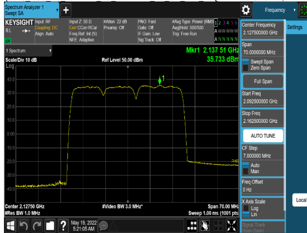
Plot 8-123. Power Spectral Density Plot
