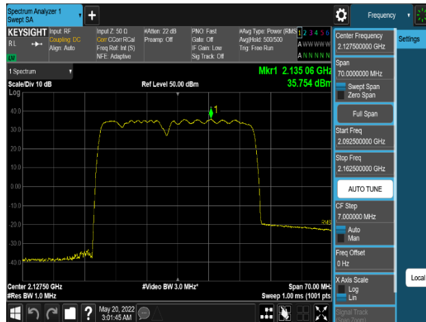
Plot 8-125. Power Spectral Density Plot
