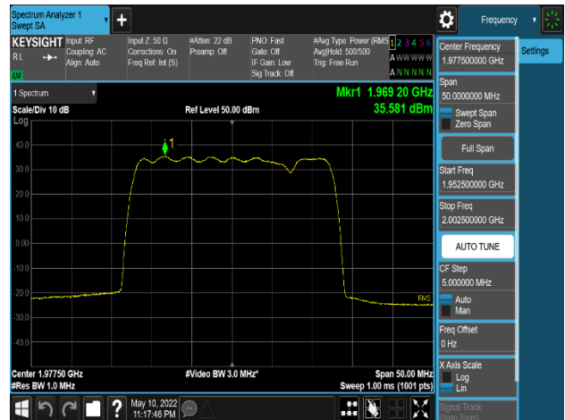
Plot 8-90. Power Spectral Density Plot
