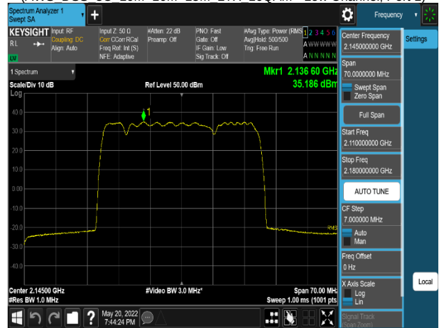
Plot 8-122. Power Spectral Density Plot
