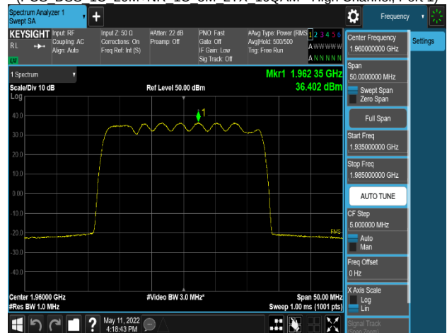
Plot 8-94. Power Spectral Density Plot
