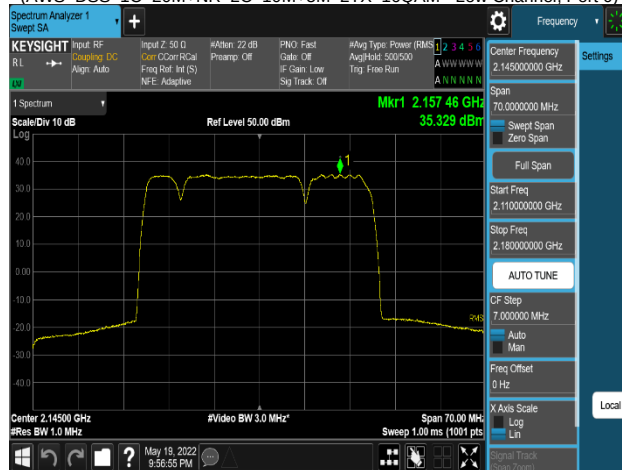
Plot 8-127. Power Spectral Density Plot
