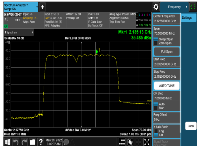
Plot 8-126. Power Spectral Density Plot
