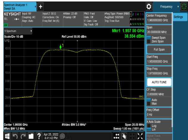
Plot 8-78. Power Spectral Density Plot (PCS_NR_2C_5M+5M_2TX_16QAM - Mid Channel, Port 1)
