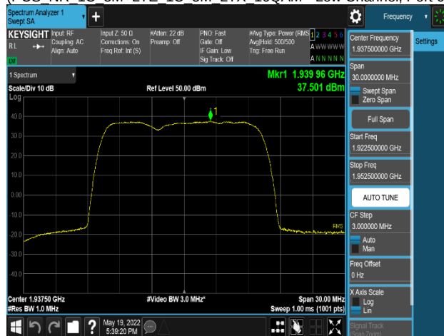
Plot 8-81. Power Spectral Density Plot (PCS_DSS_1C_10M+NR_1C_5M_2TX_16QAM - Low Channel, Port 0)
