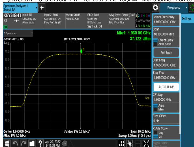
Plot 8-129. Power Spectral Density Plot
