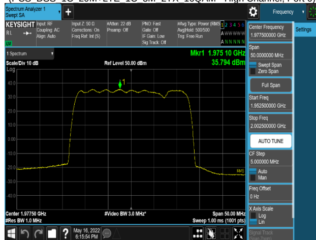
Plot 8-91. Power Spectral Density Plot
