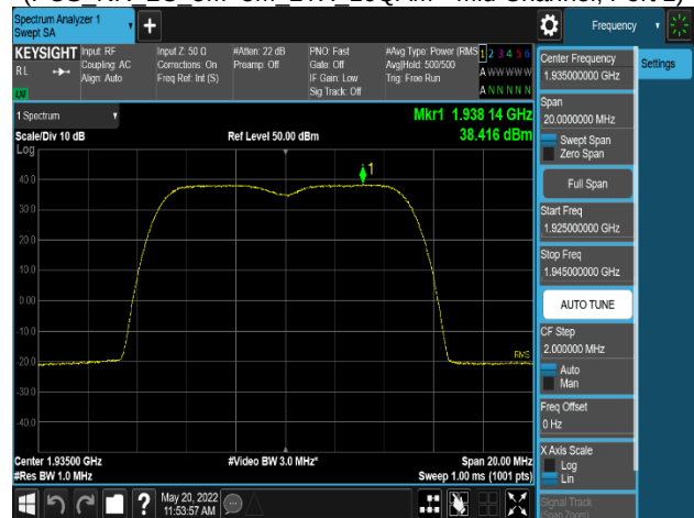
Plot 8-80. Power Spectral Density Plot (PCS_NR_1C_5M+LTE_1C_5M_2TX_16QAM - Low Channel, Port 1)
