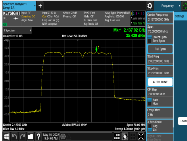
Plot 8-119. Power Spectral Density Plot
