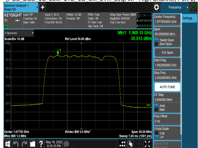
Plot 8-92. Power Spectral Density Plot
