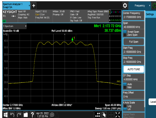
Plot 8-101. Power Spectral Density Plot (AWS_NR_1C_20M_2TX_16QAM – High Channel, Port 0)
