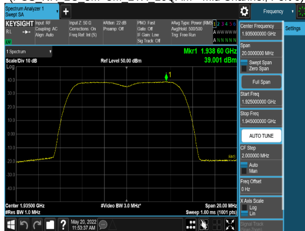
Plot 8-79. Power Spectral Density Plot (PCS_NR_1C_5M+LTE_1C_5M_2TX_16QAM - Low Channel, Port 0)
