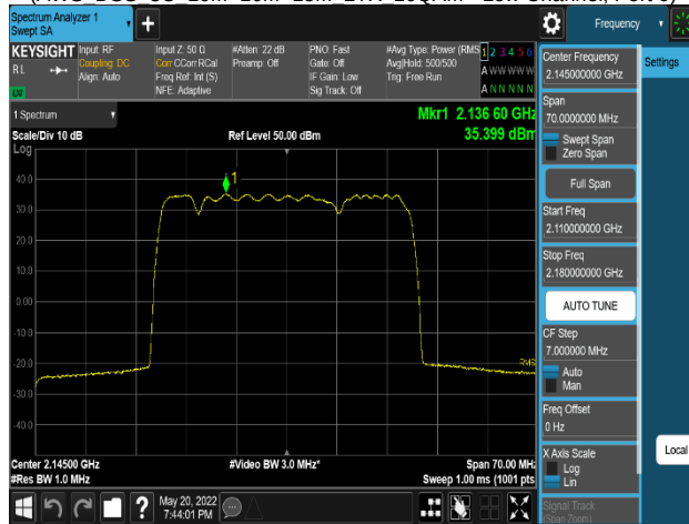
Plot 8-121. Power Spectral Density Plot
