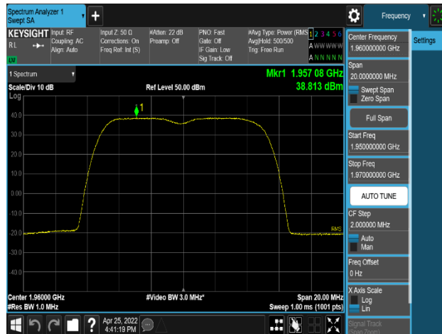
Plot 8-77. Power Spectral Density Plot (PCS_NR_2C_5M+5M_2TX_16QAM - Mid Channel, Port 0)
