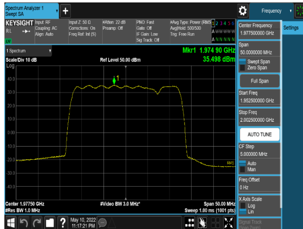
Plot 8-89. Power Spectral Density Plot
