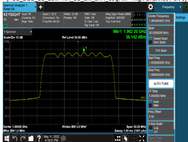
Plot 8-93. Power Spectral Density Plot
