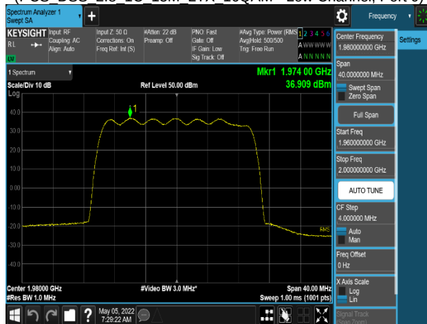
Plot 8-75. Power Spectral Density Plot (PCS DSS 2:8 1C 20M 2TX 16QAM - High Channel, Port 0)
