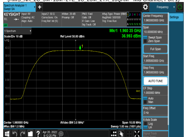
Plot 8-130. Power Spectral Density Plot
