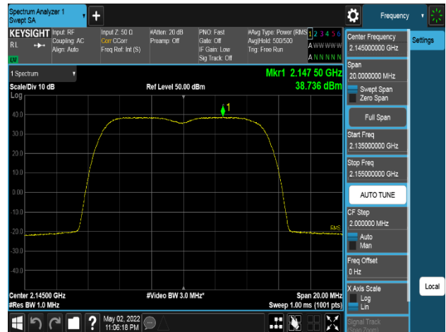
Plot 8-108. Power Spectral Density Plot (AWS_NR_2C_5M+5M_2TX_16QAM - Mid Channel, Port 1)
