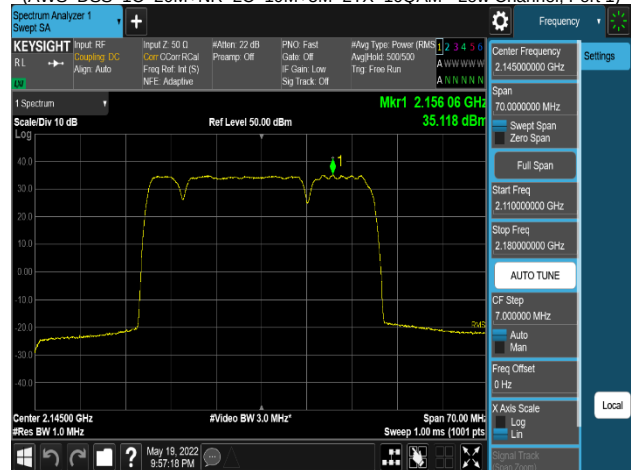
Plot 8-128. Power Spectral Density Plot
