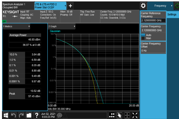
Plot 7-241. Peak To Average Power Ratio Plot (B66_20M+5M+10M_QPSK - Low Channel, Port 0)
