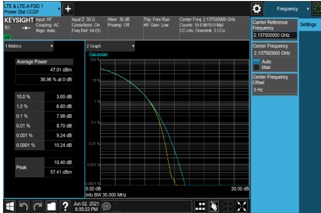
Plot 7-247. Peak To Average Power Ratio Plot (B66_20M+5M+10M_64QAM - Middle Channel, Port 0)
