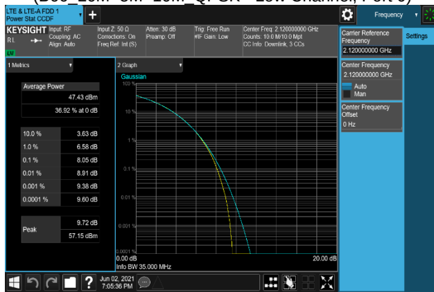
Plot 7-243. Peak To Average Power Ratio Plot (B66_20M+5M+10M_64QAM - Low Channel, Port 3)
