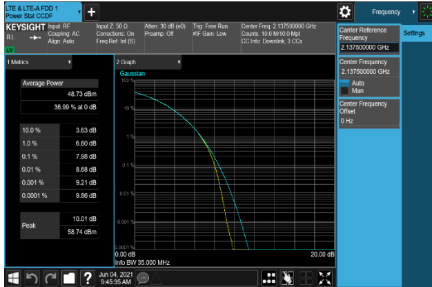
Plot 7-235. Peak To Average Power Ratio Plot (B66_20M+5M+10M_64QAM - Middle Channel, Port 0)
