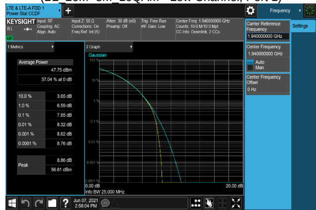
Plot 7-256. Peak To Average Power Ratio Plot (B2_20M+5M_256QAM - Low Channel, Port 1)
