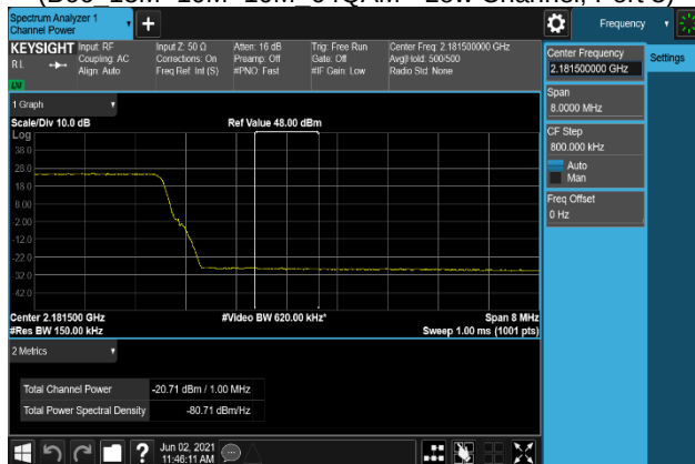
Plot 7-297. Band Edge Emission(Channel Power) Plot 2181 MHz to 2182 MHz
