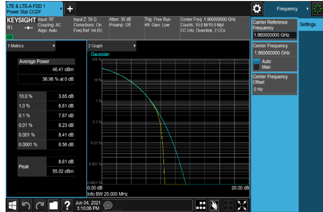
Plot 7-272. Peak To Average Power Ratio Plot (B2_20M+5M_256QAM - Middle Channel, Port 0)
