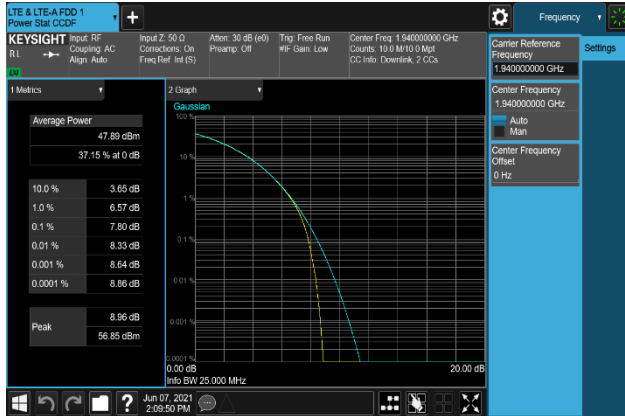
Plot 7-253. Peak To Average Power Ratio Plot (B2_20M+5M_QPSK - Low Channel, Port 0)
