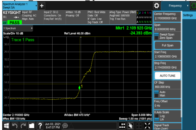
Plot 7-287. Band Edge Emission Plot 2109 MHz to 2110 MHz
