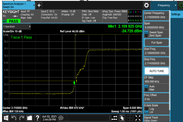
Plot 7-303. Band Edge Emission Plot 2109 MHz to 2110 MHz
