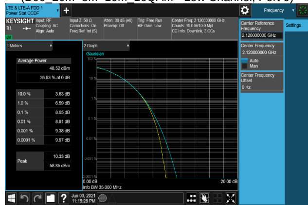
Plot 7-232. Peak To Average Power Ratio Plot (B66_20M+5M+10M_256QAM - Low Channel, Port 0)
