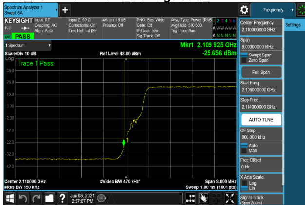
Plot 7-293. Band Edge Emission Plot 2109 MHz to 2110 MHz
