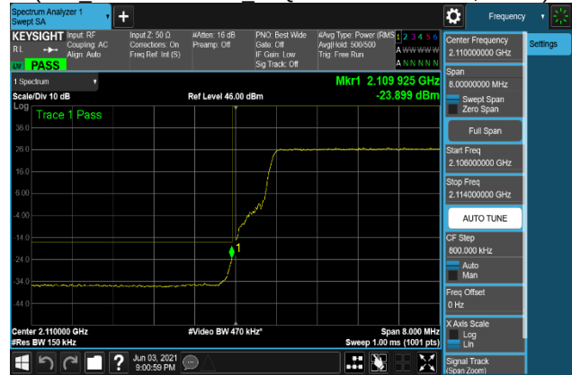
Plot 7-288. Band Edge Emission Plot 2109 MHz to 2110 MHz
