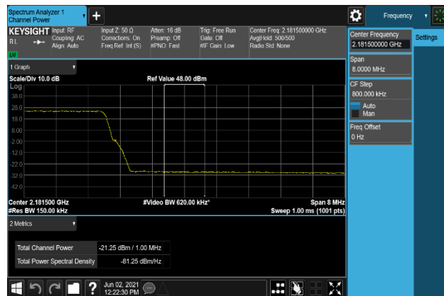
Plot 7-300. Band Edge Emission(Channel Power) Plot 2181 MHz to 2182 MHz (B66_15M+10M+10M_256QAM – High Channel, Port 2)
