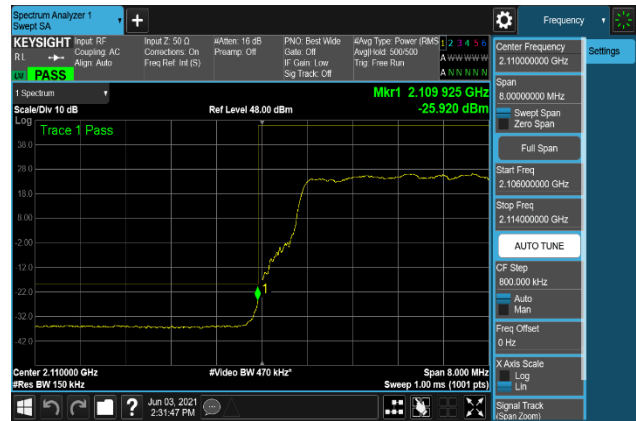
Plot 7-294. Band Edge Emission Plot 2109 MHz to 2110 MHz
