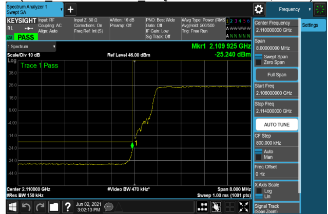
Plot 7-304. Band Edge Emission Plot 2109 MHz to 2110 MHz
