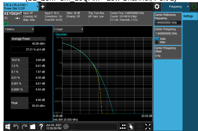
Plot 7-268. Peak To Average Power Ratio Plot (B2_20M+5M_256QAM - Low Channel, Port 1)
