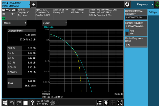
Plot 7-259. Peak To Average Power Ratio Plot (B2_20M+5M_64QAM - Middle Channel, Port 0)
