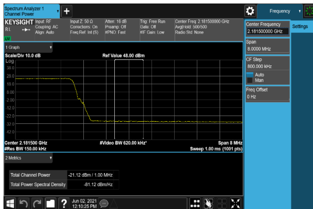
Plot 7-299. Band Edge Emission(Channel Power) Plot 2181 MHz to 2182 MHz (B66_15M+10M+10M_64QAM – High Channel, Port 0)
