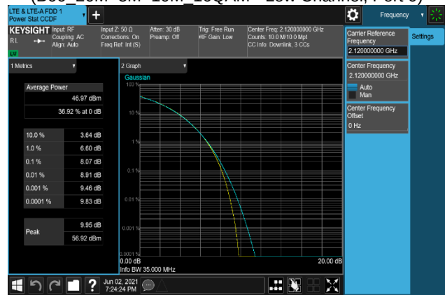
Plot 7-244. Peak To Average Power Ratio Plot (B66_20M+5M+10M_256QAM - Low Channel, Port 0)
