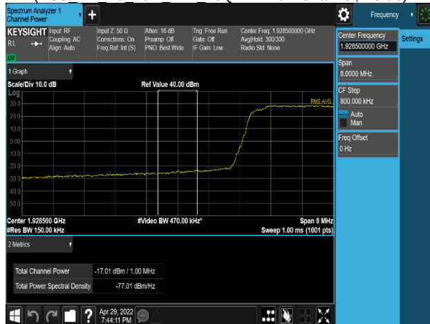
Plot 8-293. Band Edge Emission Plot (PCS DSS 5:5 1C 15M 2TX 64QAM - Low Channel, Port 0)
