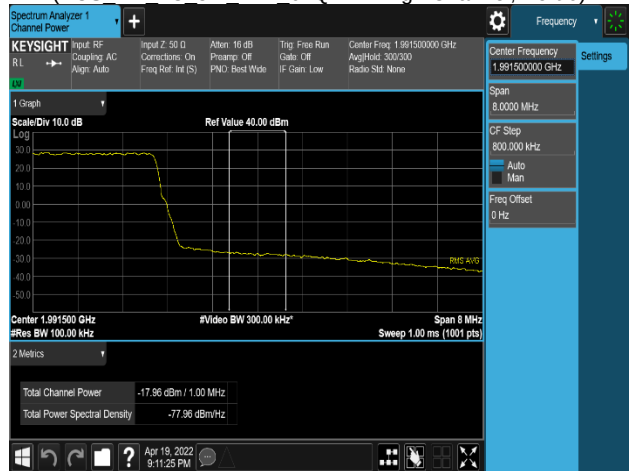
Plot 8-288. Band Edge Emission Plot (PCS NR 1C 5M 2TX 64QAM - High Channel, Port 0)
