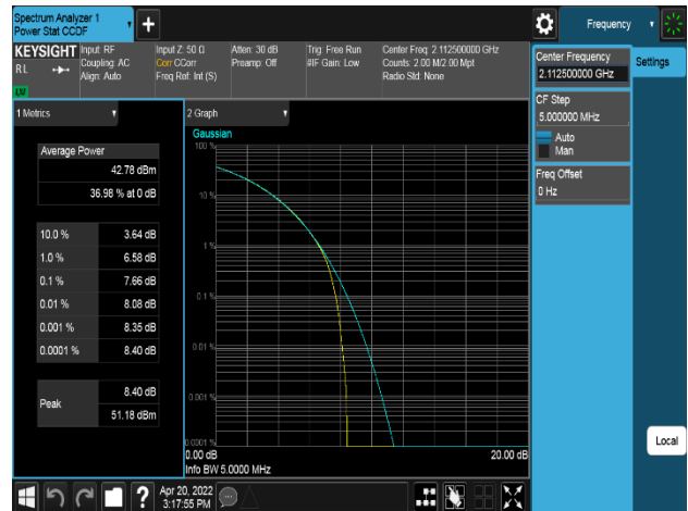
Plot 8-264. Peak To Average Power Ratio Plot (AWS NR 1C 5M 2TX 64QAM - Low Channel, Port 1)
