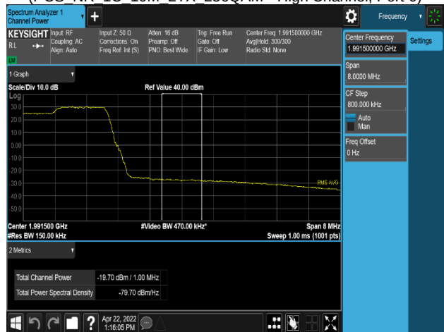
Plot 8-290. Band Edge Emission Plot (PCS NR 1C 10M 2TX 256QAM - High Channel, Port 0)
