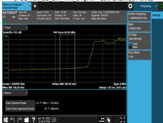
Plot 8-317. Band Edge Emission Plot (PCS_NR_1C_5M_4TX 64QAM - Low Channel, Port 1)
