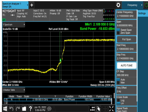
Plot 8-315. Band Edge Emission Plot (AWS_NR_1C_5M+LTE_1C_5M_2TX Non-Cont QPSK - Low Channel, Port 0)
