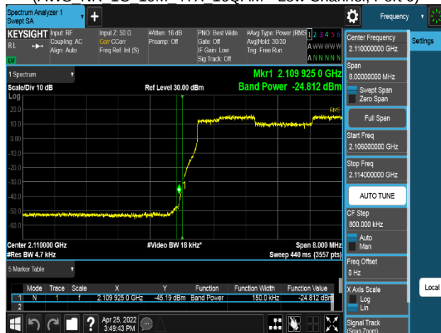
Plot 8-337. Band Edge Emission Plot (AWS_NR_1C_15M_4TX_16QAM - Low Channel, Port 0)
