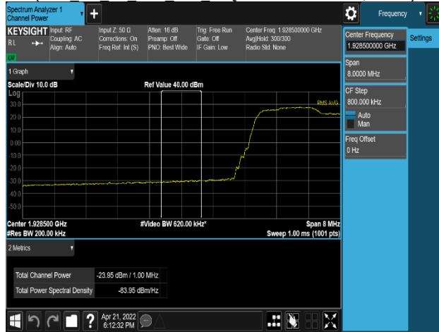
Plot 8-323. Band Edge Emission Plot (PCS_NR_1C_20M_4TX_16QAM - Low Channel, Port 2)
