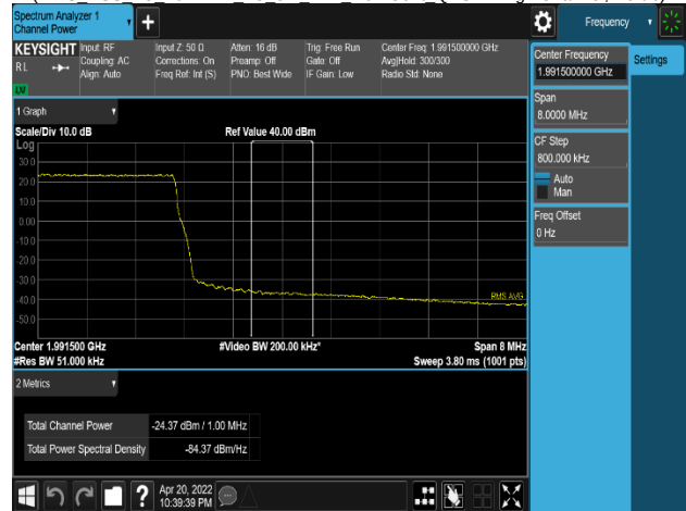
Plot 8-320. Band Edge Emission Plot (PCS_NR_1C_10M_4TX_256QAM - High Channel, Port 0)
