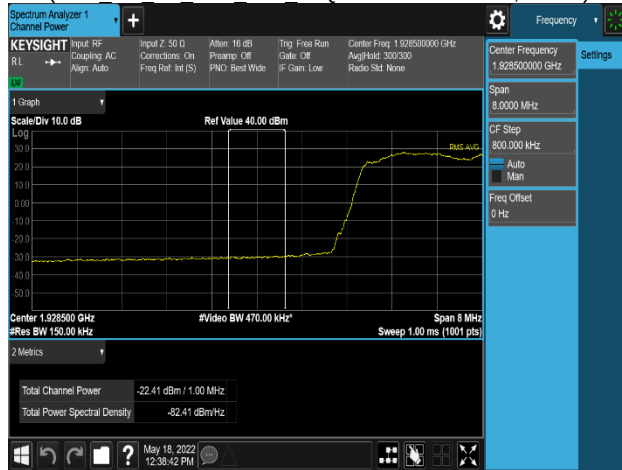
Plot 8-325. Band Edge Emission Plot (PCS_DSS_5:5_1C_15M_4TX_16QAM - Low Channel, Port 3)
