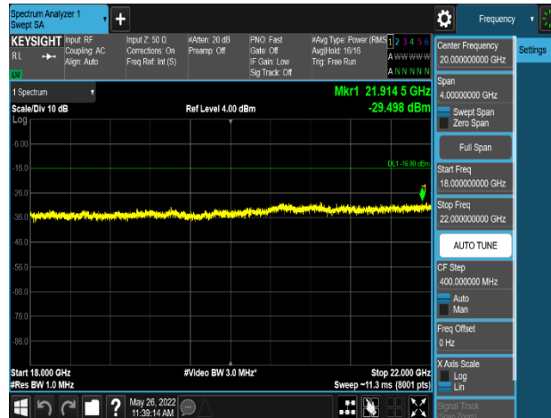
Plot 8-355. Conducted Spurious Emission Plot 18 GHz to 22 GHz (PCS_NR_1C_5M_2TX_64QAM - Low Channel, Port 0)
