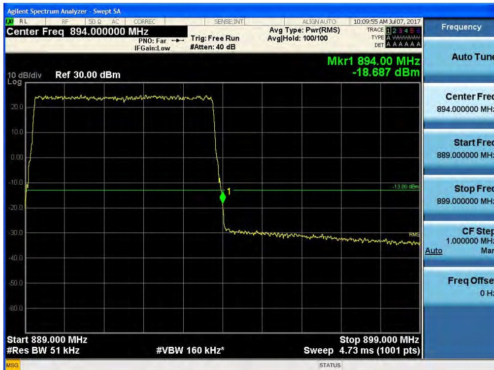
(64QAM High)
