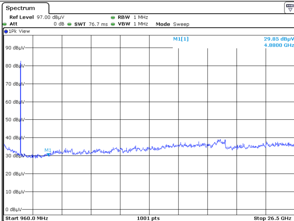
Radiated Emission - Middle Channel _ H
