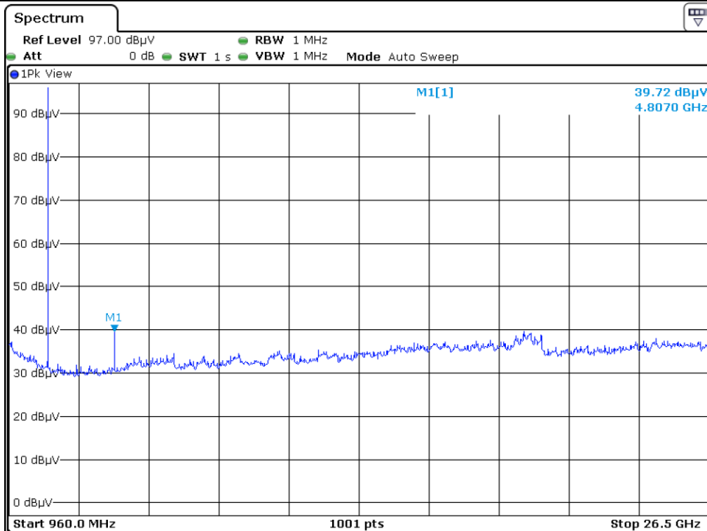
Radiated Emission - Low Channel _ H
