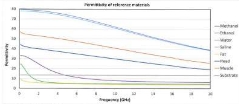
Fig. B.1 Permittivity of reference materials
