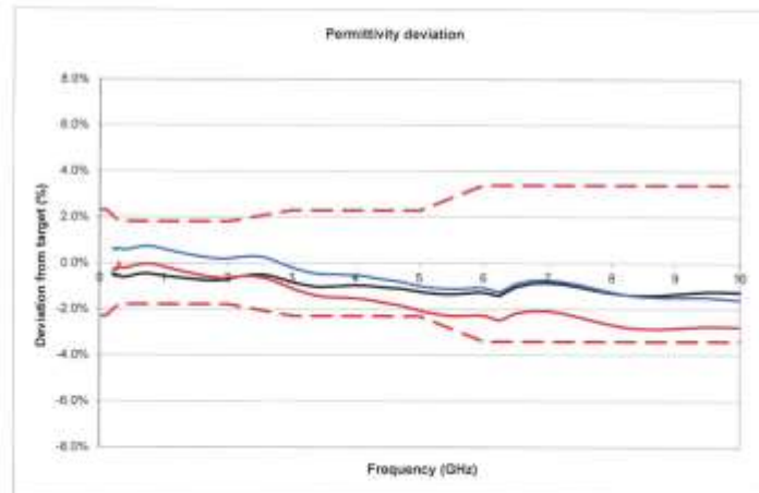
Fig. 3.1 Methanol permittivity deviation from target, 200 MHz – 10 GHz
