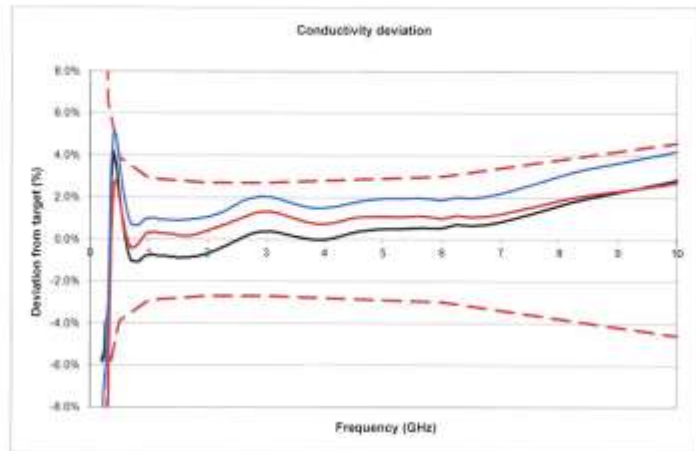
Fig. 3.2 Methanol conductivity deviation from target, 200 MHz – 10 GHz
