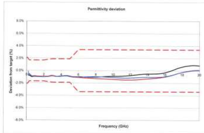
Fig. 4.1 HBBL permittivity deviation from target, 200 MHz – 20 GHz
