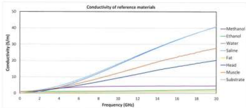
Fig. B.2 Conductivity of reference materials
