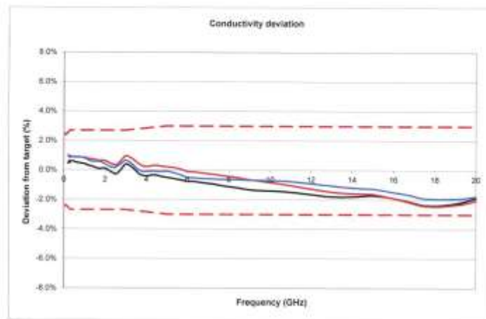
Fig. 4.2 HBBL conductivity deviation from target, 200 MHz – 20 GHz
