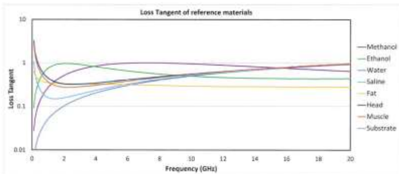
Fig. B.3 Loss tangent of reference materials
