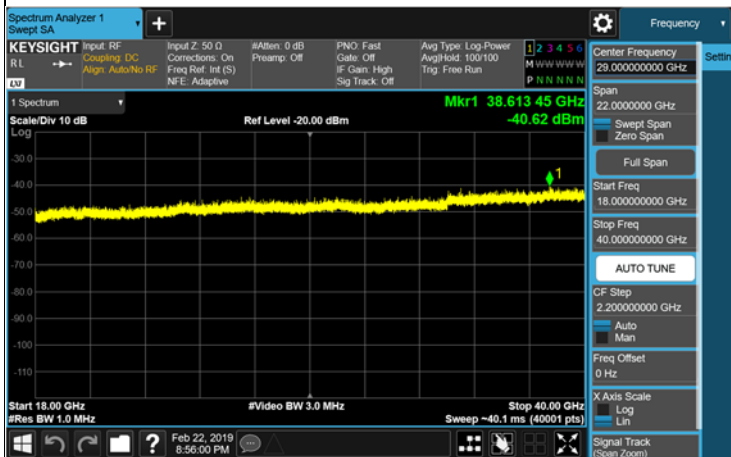
18 GHz ~ 40 GHz Peak
