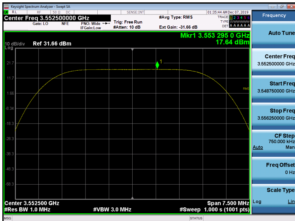
Plot 7-72. Peak Power Spectral Density Plot (1CC Configuration 5MHz 64QAM - Low Channel) Port 03
