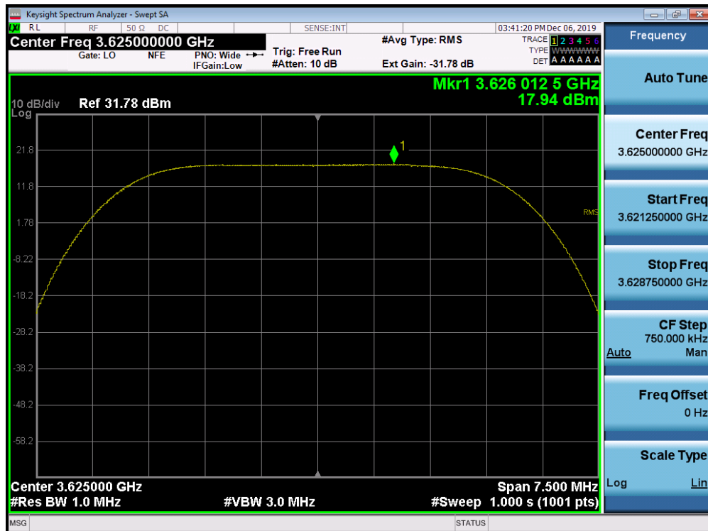
Plot 7-90. Peak Power Spectral Density Plot (1CC Configuration 5MHz 256QAM - Mid Channel) Port 01
