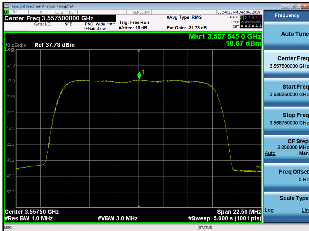
Plot 7-114. Peak Power Spectral Density Plot (1CC Configuration 15MHz 16QAM - Low Channel) Port 01
