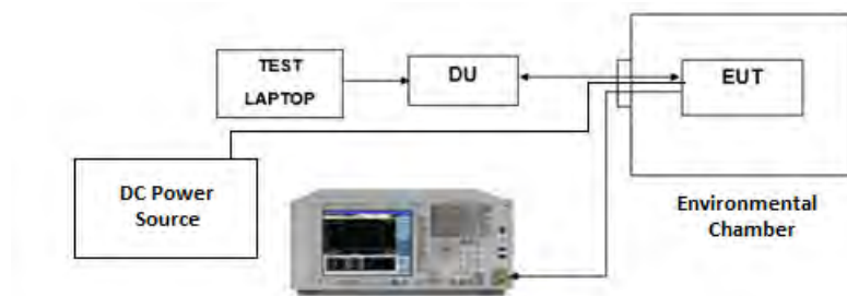
Figure 7-8. Test Instrument & Measurement Setup
