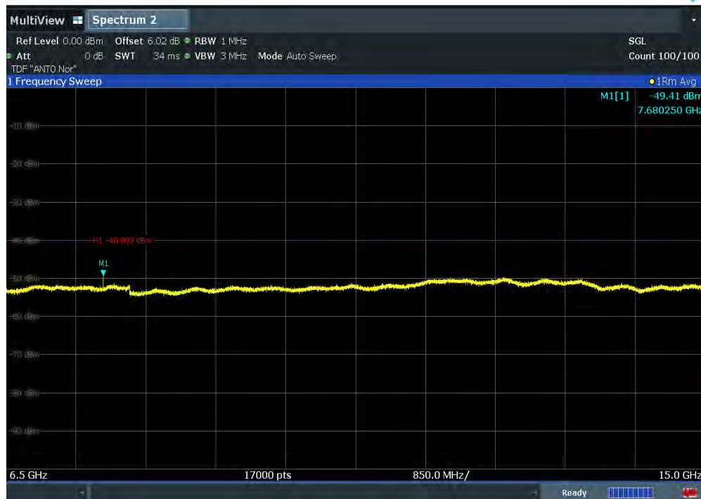
Plot 7-202. Conducted Spurious Emission at Antenna Port (75MHz Total Bandwidth 16QAM - Mid Channel, 6.5G ~ 15GHz)
