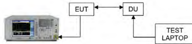
Figure 7-7. Test Instrument & Measurement Setup
