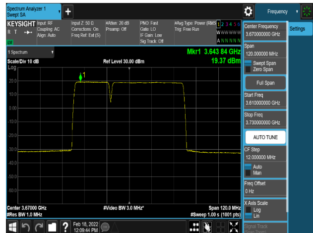
Plot 8-88. Power Spectral Density Plot (NR_n48_2C_20M+40M_256QAM – High Channel, Port 1)
