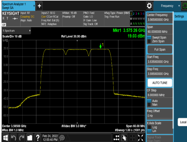
Plot 8-107. Power Spectral Density Plot (LTE_2C+NR_1C_10M+10M+10M_256QAM-Low Channel, Port 0)
