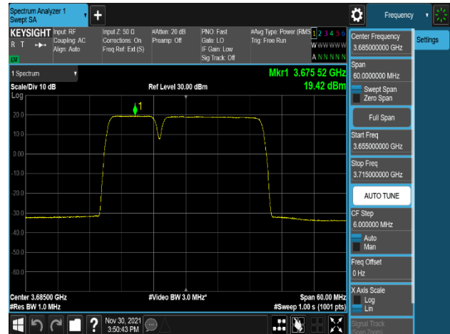
Plot 8-74. Power Spectral Density Plot (NR_n48_2C_10M+20M_256QAM – High Channel, Port 3)
