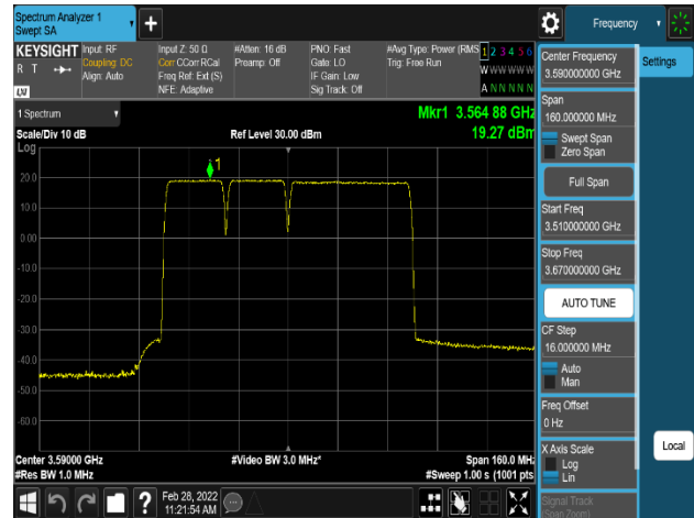
Plot 8-114. Power Spectral Density Plot (LTE_2C+NR_1C_20M+20M+40M_16QAM-Low Channel, Port 3)
