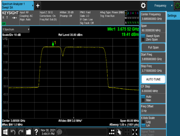
Plot 8-71. Power Spectral Density Plot (NR_n48_2C_10M+20M_256QAM – High Channel, Port 0)
