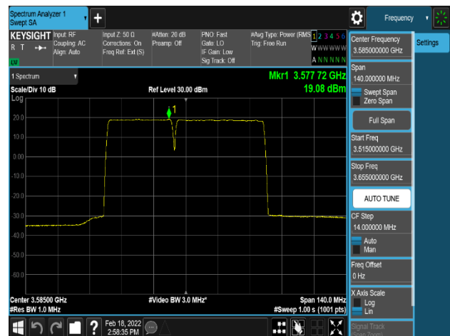
Plot 8-94. Power Spectral Density Plot (NR_n48_2C_30M+40M_16QAM – Low Channel, Port 3)
