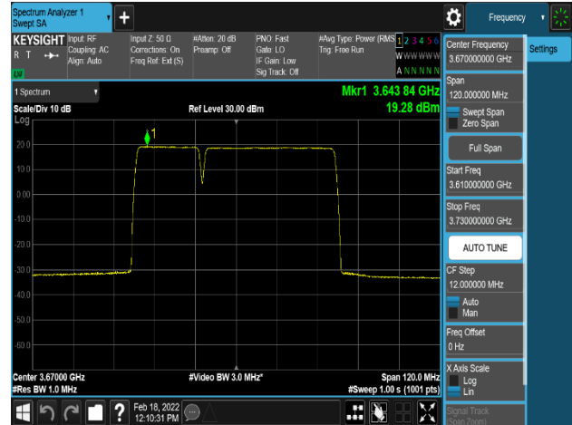
Plot 8-90. Power Spectral Density Plot (NR_n48_2C_20M+40M_256QAM – High Channel, Port 3)
