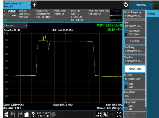
Plot 8-84. Power Spectral Density Plot (NR_n48_2C_10M+40M_64QAM – High Channel, Port 0)
