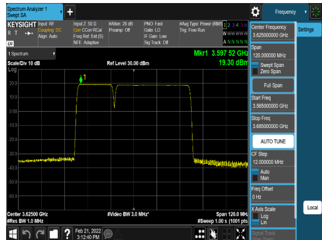
Plot 8-106. Power Spectral Density Plot (LTE_1C+NR_1C_20M+40M_QPSK - Mid Channel, Port 3)
