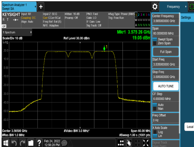
Plot 8-109. Power Spectral Density Plot (LTE_2C+NR_1C_10M+10M+10M_256QAM-Low Channel, Port 2)
