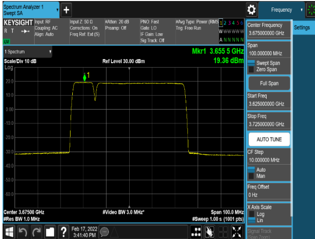
Plot 8-83. Power Spectral Density Plot (NR_n48_2C_10M+40M_64QAM – High Channel, Port 0)
