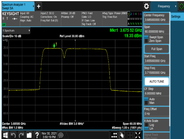
Plot 8-73. Power Spectral Density Plot (NR_n48_2C_10M+20M_256QAM – High Channel, Port 2)
