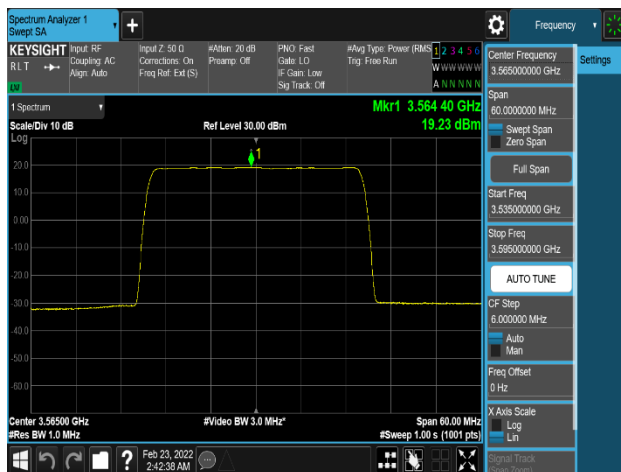
Plot 8-57. Power Spectral Density Plot (NR_n48_1C_30M_16QAM - Low Channel, Port 2)
