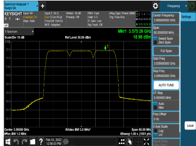
Plot 8-108. Power Spectral Density Plot (LTE_2C+NR_1C_10M+10M+10M_256QAM-Low Channel, Port 1)
