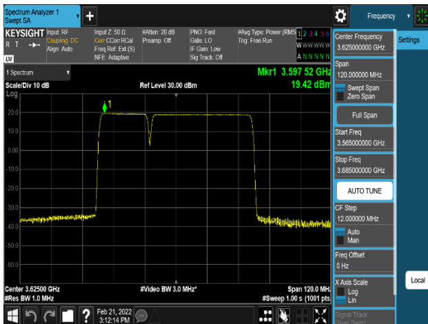
Plot 8-105. Power Spectral Density Plot (LTE_1C+NR_1C_20M+40M_QPSK - Mid Channel, Port 2)
