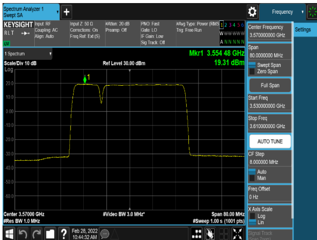
Plot 8-75. Power Spectral Density Plot (NR_n48_2C_10M+30M_16QAM – Low Channel, Port 0)
