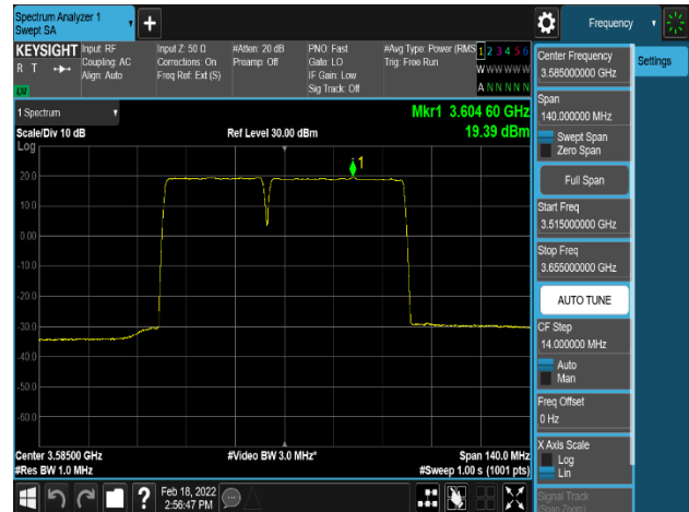
Plot 8-92. Power Spectral Density Plot (NR_n48_2C_30M+40M_16QAM – Low Channel, Port 1)
