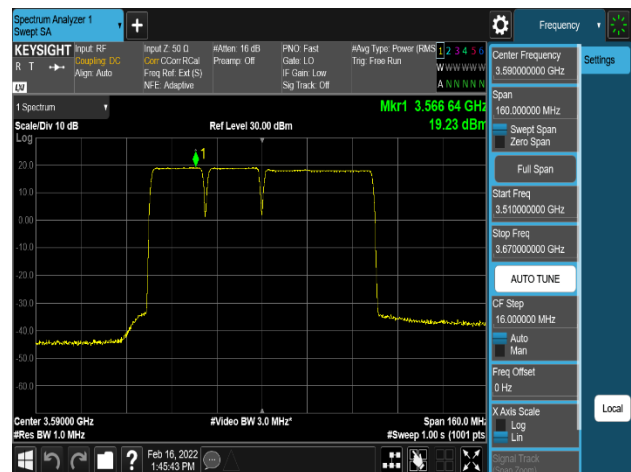
Plot 8-112. Power Spectral Density Plot (LTE_2C+NR_1C_20M+20M+40M_16QAM-Low Channel, Port 1)
