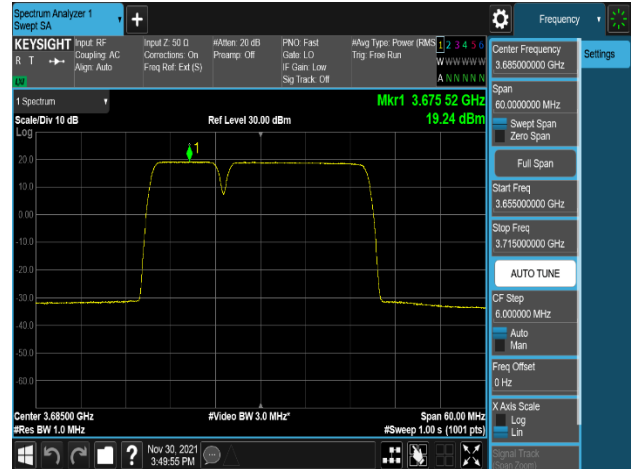
Plot 8-72. Power Spectral Density Plot (NR_n48_2C_10M+20M_256QAM – High Channel, Port 1)
