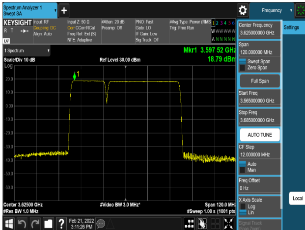
Plot 8-103. Power Spectral Density Plot (LTE_1C+NR_1C_20M+40M_QPSK - Mid Channel, Port 0)
