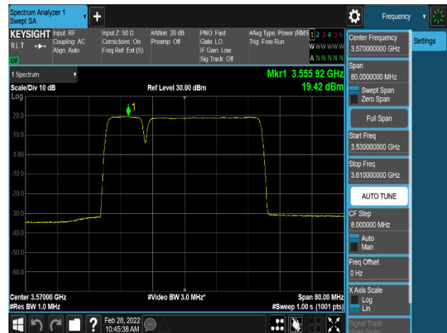
Plot 8-76. Power Spectral Density Plot (NR_n48_2C_10M+30M_16QAM – Low Channel, Port 1)
