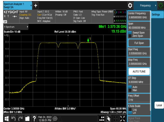
Plot 8-110. Power Spectral Density Plot (LTE_2C+NR_1C_10M+10M+10M_256QAM-Low Channel, Port 3)
