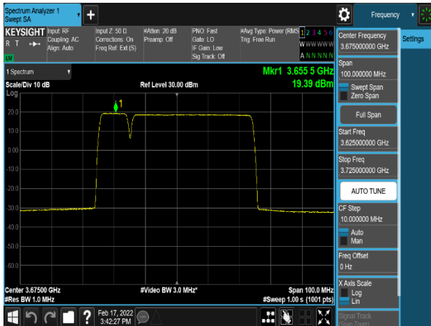
Plot 8-85. Power Spectral Density Plot (NR_n48_2C_10M+40M_64QAM – High Channel, Port 0)
