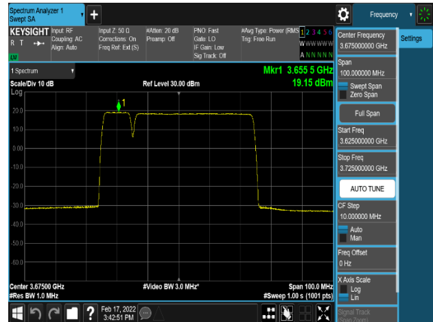
Plot 8-86. Power Spectral Density Plot (NR_n48_2C_10M+40M_64QAM – High Channel, Port 0)
