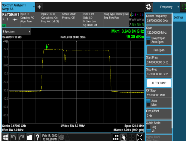
Plot 8-87. Power Spectral Density Plot (NR_n48_2C_20M+40M_256QAM – High Channel, Port 0)
