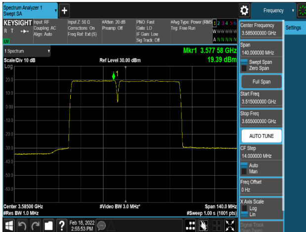
Plot 8-91. Power Spectral Density Plot (NR_n48_2C_30M+40M_16QAM – Low Channel, Port 0)
