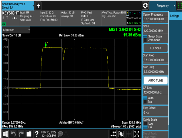
Plot 8-89. Power Spectral Density Plot (NR_n48_2C_20M+40M_256QAM – High Channel, Port 2)
