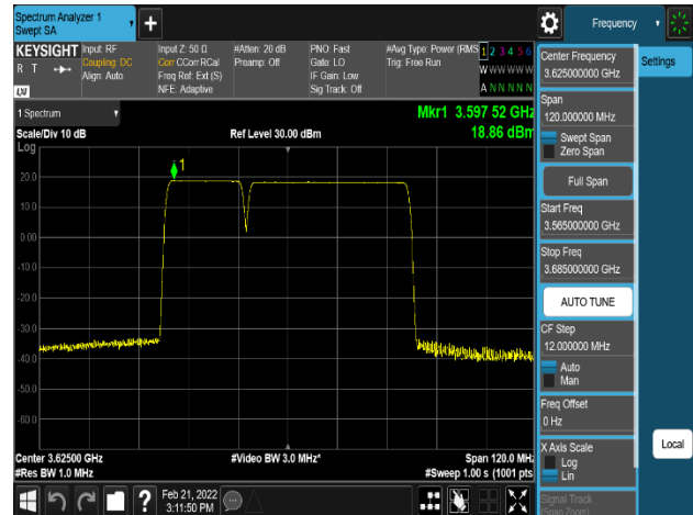
Plot 8-104. Power Spectral Density Plot (LTE_1C+NR_1C_20M+40M_QPSK - Mid Channel, Port 1)
