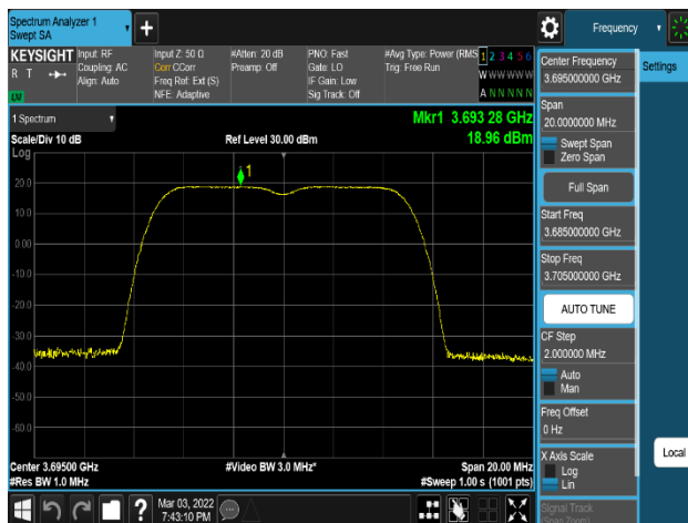
Plot 8-63. Power Spectral Density Plot (LTE_B48_2C_5M+5M_16QAM - High Channel, Port 0)
