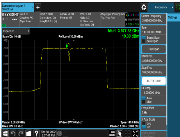
Plot 8-93. Power Spectral Density Plot (NR_n48_2C_30M+40M_16QAM – Low Channel, Port 2)
