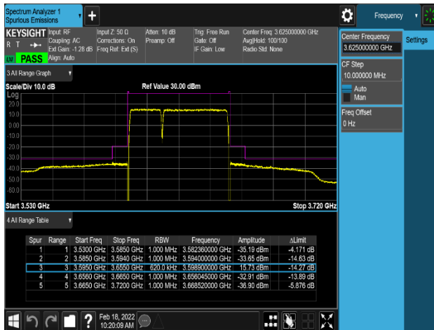
Plot 8-232. Channel Edge Emission Plot (NR_n48_2C_20M+40M_QPSK – Mid Channel, Port 0)
