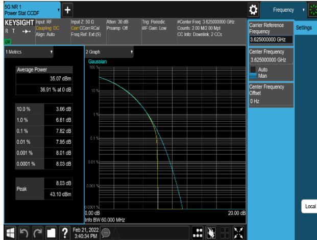
Plot 8-207. Peak To Average Power Ratio Plot (LTE_1C+NR_1C_20M+40M_QPSK - Mid Channel, Port0)
