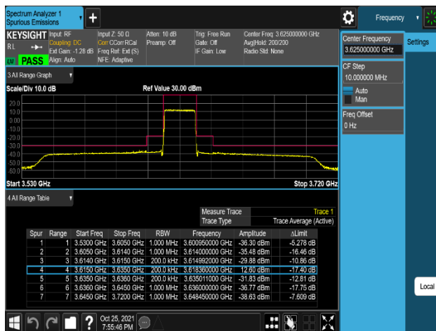
Plot 8-217. Channel Edge Emission Plot (NR_n48_1C_20M_64QAM – Mid Channel, Port 3)
