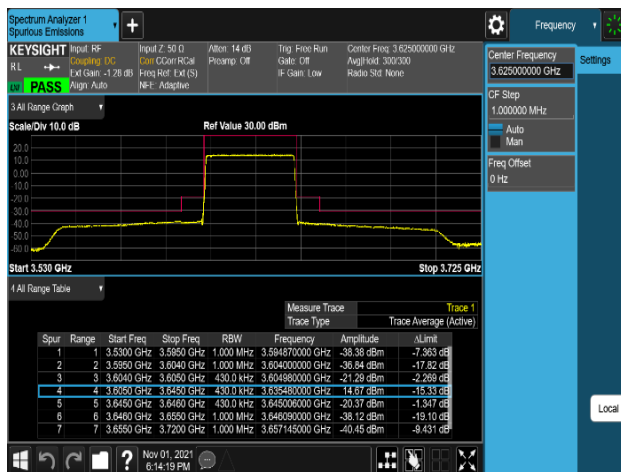
Plot 8-223. Channel Edge Emission Plot (NR_n48_1C_40M_256QAM – Mid Channel, Port 1)
