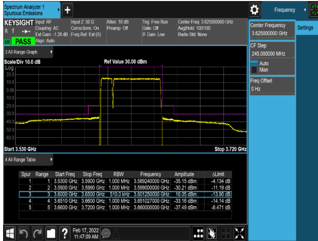
Plot 8-230. Channel Edge Emission Plot (NR_n48_2C_10M+40M_QPSK – Mid Channel, Port 0)
