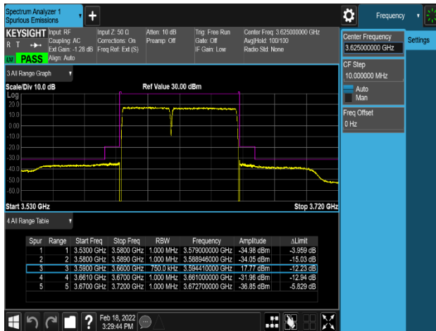
Plot 8-234. Channel Edge Emission Plot (NR_n48_2C_30M+40M_QPSK – Mid Channel, Port 0)
