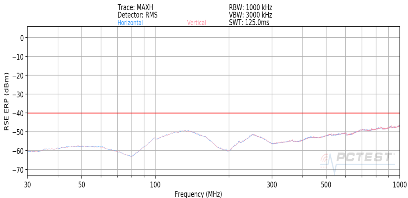
Plot 8-292. Radiated spurious emission Plot_30 MHz to 1000 MHz (NR_n48_1C_40M_QPSK - Mid Channel)
