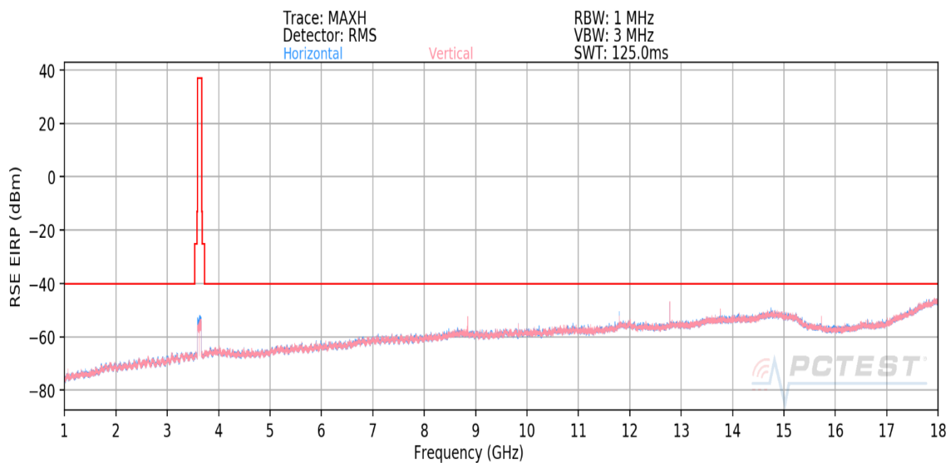
Plot 8-297. Radiated spurious emission Plot_1 GHz to 18 GHz (NR_n48_2C_40M+40M_QPSK - Mid Channel)
