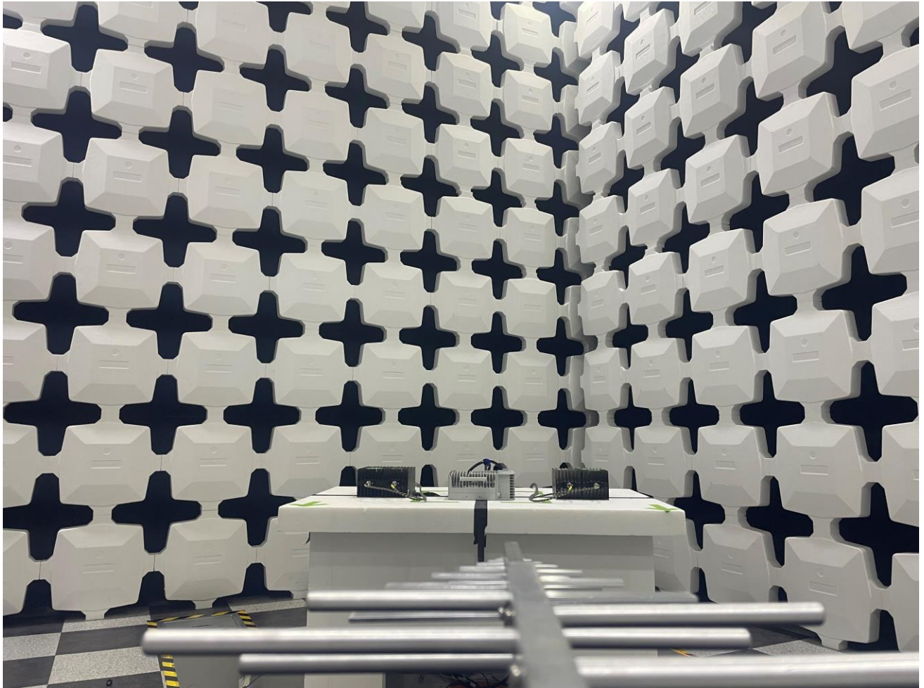
Below 1GHz Test Instrument & Measurement Setup
