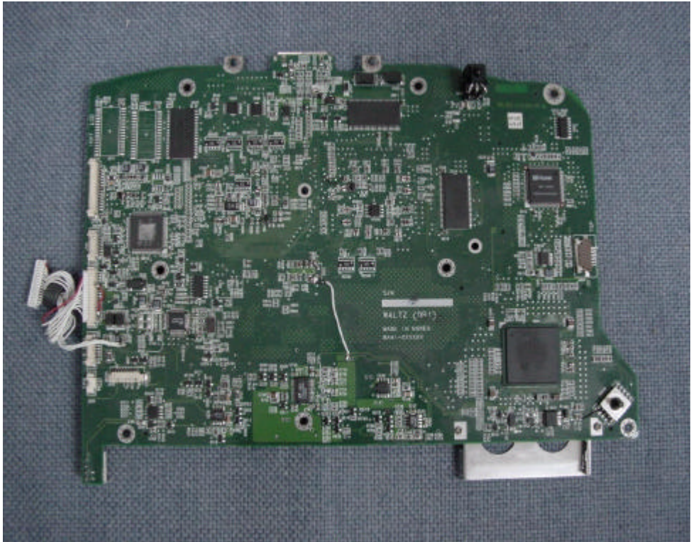
Rear view of Main PCB
