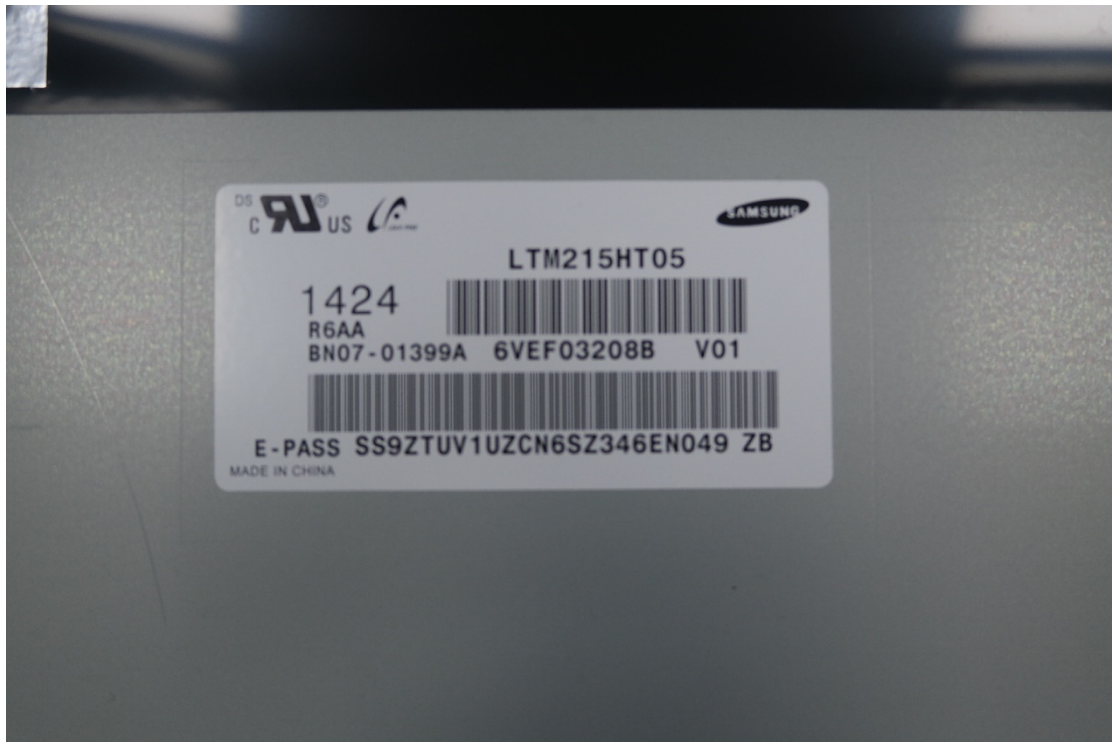
Before change LTM215HT05 rear view
