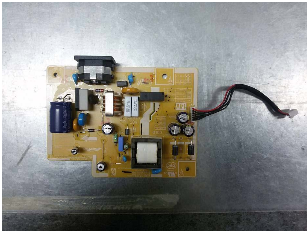
Before change P2514Z_FPN R.B rear view
