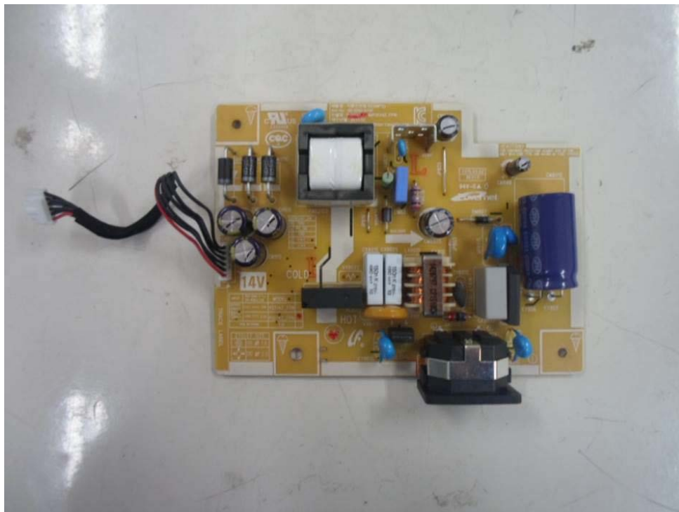
Before change P3514Z_FPN R.B rear view
