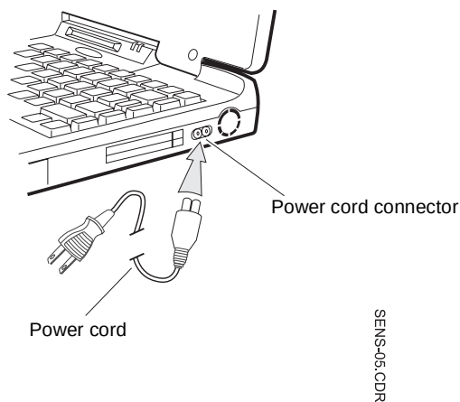
Figure 5. Connecting the Power Cord
