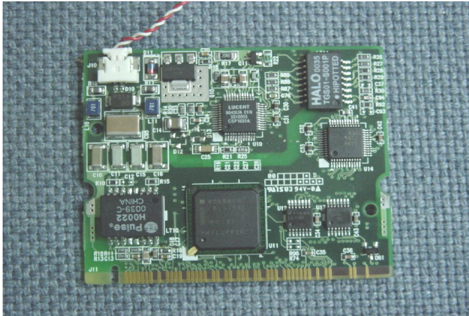
Front side of Mini PCI LAN/Modem Combo Card
