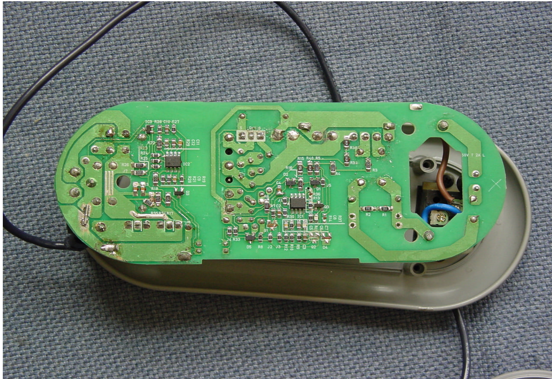
Rear view of Adapter
