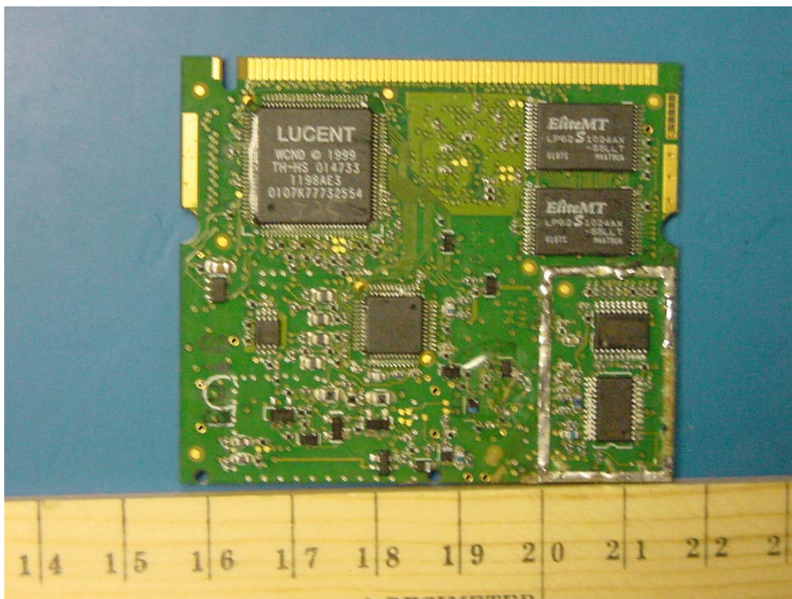
PHOTOGRAPH 6: BOTTOM VIEW OF THE BOARD WITHOUT CAN
