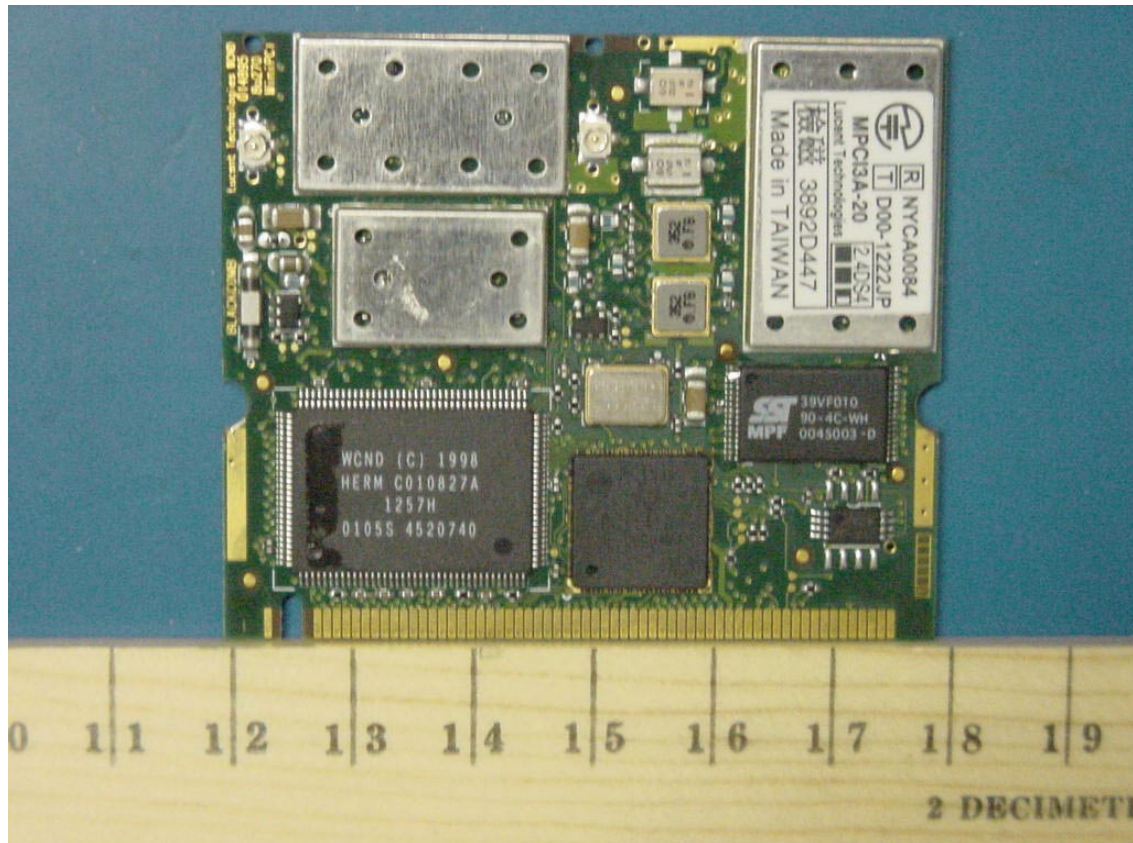
PHOTOGRAPH 3: TOP VIEW
