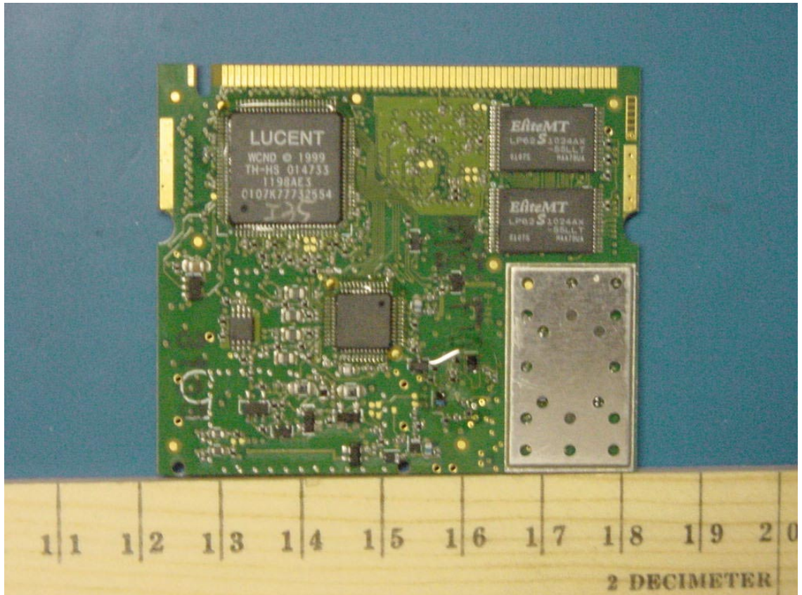
PHOTOGRAPH 4: BOTTOM VIEW
