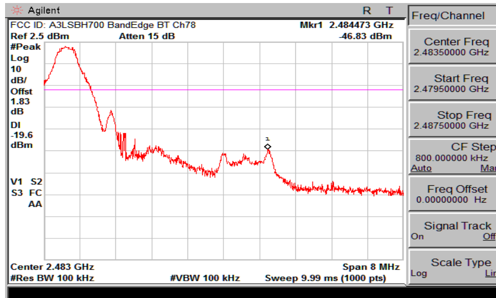
Plot 6-5. Band Edge Plot (Bluetooth – Ch. 78)
