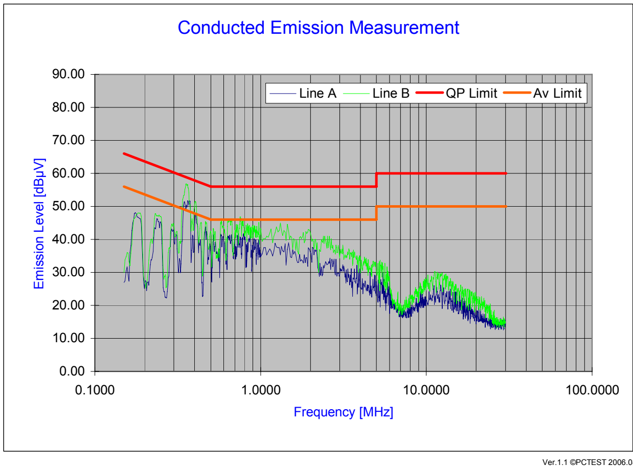
Plot 6-16. Line Conducted Plot with Bluetooth
