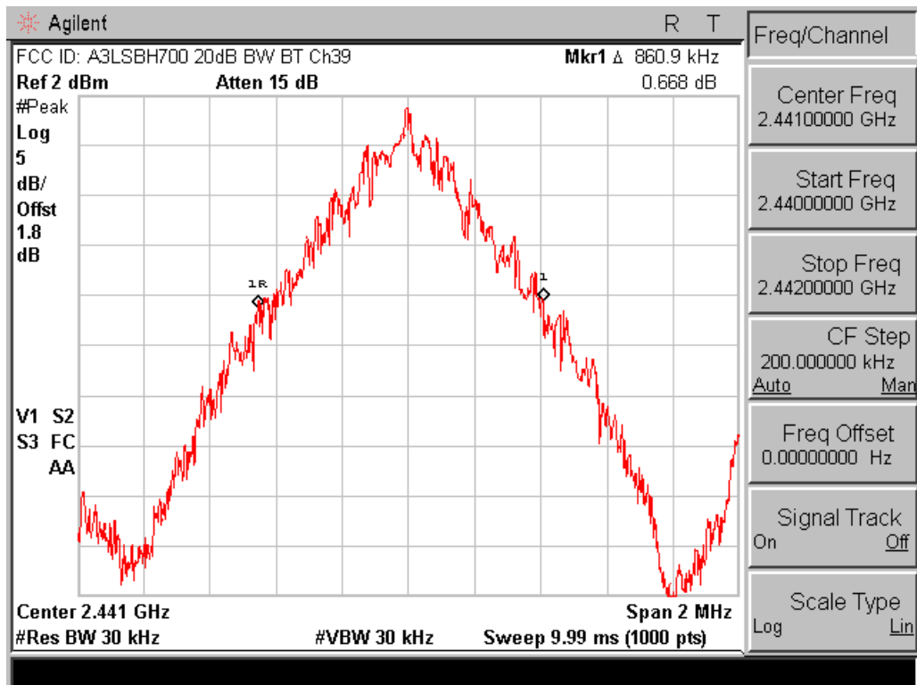
Plot 6-2. 20dB Bandwidth Plot (Ch. 39)
