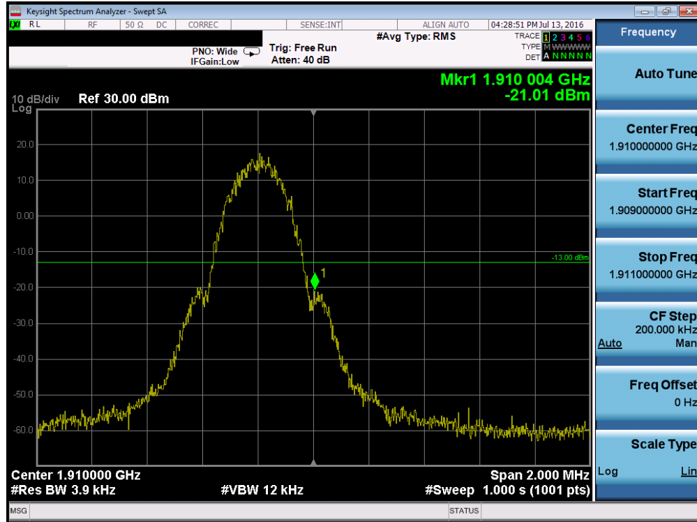
Plot 7-37. Band Edge Plot (PCS GPRS Mode – Ch. 810)
