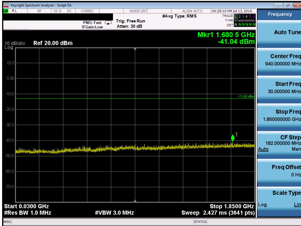
Plot 7-21. Conducted Spurious Plot (PCS GPRS Mode – Ch. 810)
