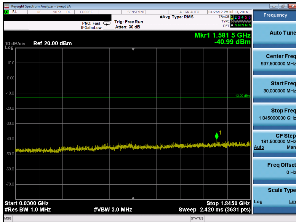
Plot 7-15. Conducted Spurious Plot (PCS GPRS Mode – Ch. 512)
