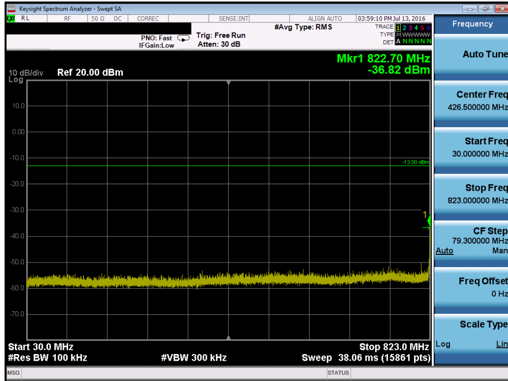
Plot 7-6. Conducted Spurious Plot (Cellular GPRS Mode – Ch. 128)
