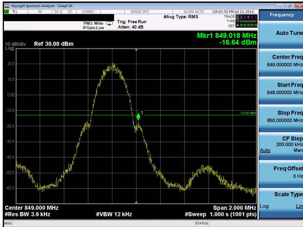
Plot 7-34. Band Edge Plot (Cellular GPRS Mode – Ch. 251)
