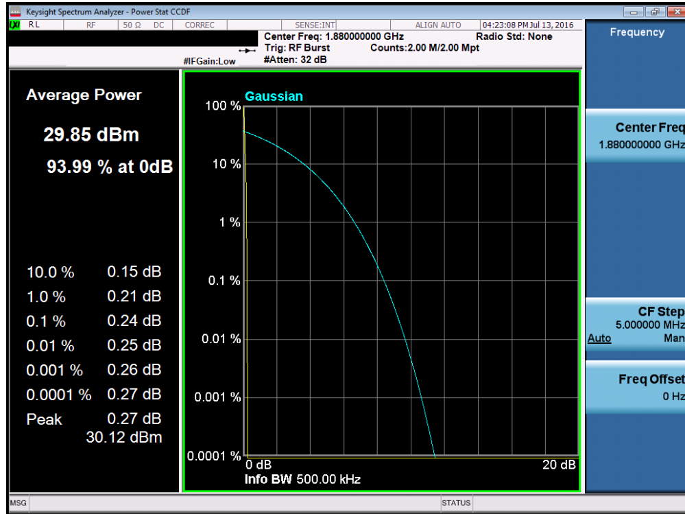
Plot 7-41. Peak-Average Ratio Plot (PCS GPRS Mode – Ch. 661)
