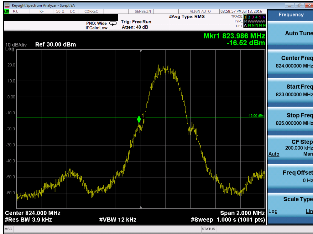
Plot 7-33. Band Edge Plot (Cellular GPRS Mode – Ch. 128)
