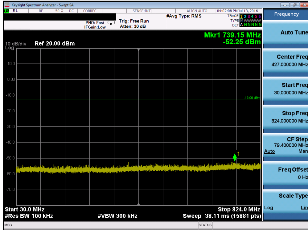
Plot 7-12. Conducted Spurious Plot (Cellular GPRS Mode – Ch. 251)
