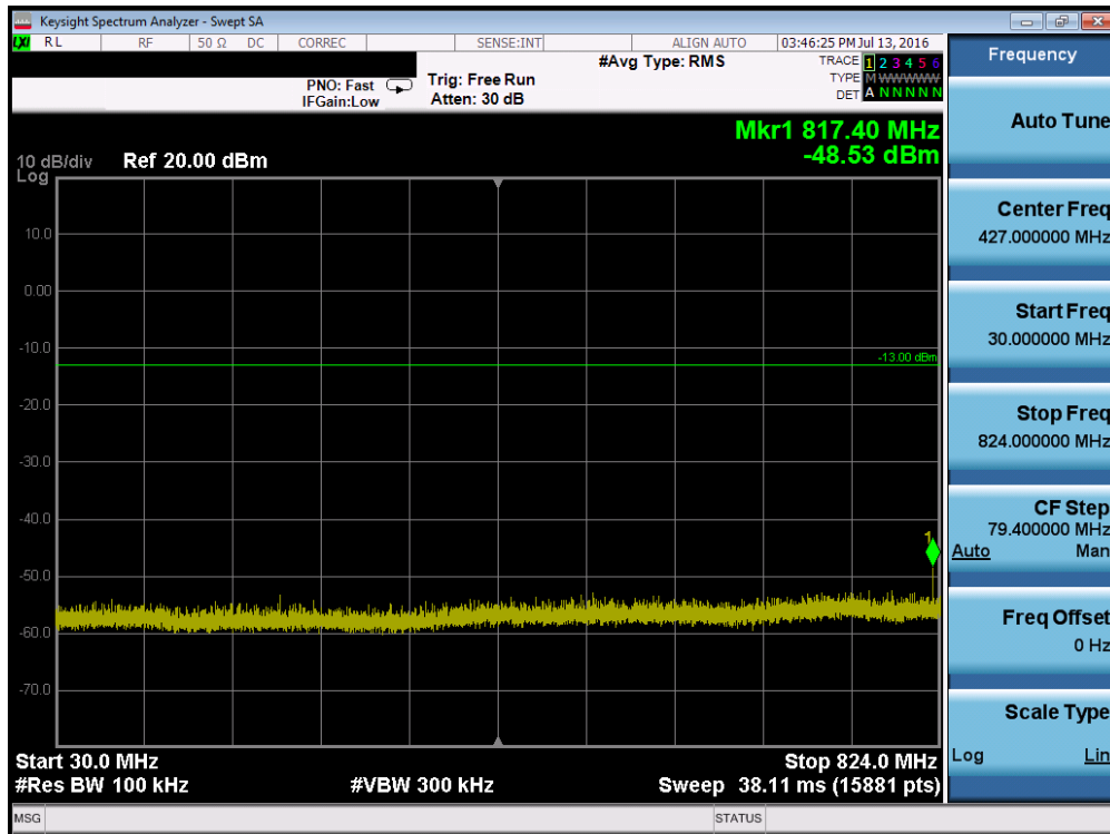
Plot 7-9. Conducted Spurious Plot (Cellular GPRS Mode – Ch. 190)
