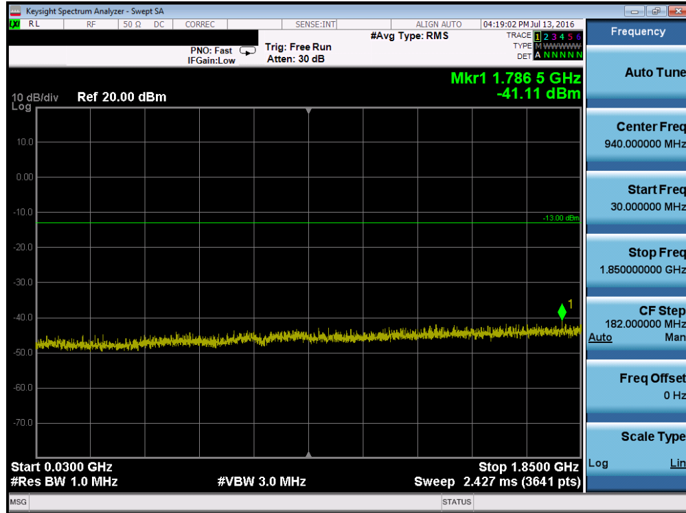
Plot 7-18. Conducted Spurious Plot (PCS GPRS Mode – Ch. 661)
