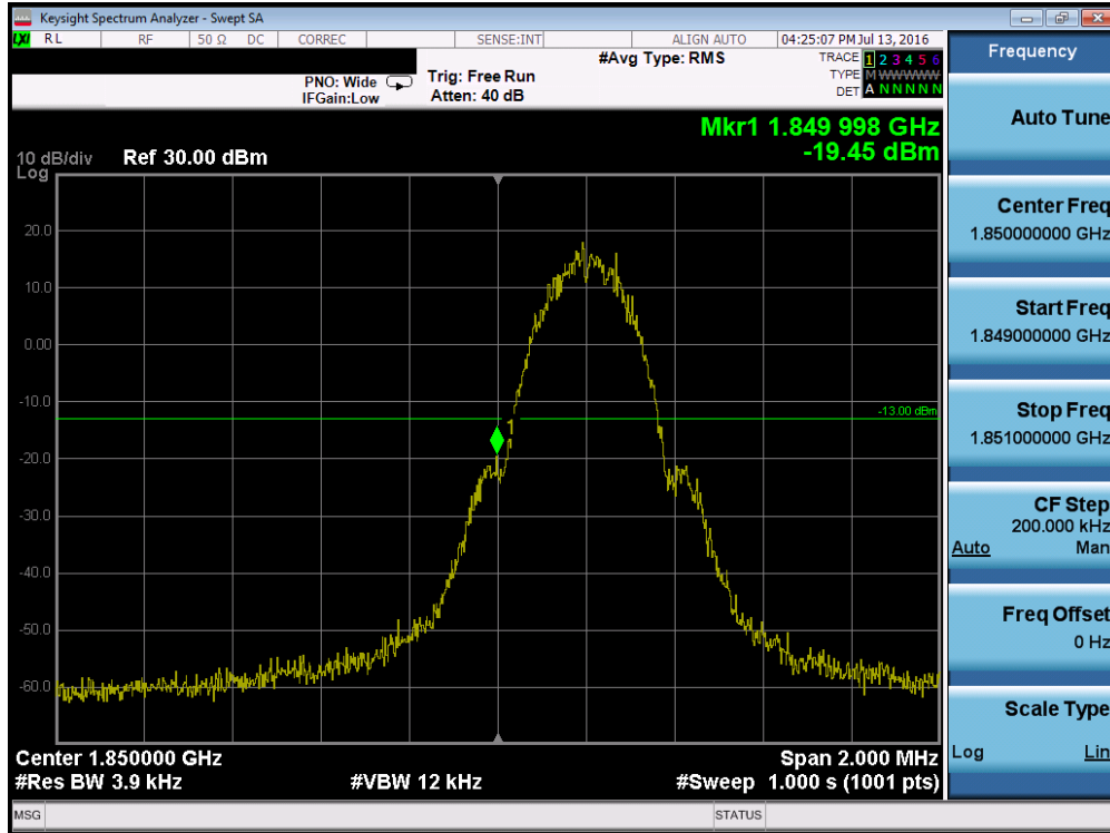
Plot 7-35. Band Edge Plot (PCS GPRS Mode – Ch. 512)
