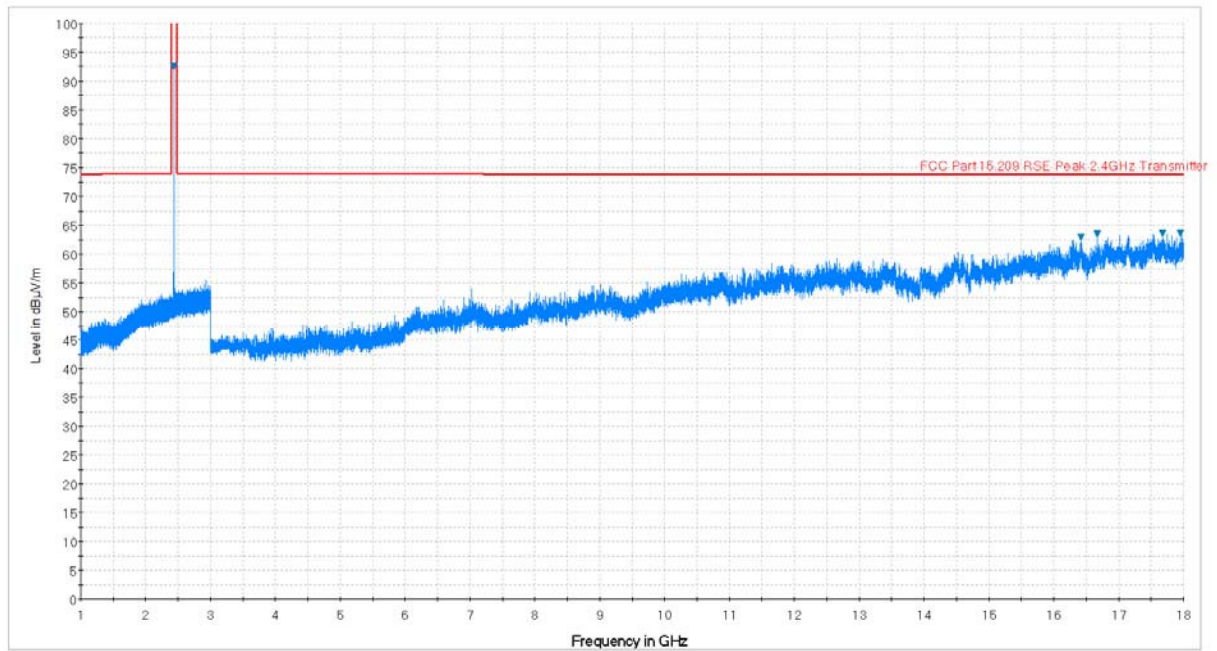
Plot 7-44. Radiated Spurious Plot above 1GHz (BT – Ch. 39, Ant. Pol. H)
