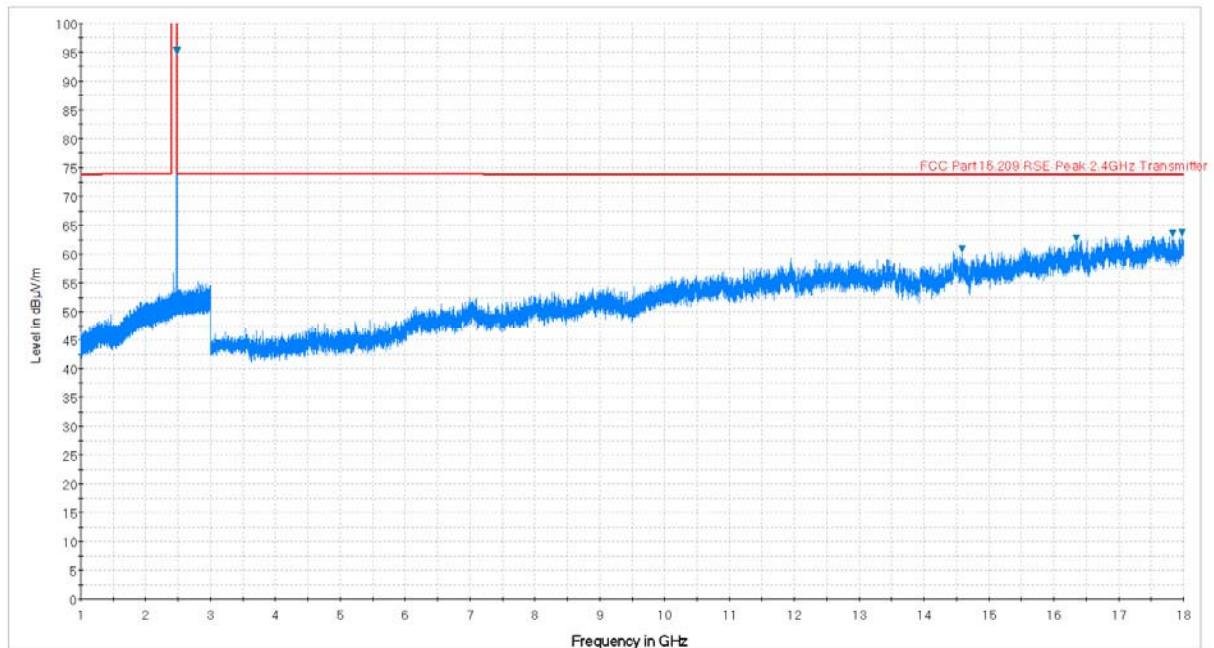
Plot 7-46. Radiated Spurious Plot above 1GHz (BT – Ch. 78, Ant. Pol. H)
