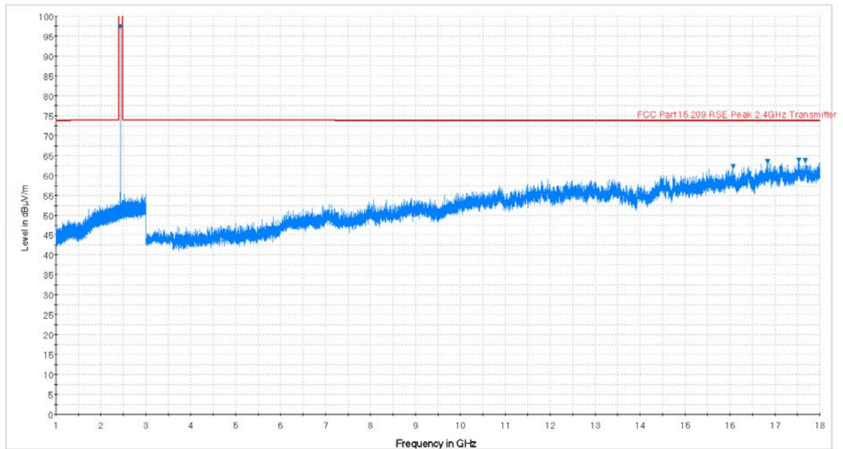
Plot 7-45. Radiated Spurious Plot above 1GHz (BT – Ch. 39, Ant. Pol. V)
