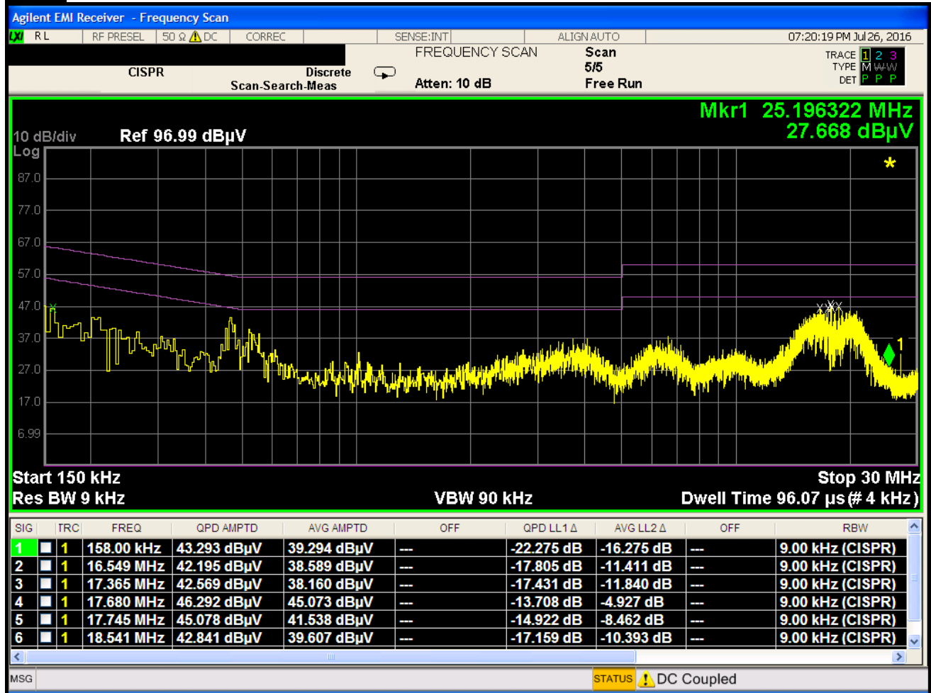
Plot 8-3. Line-Conducted Test Plot with 50 \Omega Termination (L1)
