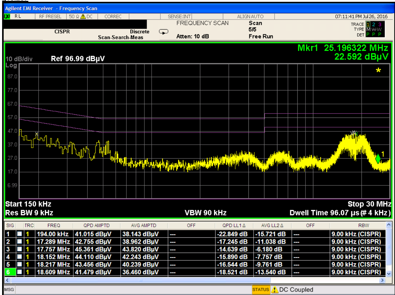
Plot 8-4. Line-Conducted Test Plot with 50 \Omega Termination (N)
