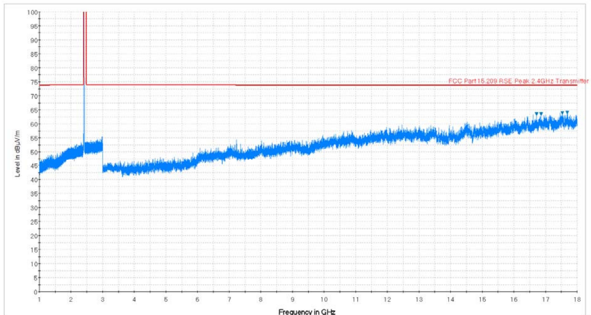
Plot 7-62. Radiated Spurious Plot above 1GHz (802.11b – Ch. 1, Ant. Pol. V)
