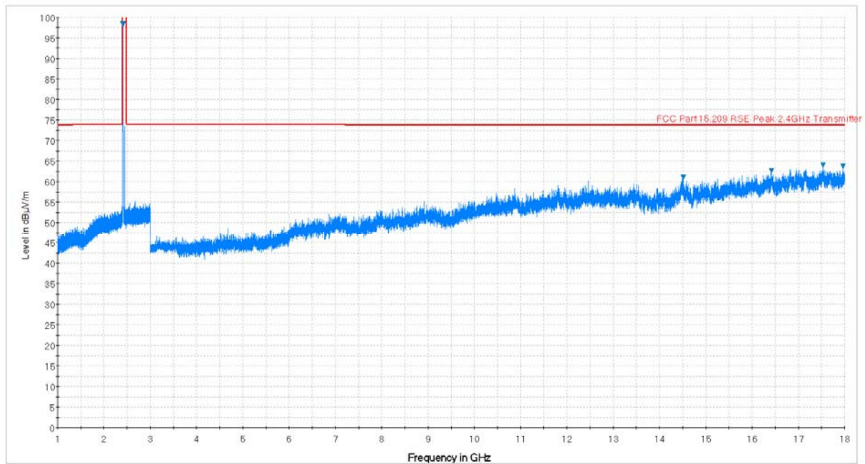
Plot 7-69. Radiated Spurious Plot above 1GHz (802.11b – Ch. 1, Ant. Pol. H)
