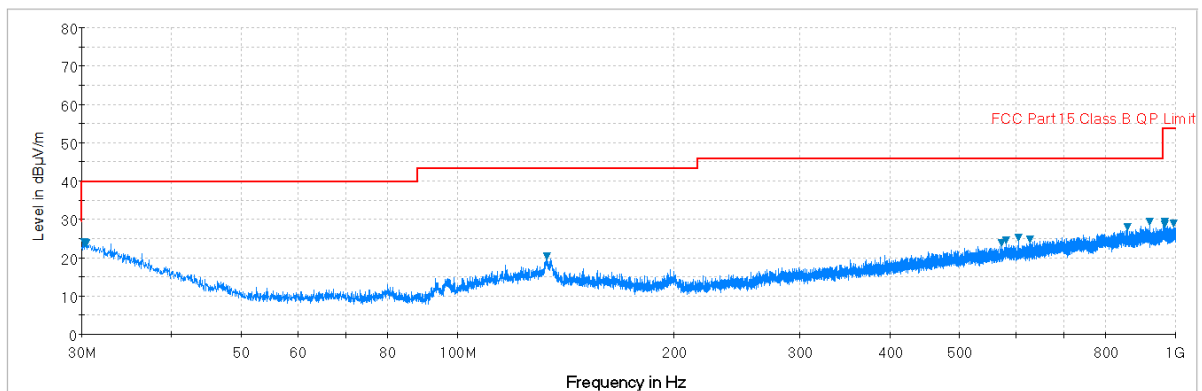
Plot 7-92. Radiated Spurious Plot below 1GHz (Pol. V)
