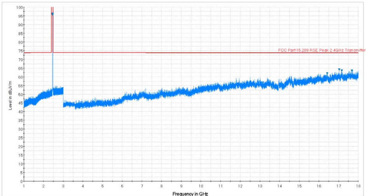
Plot 7-73. Radiated Spurious Plot above 1GHz (802.11b – Ch. 11, Ant. Pol. H)
