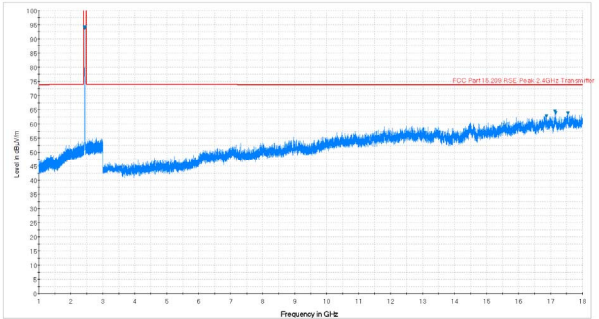
Plot 7-71. Radiated Spurious Plot above 1GHz (802.11b – Ch. 6, Ant. Pol. H)
