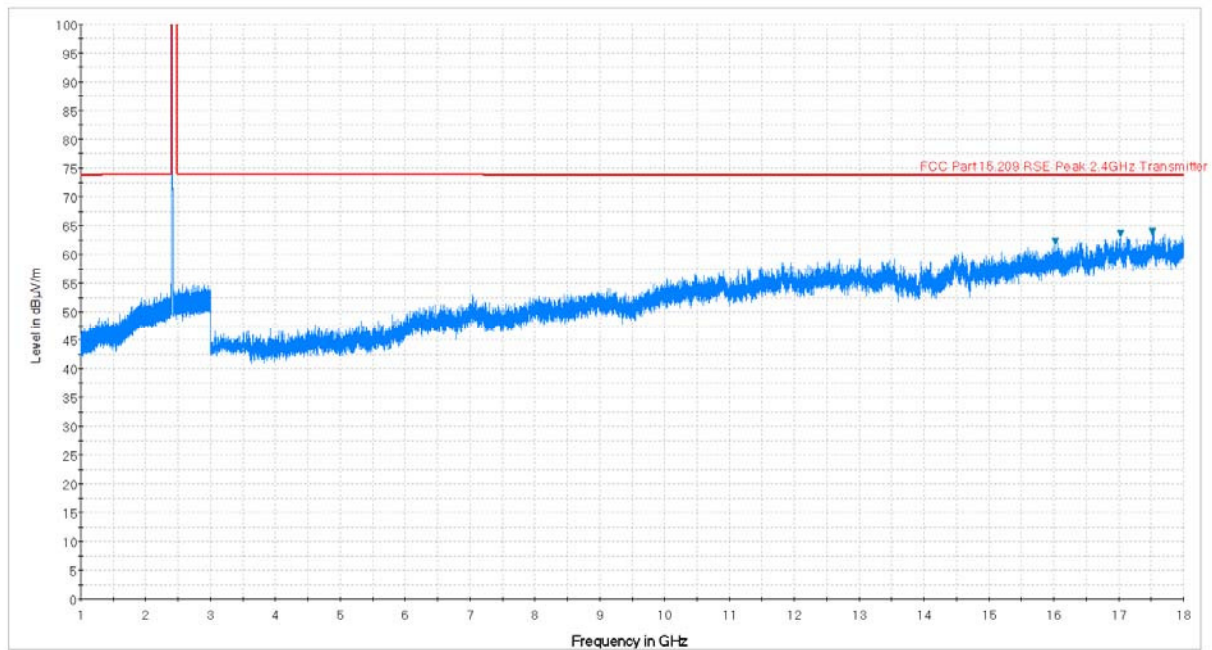
Plot 7-61. Radiated Spurious Plot above 1GHz (802.11b – Ch. 1, Ant. Pol. H)
