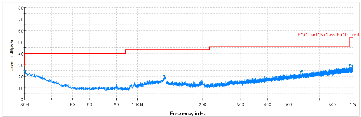
Plot 7-90. Radiated Spurious Plot below 1GHz (Pol. V)
