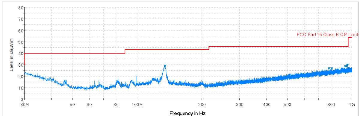
Plot 7-91. Radiated Spurious Plot below 1GHz (Pol. H)
