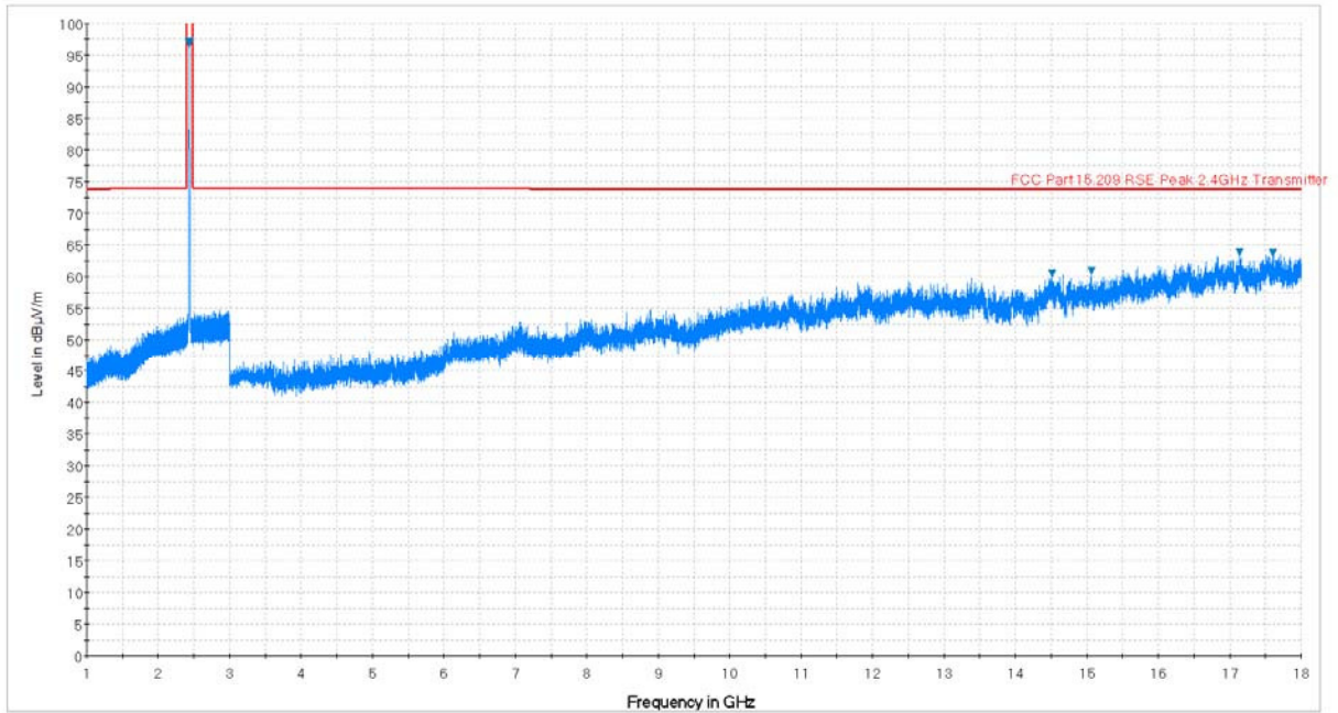
Plot 7-72. Radiated Spurious Plot above 1GHz (802.11b – Ch. 6, Ant. Pol. V)
