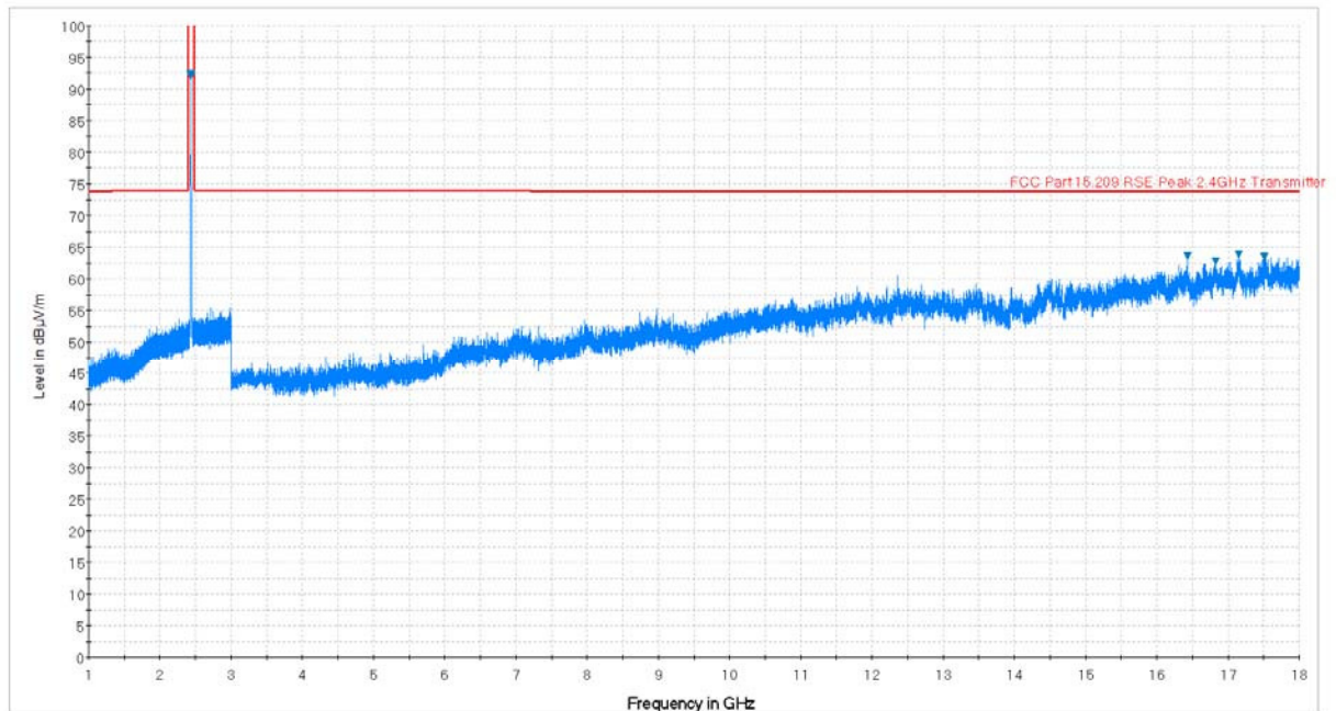
Plot 7-63. Radiated Spurious Plot above 1GHz (802.11b – Ch. 6, Ant. Pol. H)
