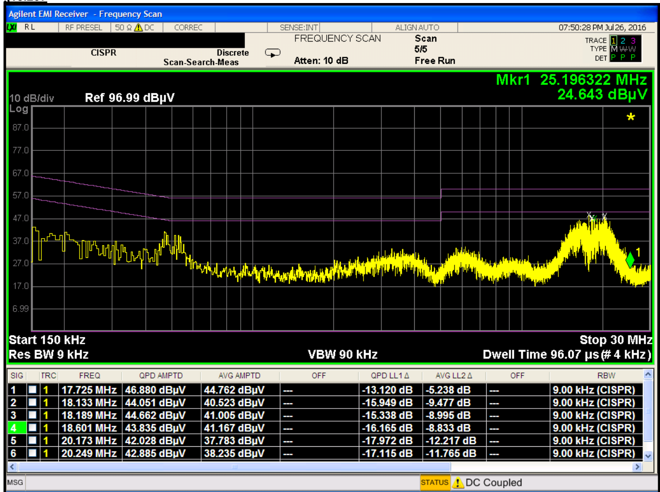
Plot 7-94. Line Conducted Plot with 802.11b (N)
