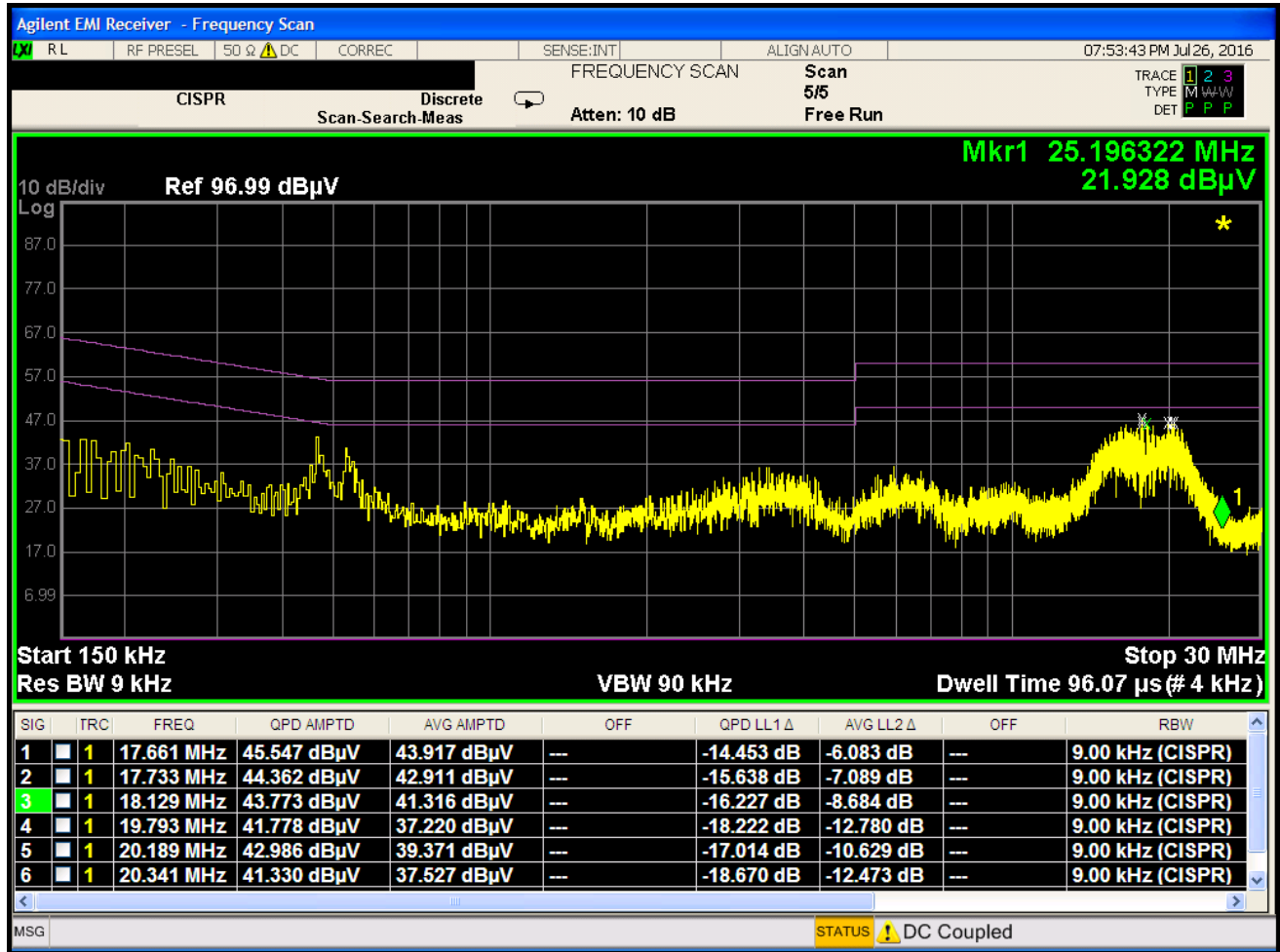
Plot 7-93. Line Conducted Plot with 802.11b (L1)
