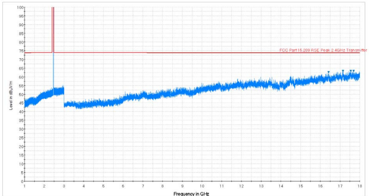
Plot 7-65. Radiated Spurious Plot above 1GHz (802.11b – Ch. 11, Ant. Pol. H)
