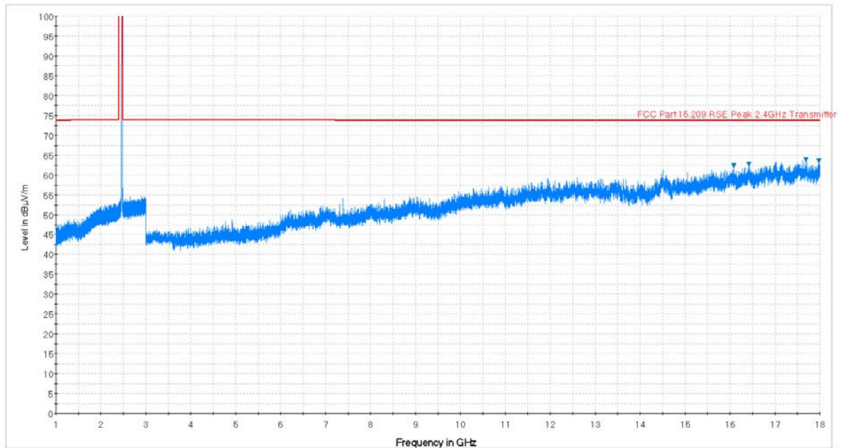
Plot 7-66. Radiated Spurious Plot above 1GHz (802.11b – Ch. 11, Ant. Pol. V)
