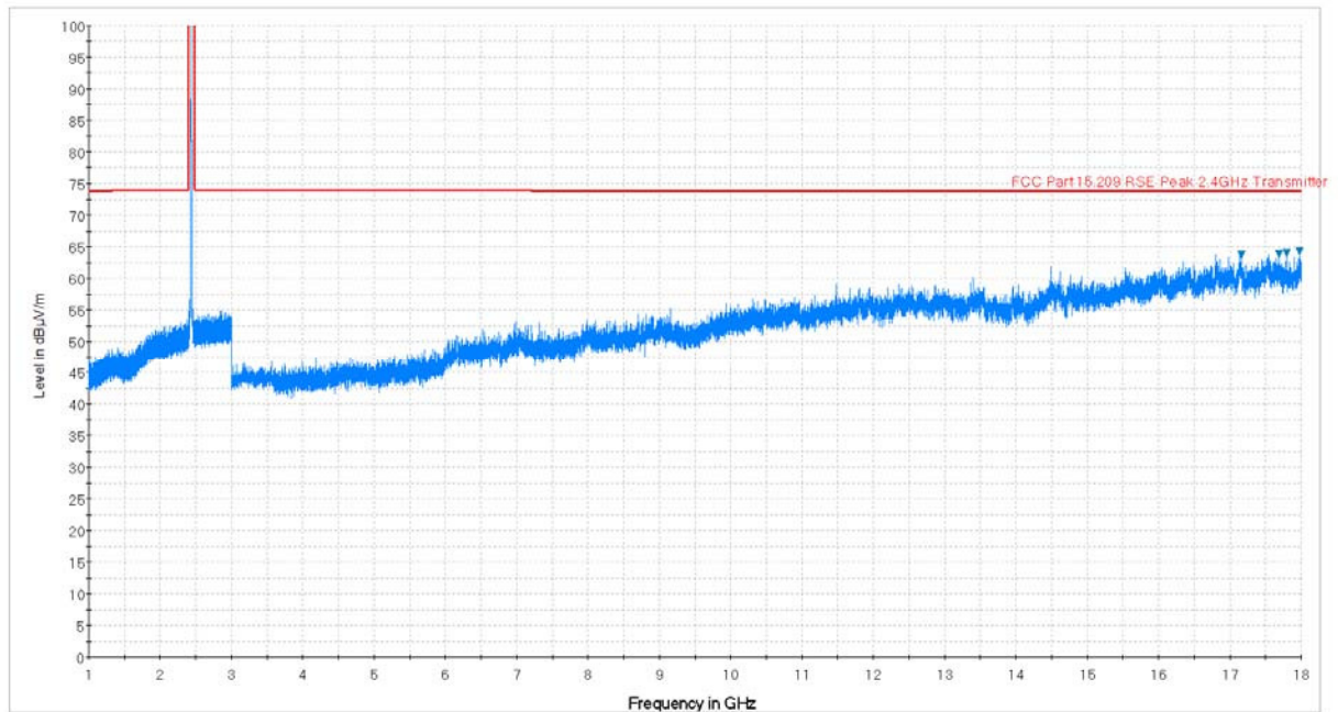
Plot 7-64. Radiated Spurious Plot above 1GHz (802.11b – Ch. 6, Ant. Pol. V)
