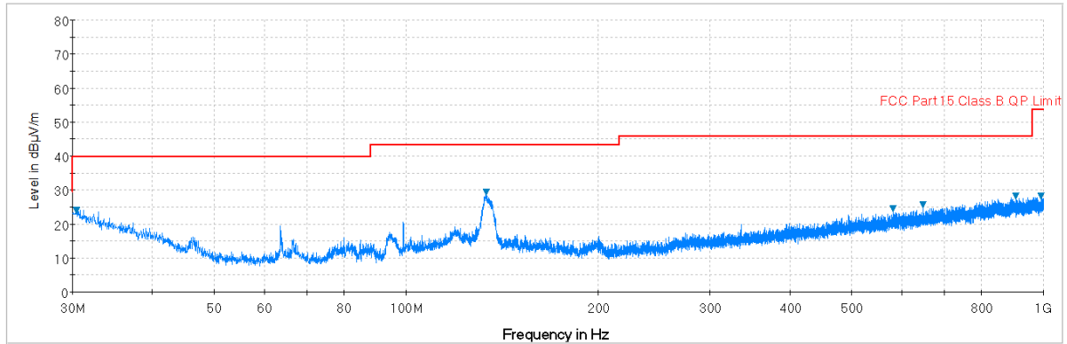
Plot 7-89. Radiated Spurious Plot below 1GHz (Pol. H)
