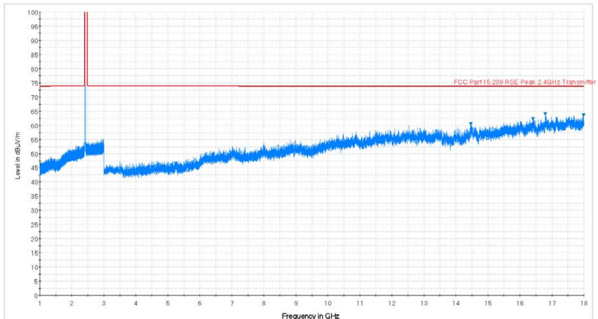
Plot 7-70. Radiated Spurious Plot above 1GHz (802.11b – Ch. 1, Ant. Pol. V)
