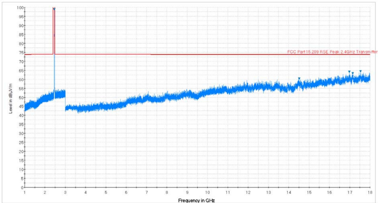
Plot 7-74. Radiated Spurious Plot above 1GHz (802.11b – Ch. 11, Ant. Pol. V)
