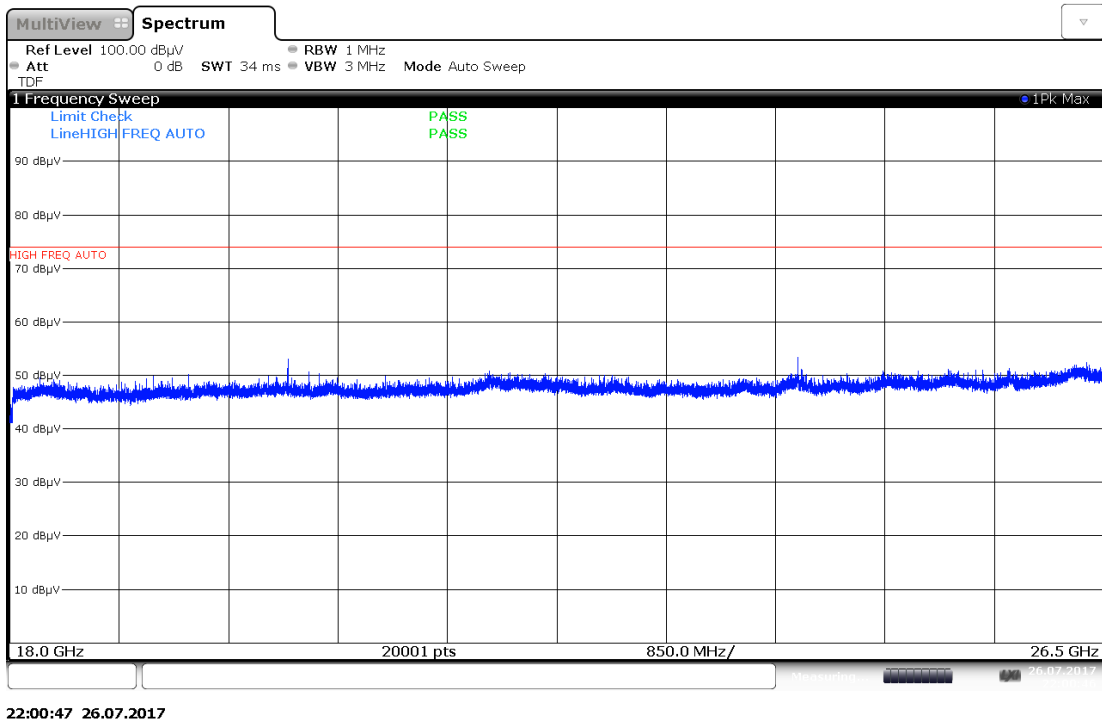
Plot 7-80. Radiated Spurious Plot above 18GHz (Pol. V)
