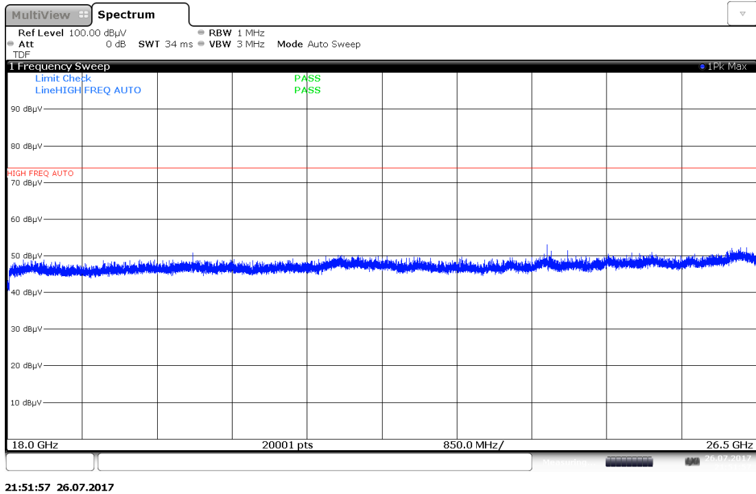
Plot 7-79. Radiated Spurious Plot above 18GHz (Pol. H)
