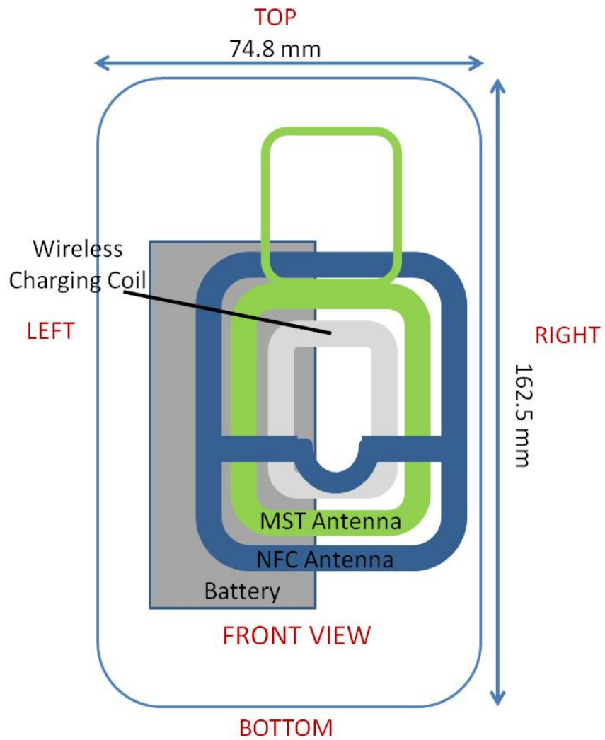
Figure F-2 NFC Antenna Locations
