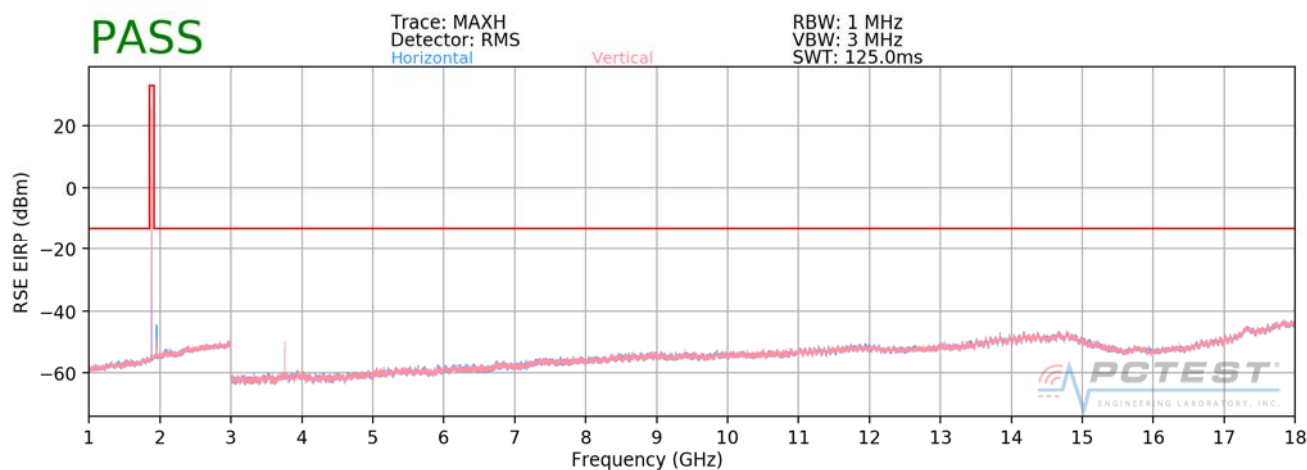
Plot 7-45. Radiated Spurious Data (GPRS Mode)
