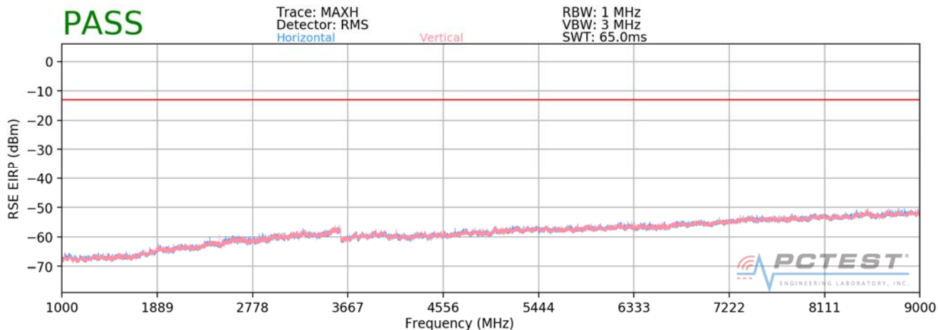
Plot 7-44. Radiated Spurious Data (Cellular GPRS Mode)
