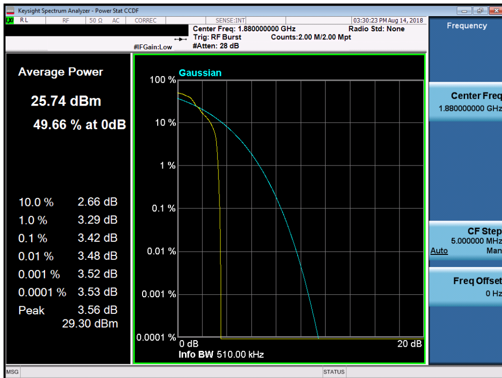
Plot 7-42. Peak-Average Ratio Plot (PCS EDGE Mode)
