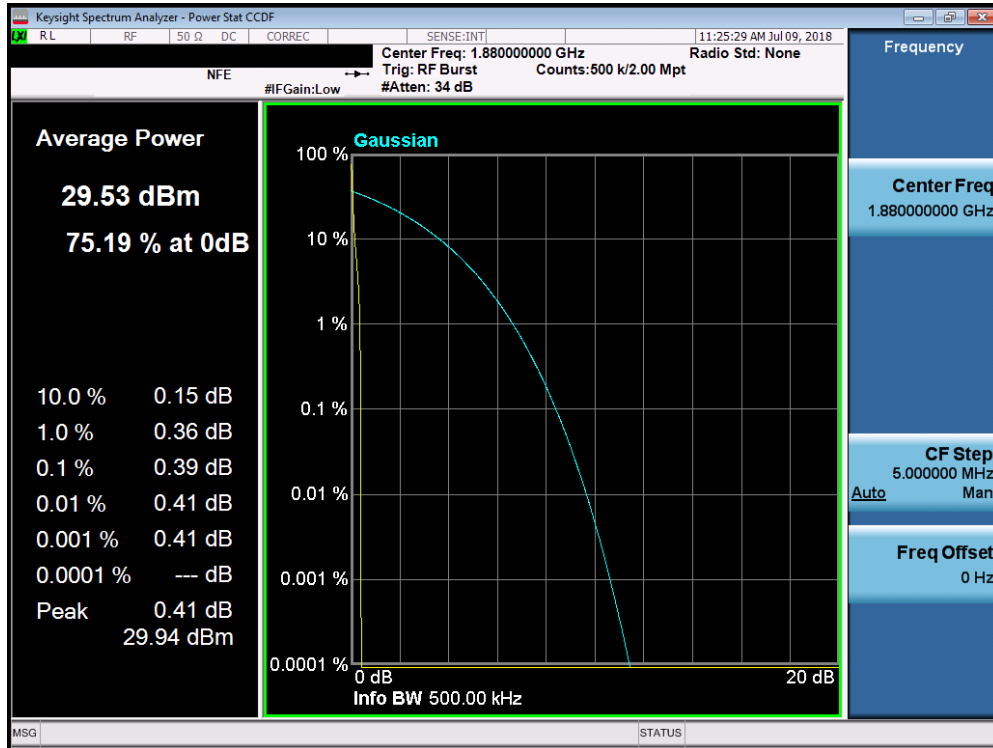
Plot 7-41. Peak-Average Ratio Plot (PCS GPRS Mode)
