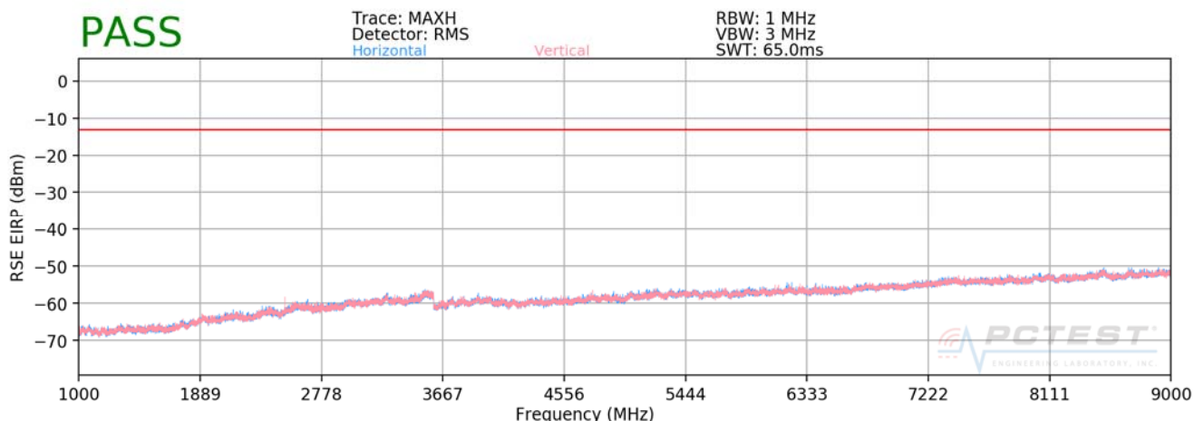
Plot 7-43. Radiated Spurious Data (Cellular GPRS Mode)
