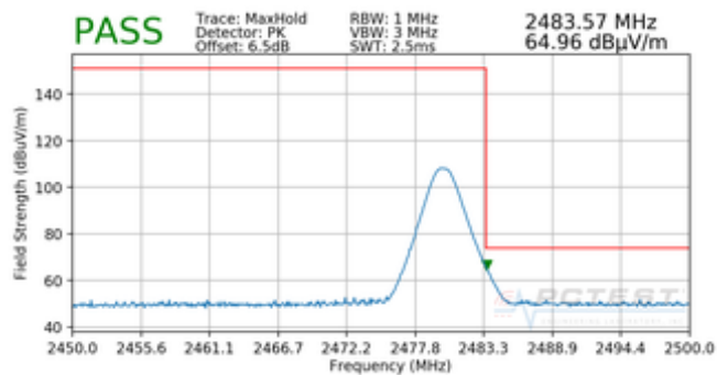
Plot 7-49. Radiated Restricted Upper Band Edge Measurement with WCP (Peak)
