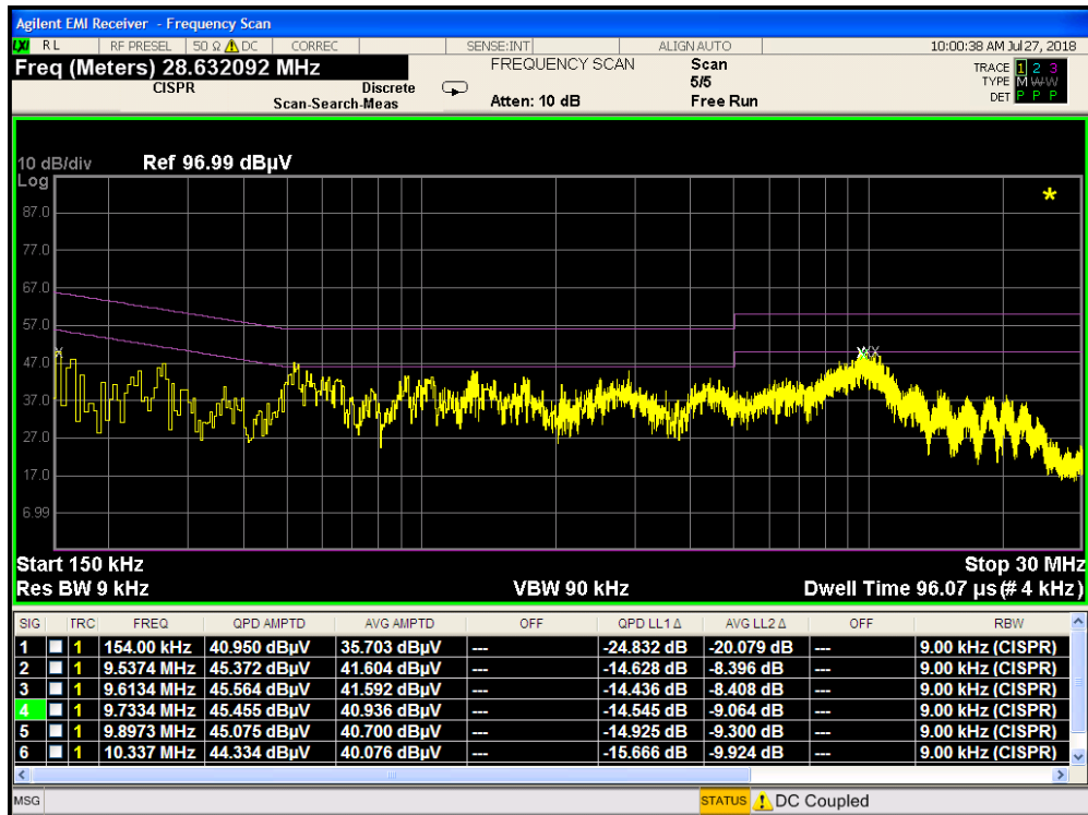
Plot 7-53. Line-Conducted Test Plot with WCP (L1)
