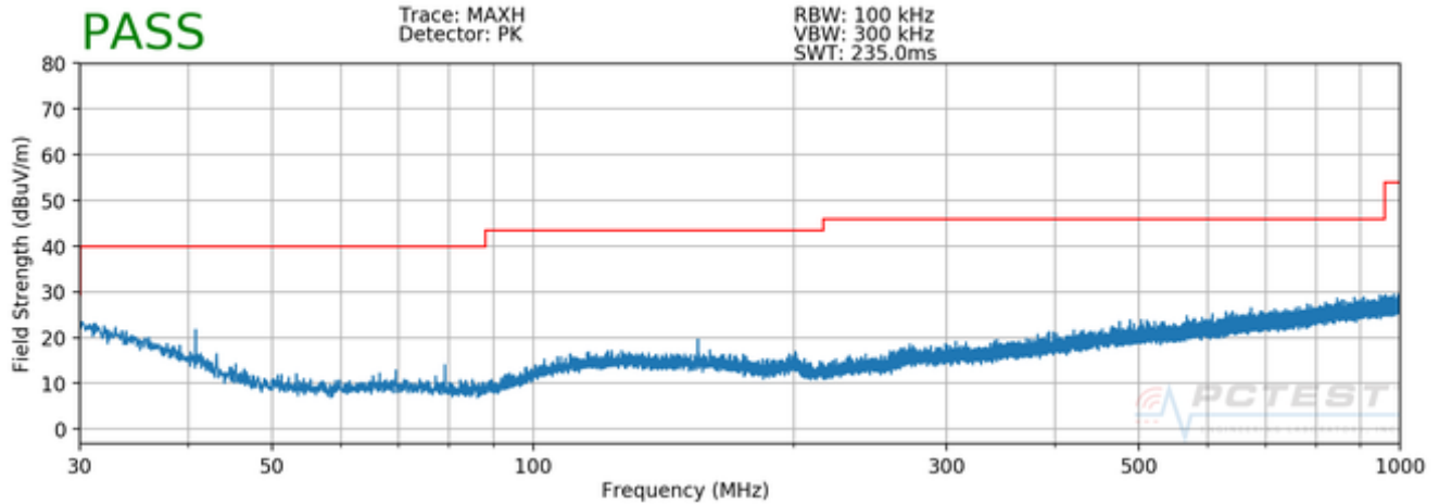
Plot 7-50. Radiated Spurious Plot below 1GHz
