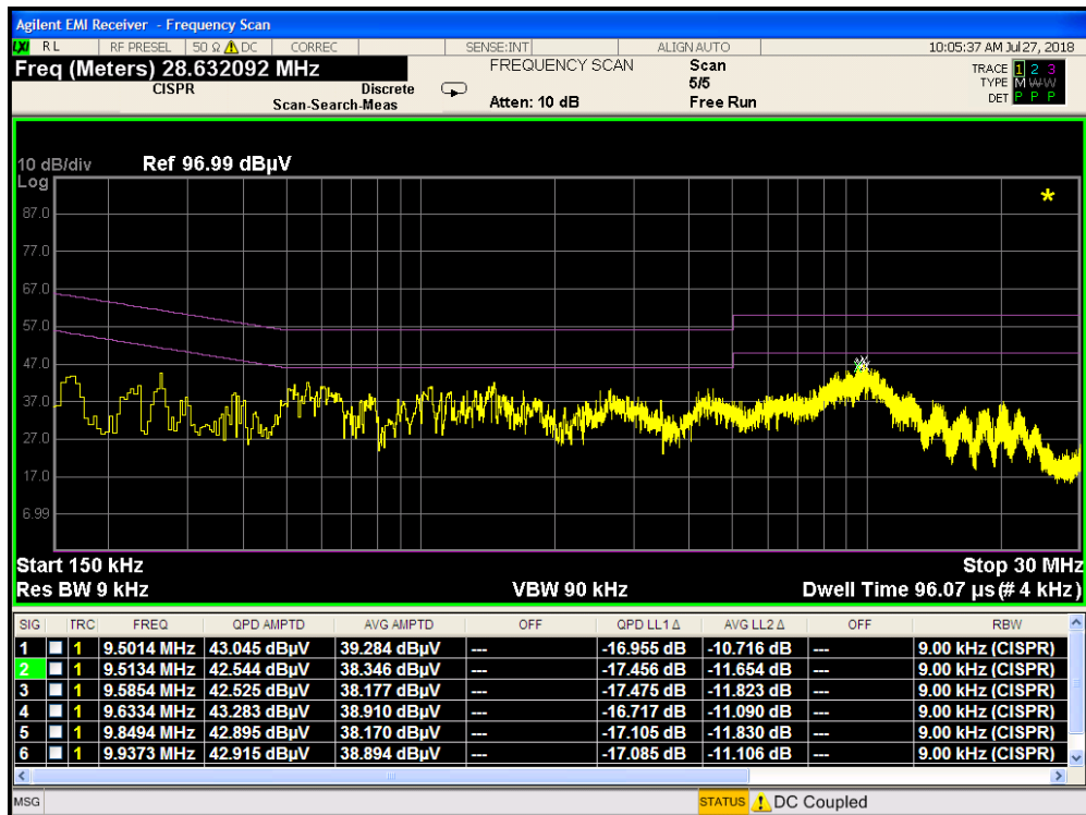
Plot 7-54. Line-Conducted Test Plot with WCP (N)
