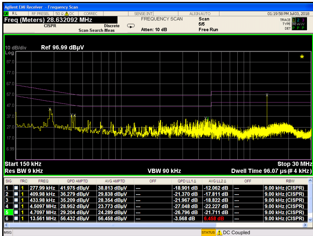
Plot 7-7. Line-Conducted Test Plot with Antenna Connected (N)
