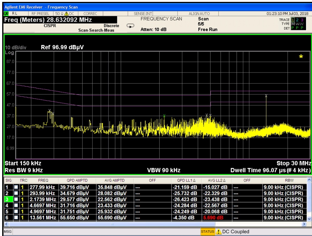
Plot 7-6. Line-Conducted Test Plot with Antenna Connected (L1)
