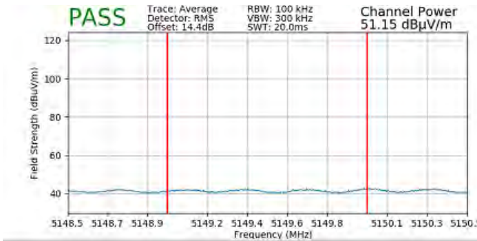
Plot 7-196. Radiated Lower Band Edge Plot SISO ANT1 (Average – UNII Band 1)
