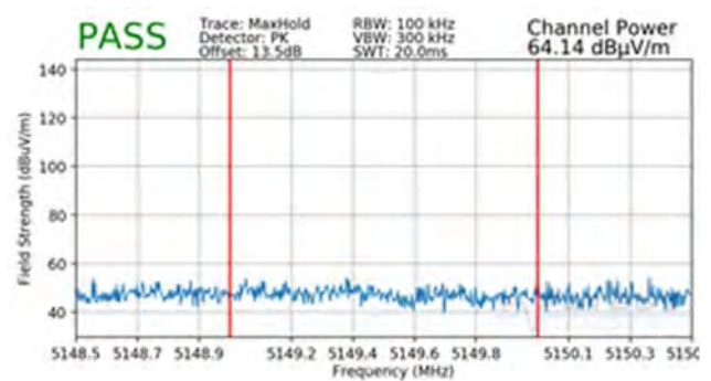
Plot 7-197. Radiated Lower Band Edge Plot SISO ANT1 (Peak – UNII Band 1)
