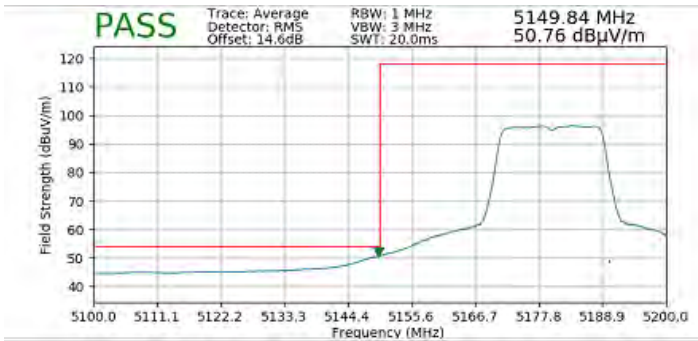
Plot 7-248. Radiated Band Edge Plot MIMO (Average – WCP)
