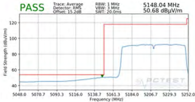
Plot 7-232. Radiated Lower Band Edge Plot SISO ANT2 (Average – UNII Band 1)
