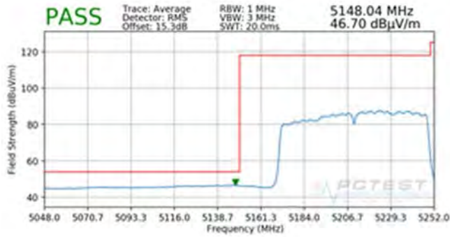
Plot 7-275. Radiated Band Edge Plot ANT (Average – WCP)
