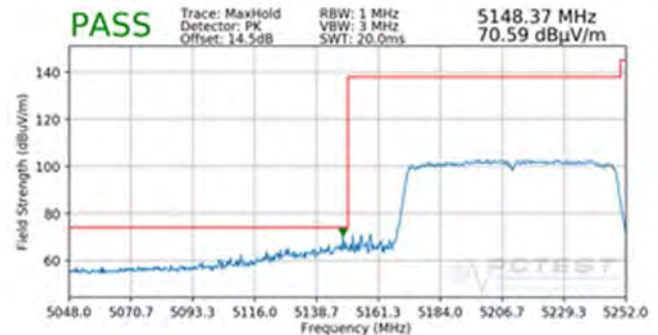
Plot 7-269. Radiated Lower Band Edge Plot MIMO (Peak – UNII Band 1)
