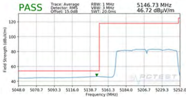
Plot 7-212. Radiated Band Edge Plot SISO ANT1 (Average – WCP)
