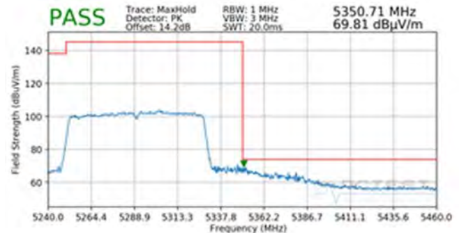
Plot 7-271. Radiated Upper Band Edge Plot MIMO (Peak – UNII Band 2A)
