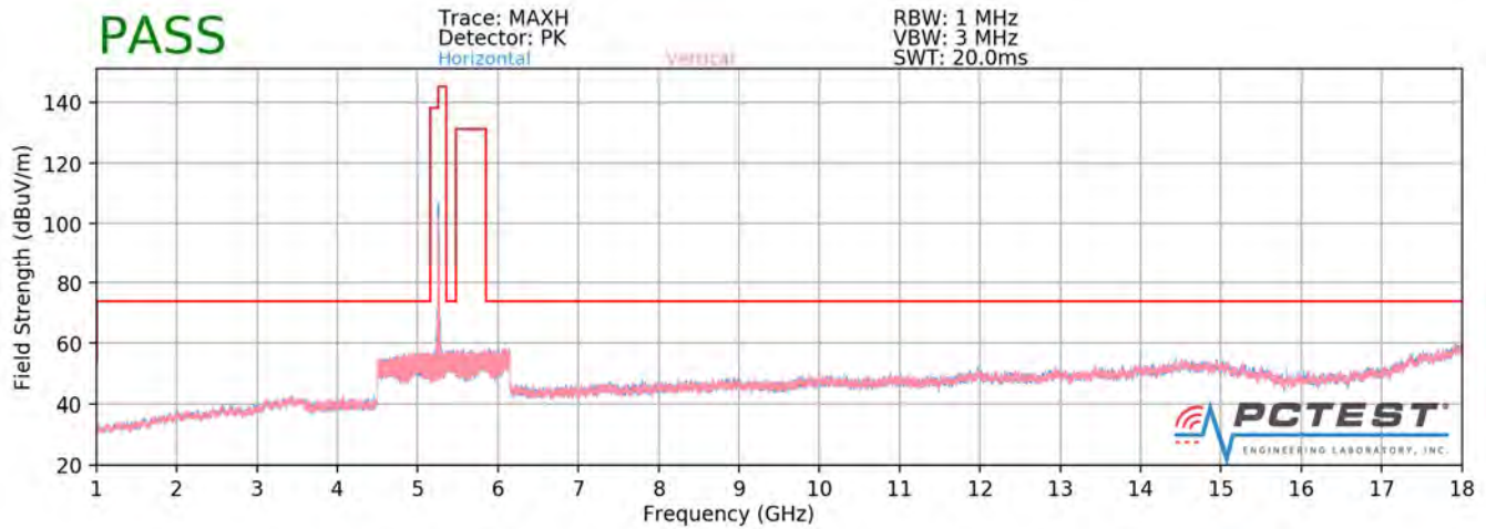
Plot 7-173. Radiated Spurious Plot above 1GHz SISO ANT2 (802.11a – U2A Ch. 56)
