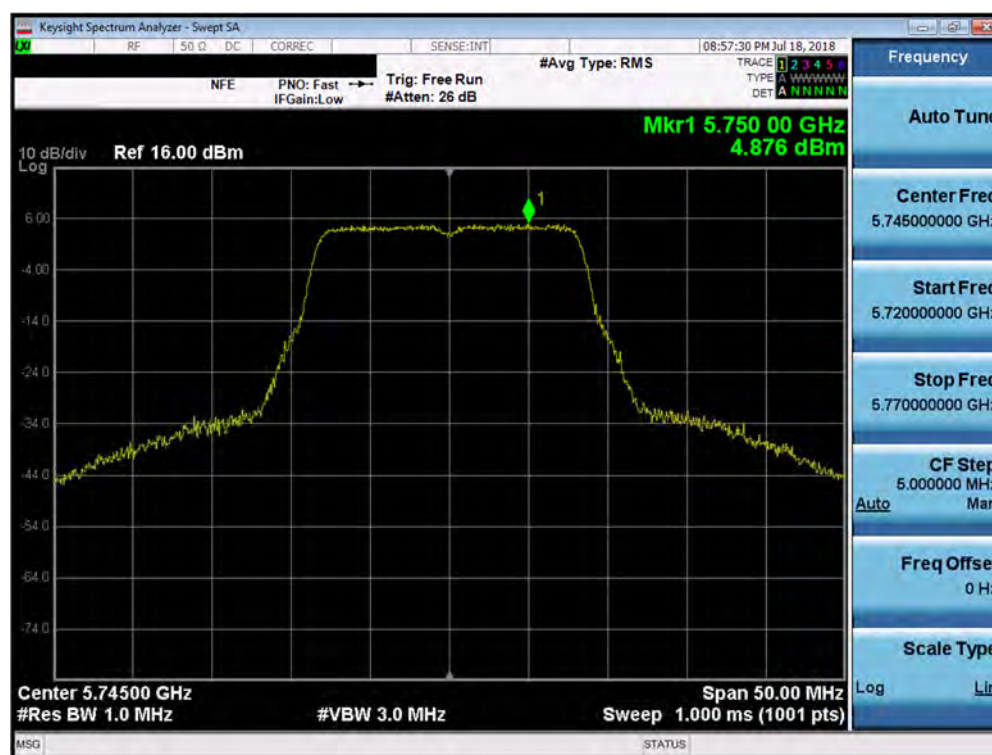
Plot 7-157. Power Spectral Density Plot SISO ANT2 (802.11a (UNII Band 3) – Ch. 149)
