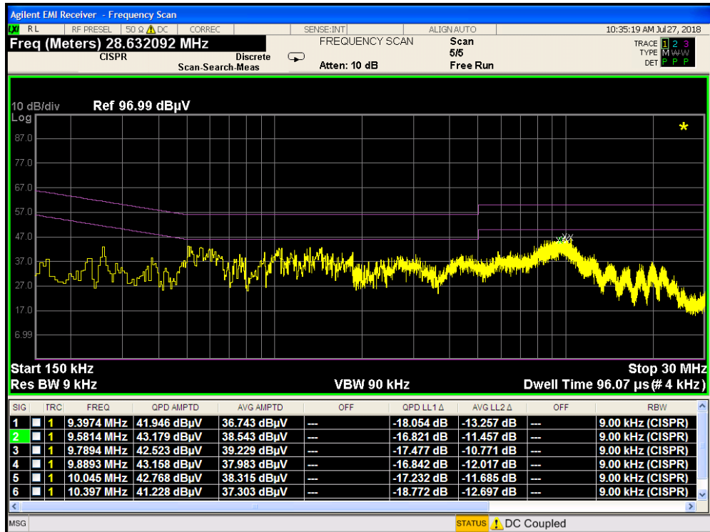
Plot 7-142. Line Conducted Plot with 802.11b with WCP (N)
