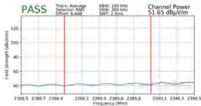
Plot 7-95. Radiated Restricted Lower Band Edge Measurement SISO ANT2 (Average)
