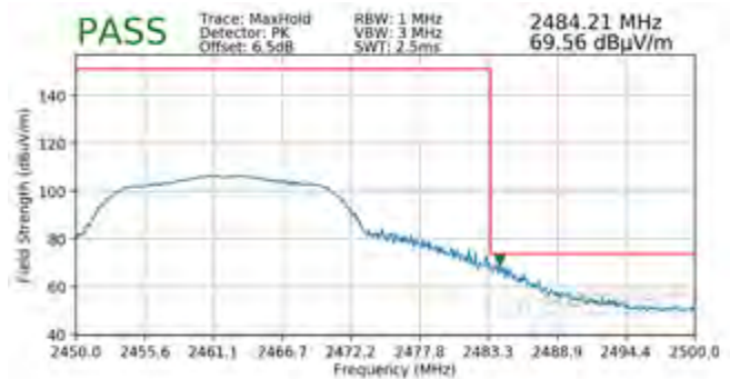
Plot 7-102. Radiated Restricted Upper Band Edge Measurement SISO ANT2 (Peak)
