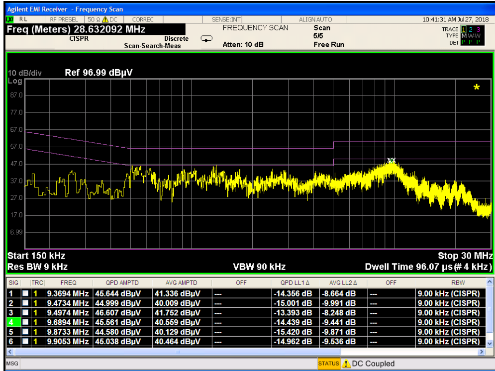
Plot 7-141. Line Conducted Plot with 802.11b with WCP (L1)
