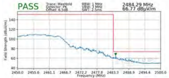
Plot 7-128. Radiated Restricted Upper Band Edge Measurement MIMO (Peak)
