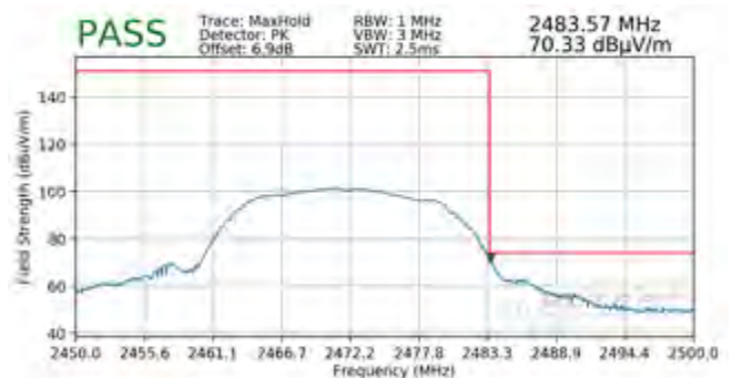
Plot 7-106. Radiated Restricted Upper Band Edge Measurement SISO ANT2 (Peak)
