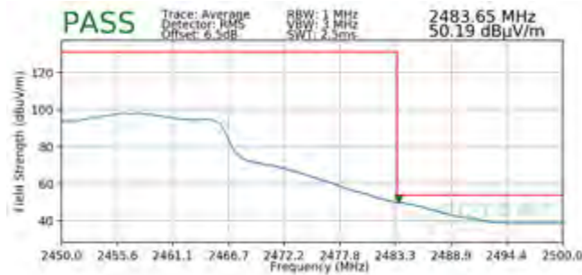
Plot 7-99. Radiated Restricted Upper Band Edge Measurement SISO ANT2 (Average)
