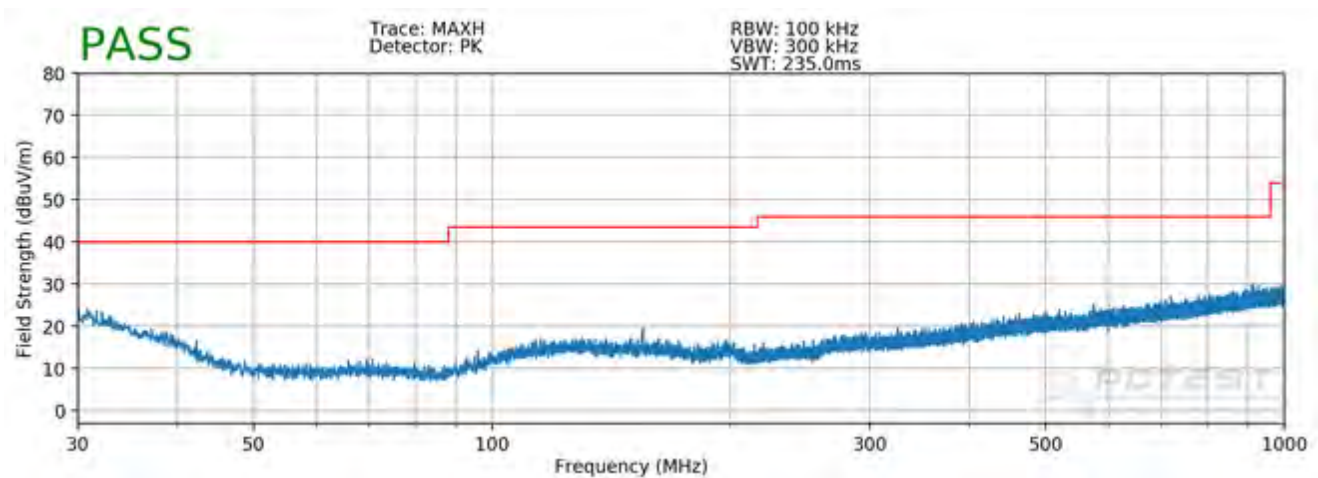
Plot 7-138. Radiated Spurious Plot below 1GHz SISO ANT2
