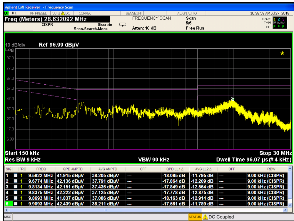
Plot 7-140. Line Conducted Plot with 802.11b (N)
