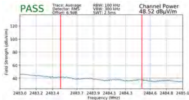
Plot 7-93. Radiated Restricted Band Edge Measurement SISO ANT1 with WCP (Average)
