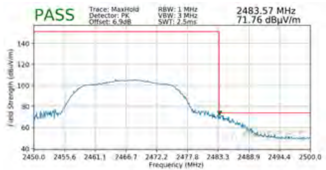
Plot 7-108. Radiated Restricted Band Edge Measurement SISO ANT2 with WCP (Peak)
