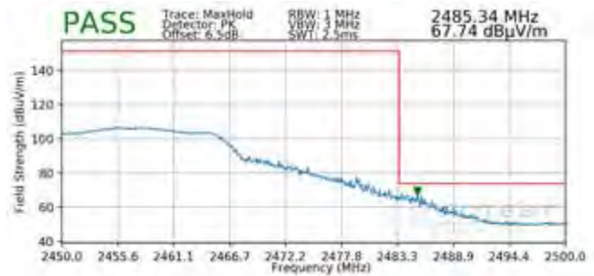
Plot 7-100. Radiated Restricted Upper Band Edge Measurement SISO ANT2 (Peak)
