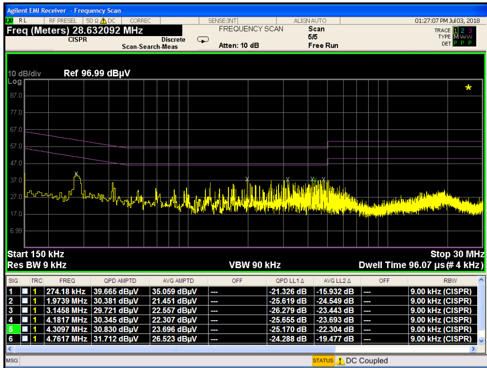
Plot 7-139. Line Conducted Plot with 802.11b (L1)
