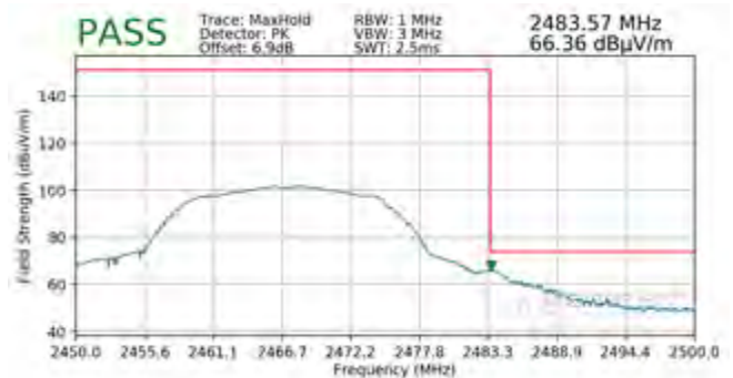
Plot 7-104. Radiated Restricted Upper Band Edge Measurement SISO ANT2 (Peak)
