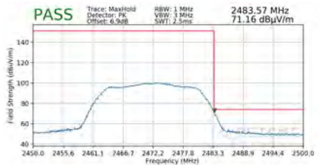
Plot 7-134. Radiated Restricted Upper Band Edge Measurement MIMO (Peak)
