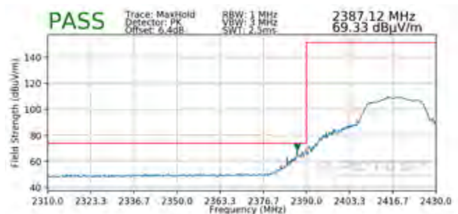
Plot 7-98. Radiated Restricted Lower Band Edge Measurement SISO ANT2 (Peak)
