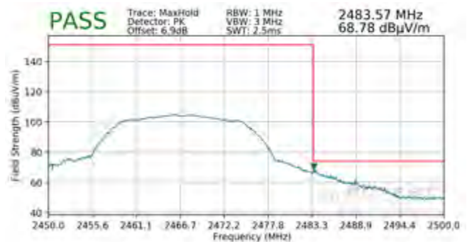
Plot 7-90. Radiated Restricted Upper Band Edge Measurement SISO ANT1 (Peak)
