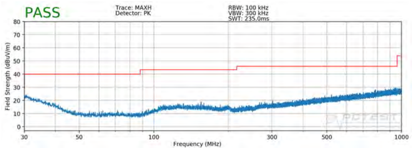
Plot 7-137. Radiated Spurious Plot below 1GHz SISO ANT1
