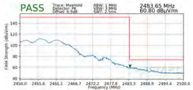
Plot 7-114. Radiated Restricted Upper Band Edge Measurement CDD (Peak)
