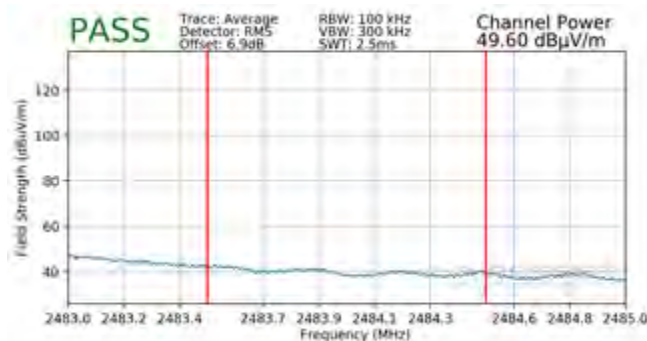
Plot 7-105. Radiated Restricted Upper Band Edge Measurement SISO ANT2 (Average)
