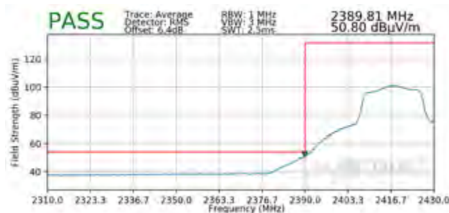
Plot 7-97. Radiated Restricted Lower Band Edge Measurement SISO ANT2 (Average)
