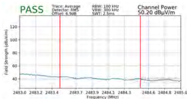
Plot 7-91. Radiated Restricted Upper Band Edge Measurement SISO ANT1 (Average)
