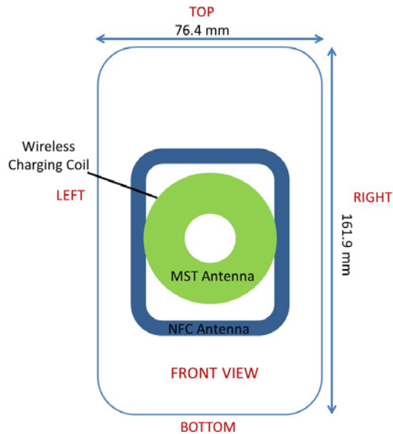
Figure F-2 NFC Antenna Locations
