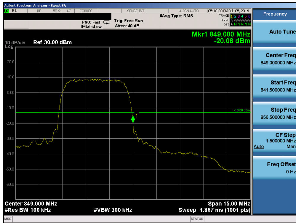
Plot 7-40. Band Edge Plot (Cellular WCDMA Mode – Ch. 4233)
