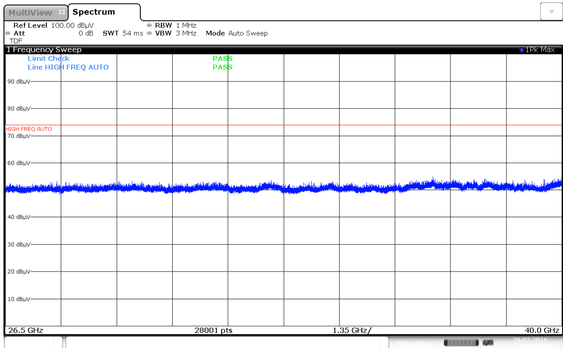
Plot 7-184. Radiated Spurious Plot above 26GHz (2.4 GHz – 5 GHz, Ant. Pol. V)
