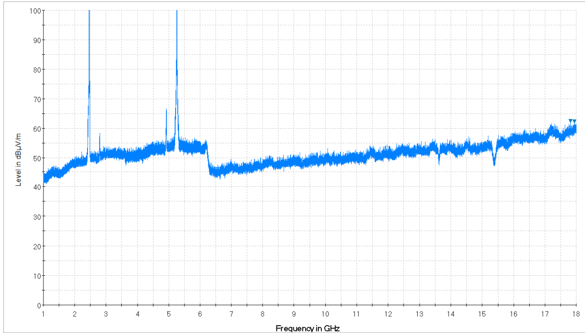
Plot 7-179. Radiated Spurious Plot above 1GHz (5GHz – 2.4 GHz, Ant. Pol. H)
