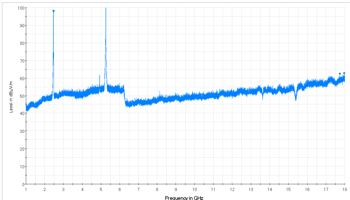
Plot 7-180. Radiated Spurious Plot above 1GHz (5GHz – 2.4 GHz, Ant. Pol. V)
