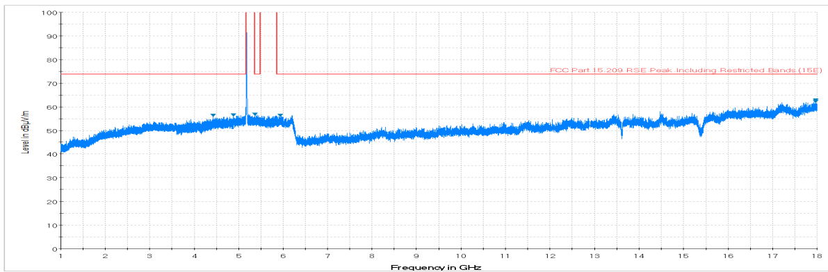
Plot 7-168. Radiated Spurious Plot above 1GHz (802.11a – U1 Ch. 40, Ant. Pol. V)
