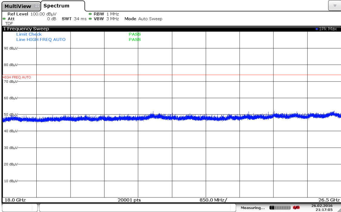
Plot 7-185. Radiated Spurious Plot 18GHz – 26GHz (5 GHz – 2.4 GHz, Ant. Pol. H)
