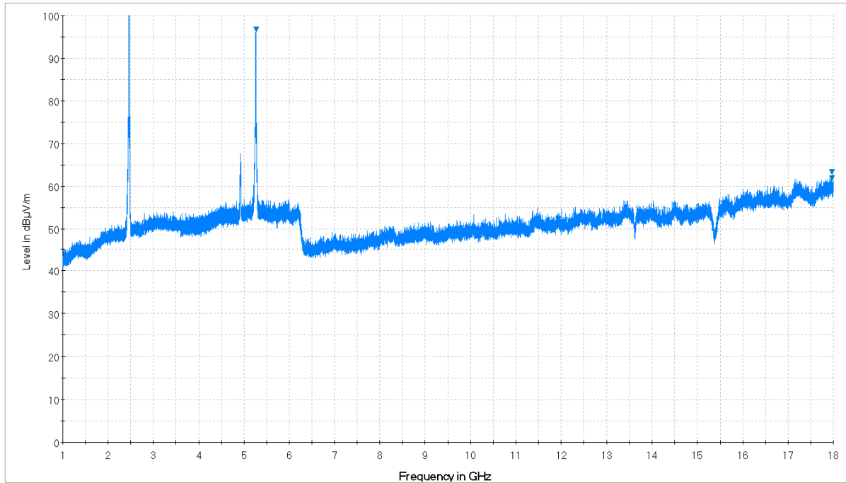
Plot 7-177. Radiated Spurious Plot above 1GHz (2.4GHz – 5GHz, Ant. Pol. H)
