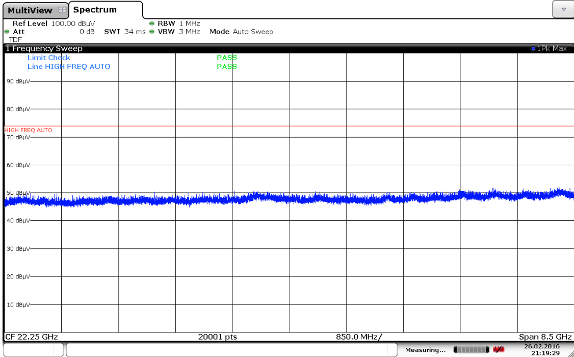
Plot 7-187. Radiated Spurious Plot 18GHz – 26GHz (5 GHz – 2.4 GHz, Ant. Pol. V)
