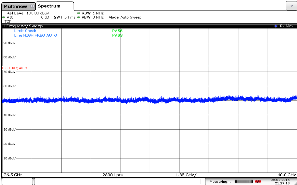
Plot 7-188. Radiated Spurious Plot above 26GHz (5 GHz – 2.4 GHz, Ant. Pol. V)
