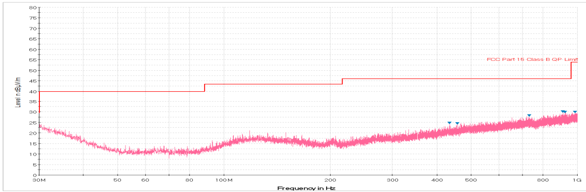
Plot 7-273. Radiated Spurious Plot below 1GHz (802.11a – U3 Ch. 157, Ant. Pol. V)
