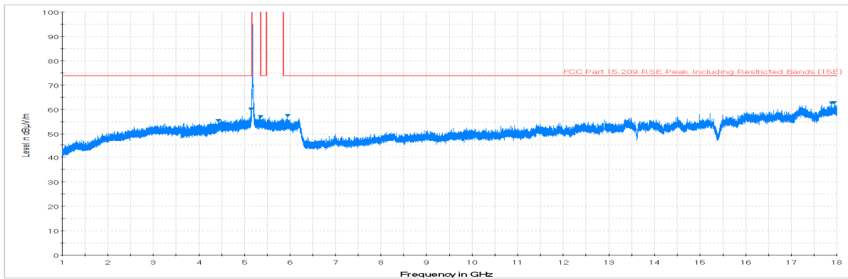
Plot 7-167. Radiated Spurious Plot above 1GHz (802.11a – U1 Ch. 40, Ant. Pol. H)
