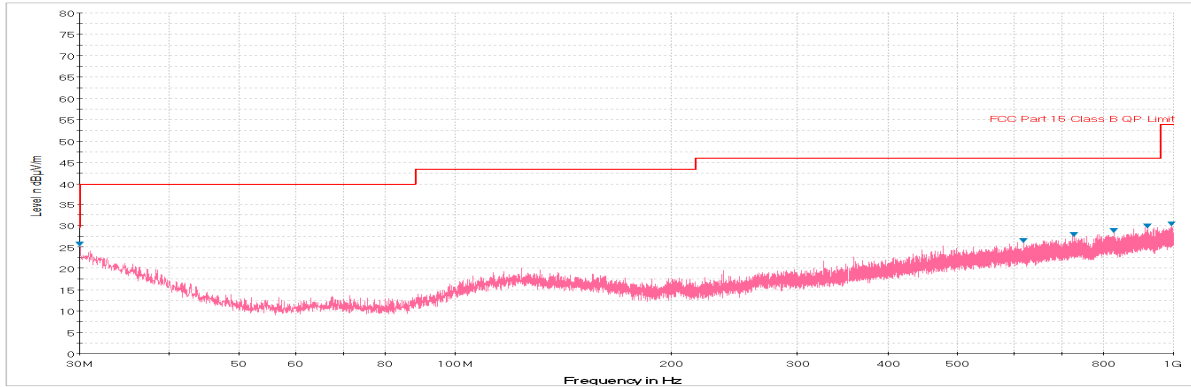
Plot 7-270. Radiated Spurious Plot below 1GHz (802.11a – U3 Ch. 157, Ant. Pol. H)
