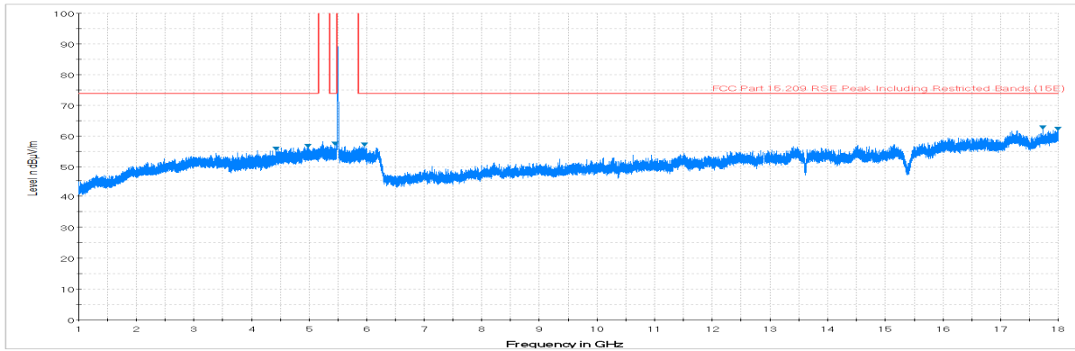
Plot 7-172. Radiated Spurious Plot above 1GHz (802.11a – U2C Ch. 116, Ant. Pol. V)
