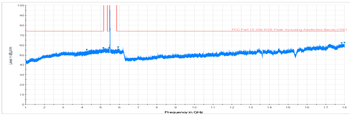
Plot 7-171. Radiated Spurious Plot above 1GHz (802.11a – U2C Ch. 116, Ant. Pol. H)
