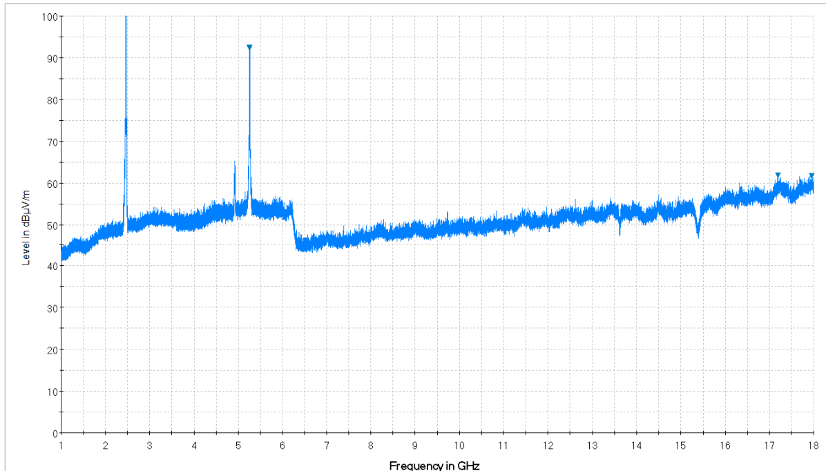
Plot 7-178. Radiated Spurious Plot above 1GHz (2.4GHz – 5GHz, Ant. Pol. V)
