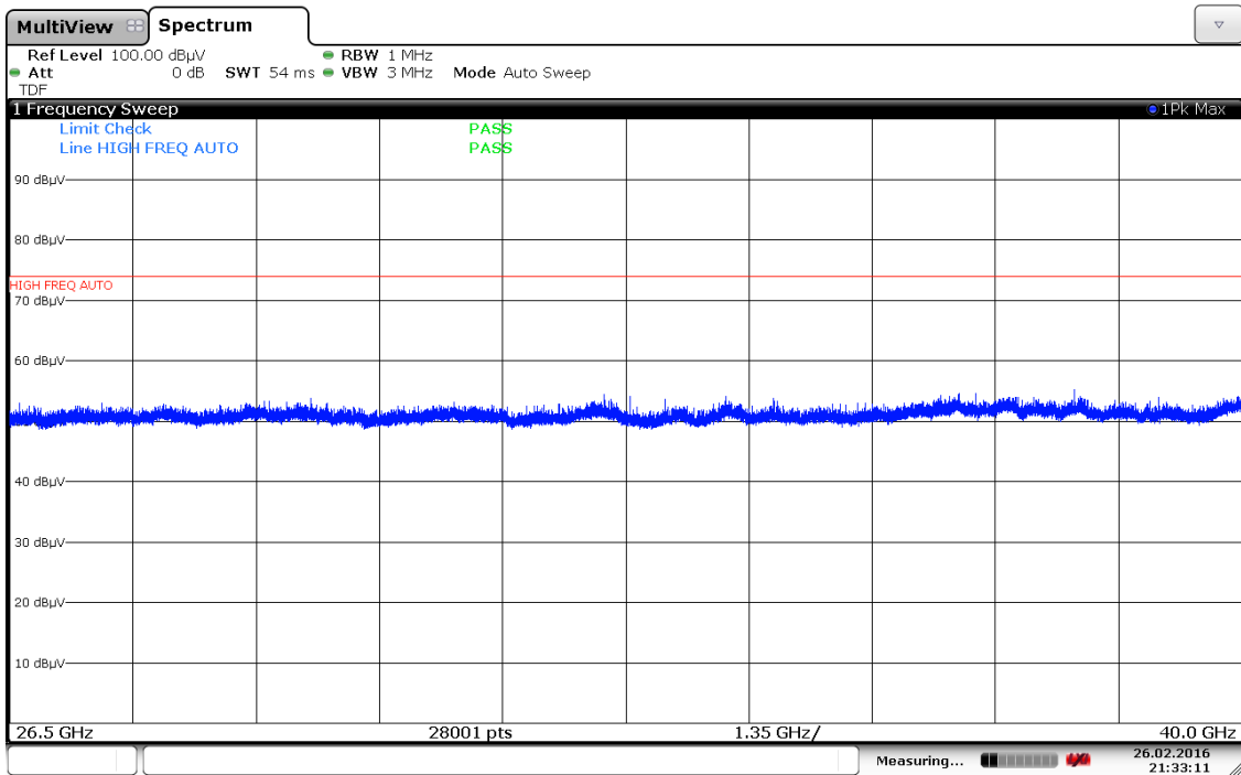
Plot 7-186. Radiated Spurious Plot above 26GHz (5 GHz – 2.4 GHz, Ant. Pol. H)
