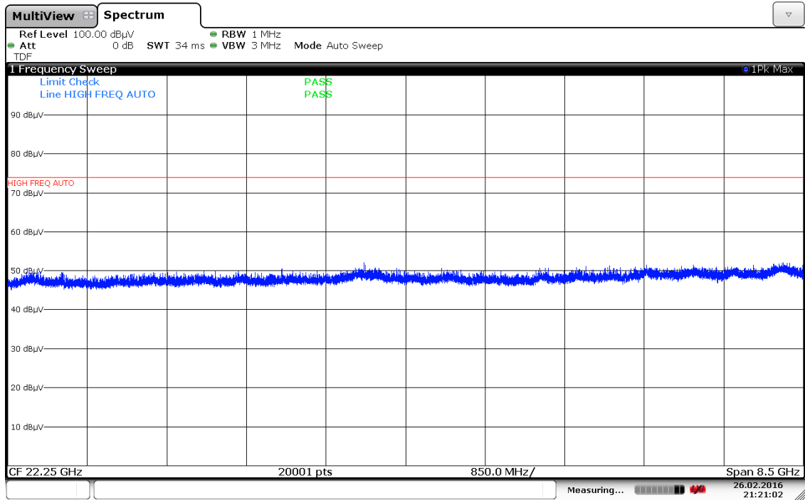
Plot 7-183. Radiated Spurious Plot 18GHz – 26GHz (2.4 GHz – 5 GHz, Ant. Pol. V)
