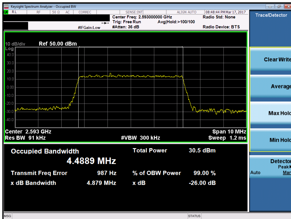
Plot 7-34. Occupied Bandwidth Plot (Band 41 – 5.0MHz 16-QAM – RB Size 25)
