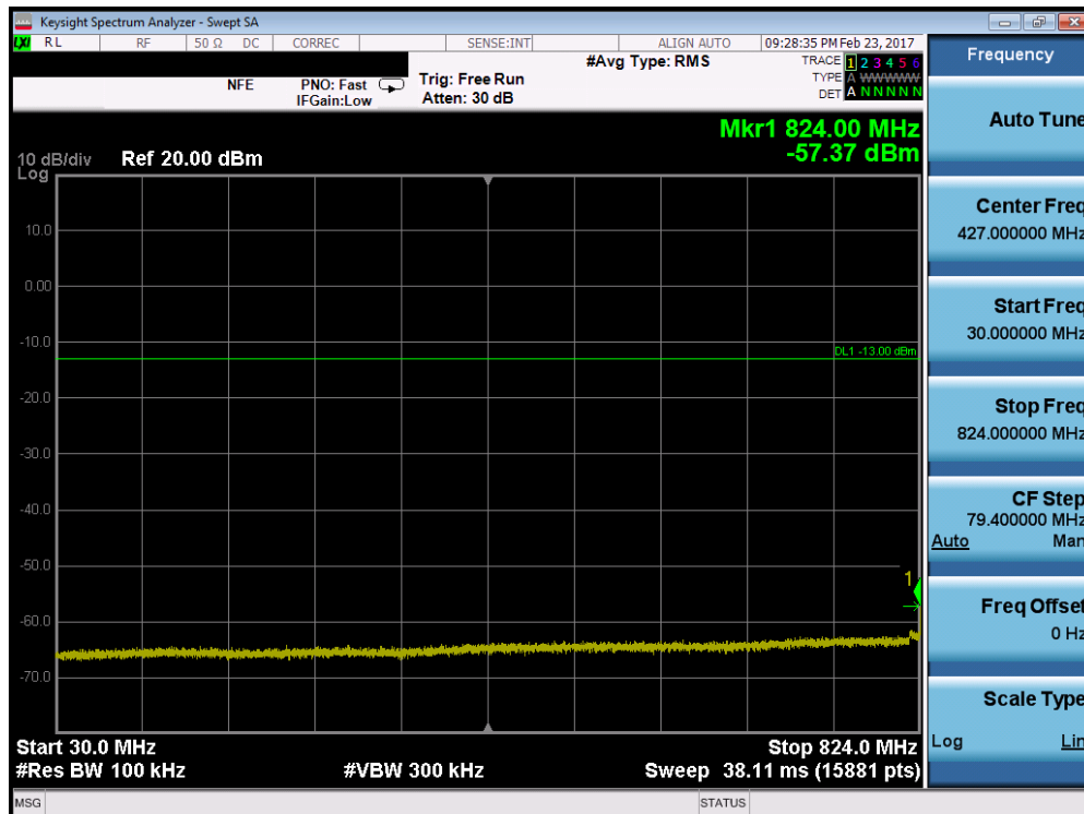
Plot 7-56. Conducted Spurious Plot (Band 5 – 5.0MHz QPSK – RB Size 1, RB Offset 0 – Mid Channel)
