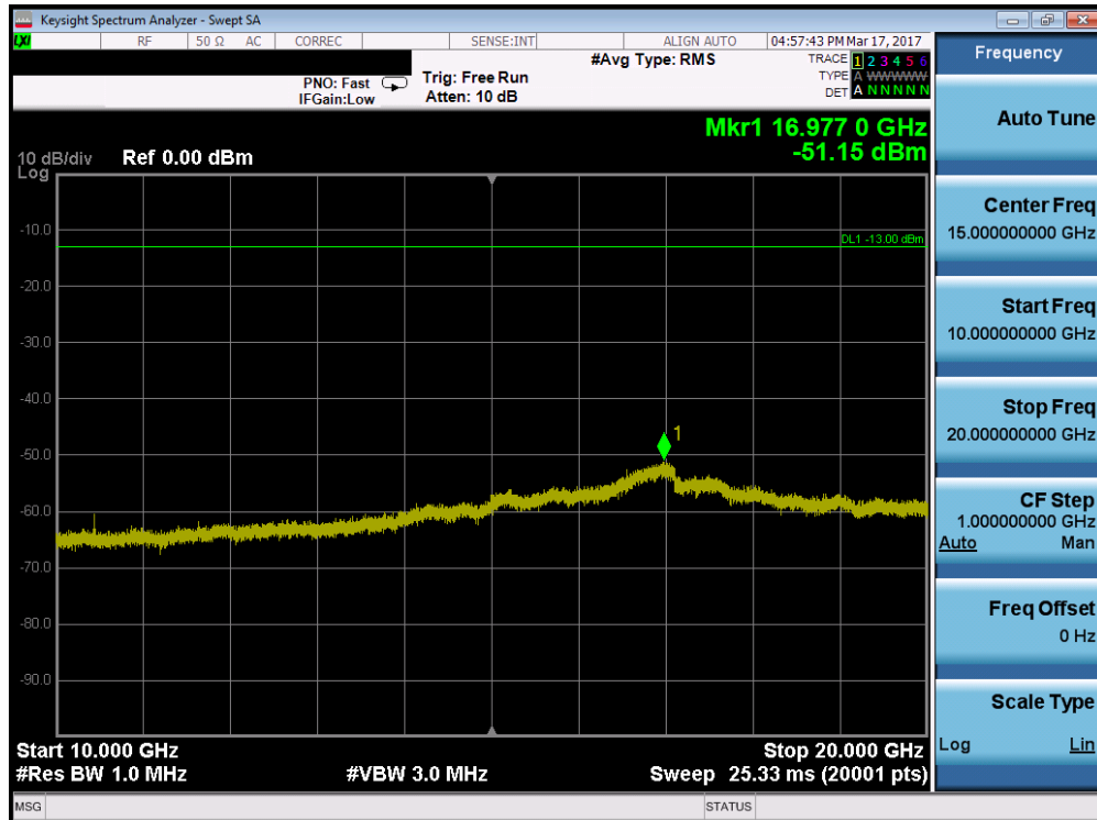
Plot 7-70. Conducted Spurious Plot (Band 4 – 15.0MHz QPSK – RB Size 1, RB Offset 0 – High Channel)
