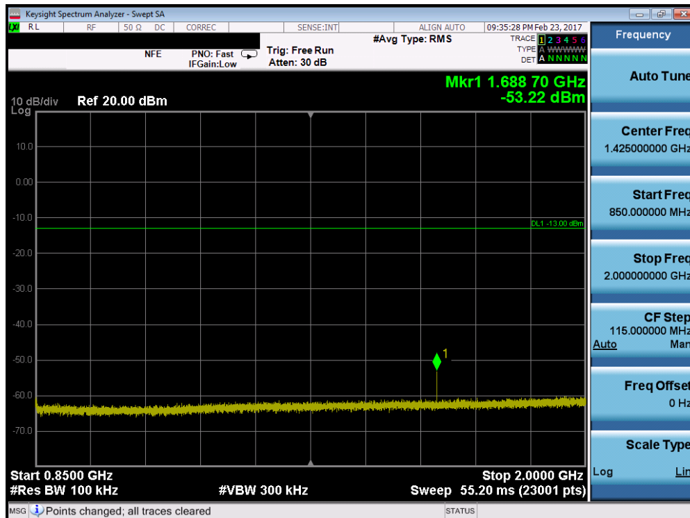
Plot 7-60. Conducted Spurious Plot (Band 5 – 5.0MHz QPSK – RB Size 1, RB Offset 0 – High Channel)
