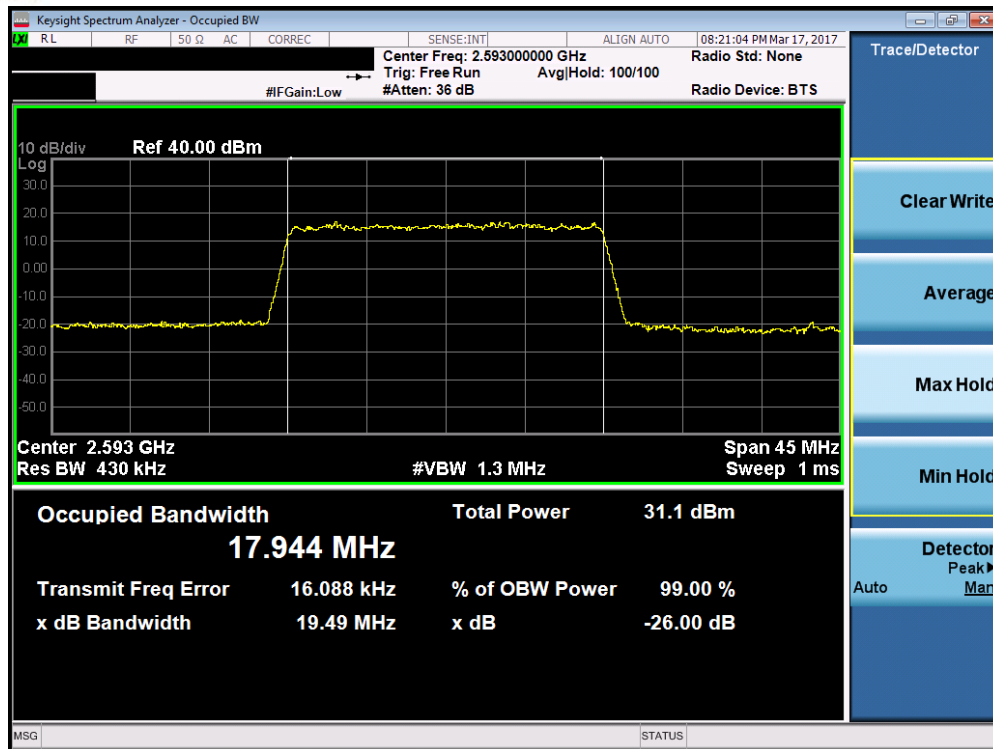
Plot 7-39. Occupied Bandwidth Plot (Band 41 – 20.0MHz QPSK – RB Size 100)
