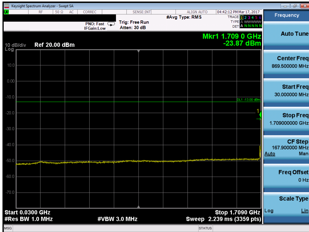
Plot 7-62. Conducted Spurious Plot (Band 4 – 15.0MHz QPSK – RB Size 1, RB Offset 0 – Low Channel)
