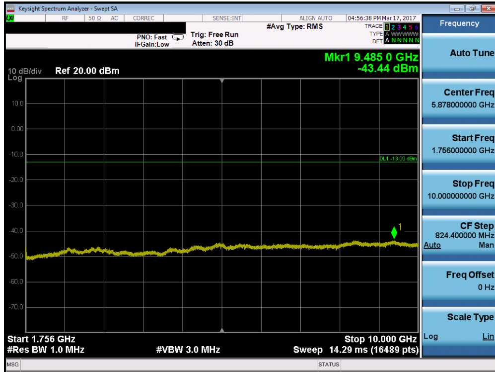
Plot 7-69. Conducted Spurious Plot (Band 4 – 15.0MHz QPSK – RB Size 1, RB Offset 0 – High Channel)
