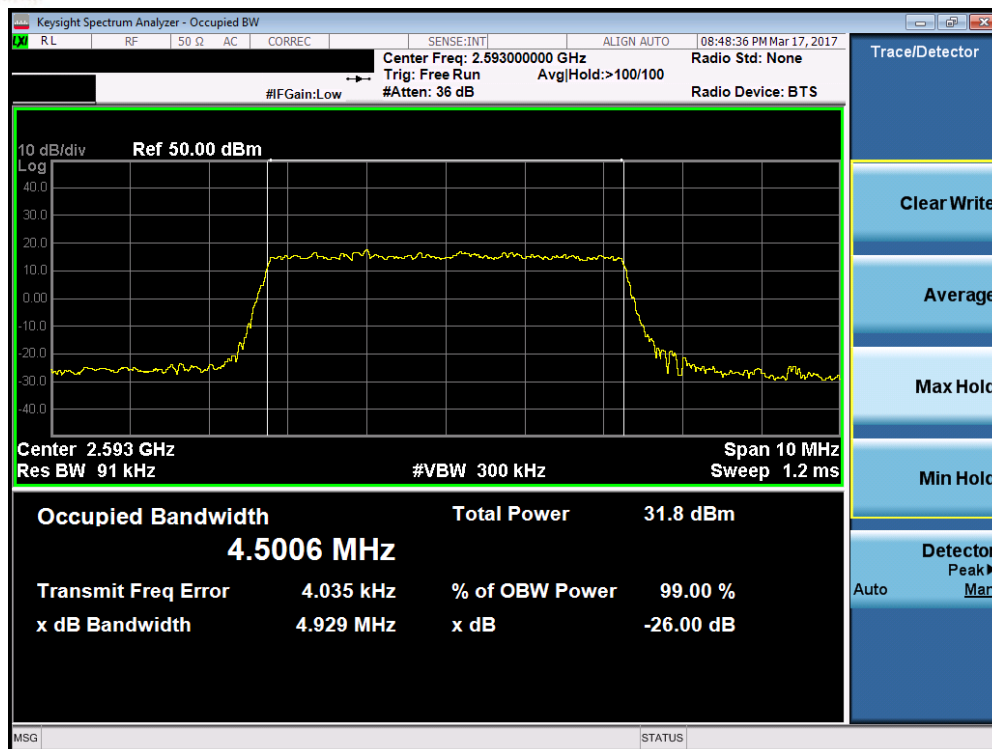
Plot 7-33. Occupied Bandwidth Plot (Band 41 – 5.0MHz QPSK – RB Size 25)
