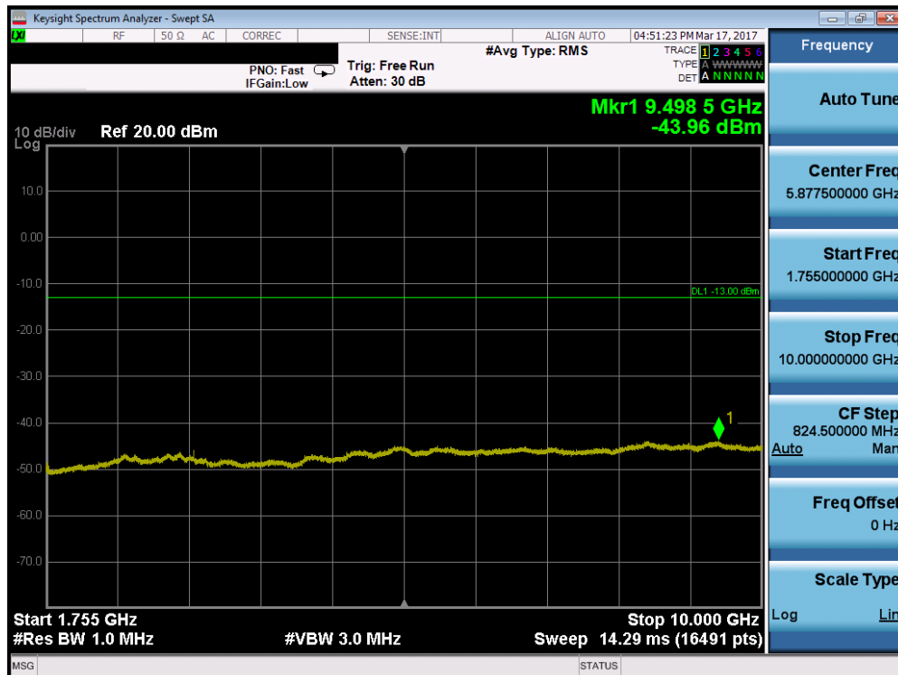
Plot 7-66. Conducted Spurious Plot (Band 4 – 15.0MHz QPSK – RB Size 1, RB Offset 0 – Mid Channel)
