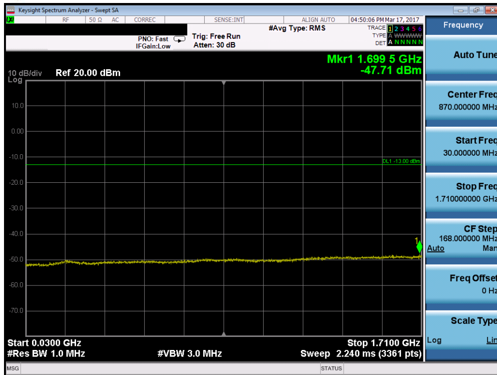
Plot 7-65. Conducted Spurious Plot (Band 4 – 15.0MHz QPSK – RB Size 1, RB Offset 0 – Mid Channel)
