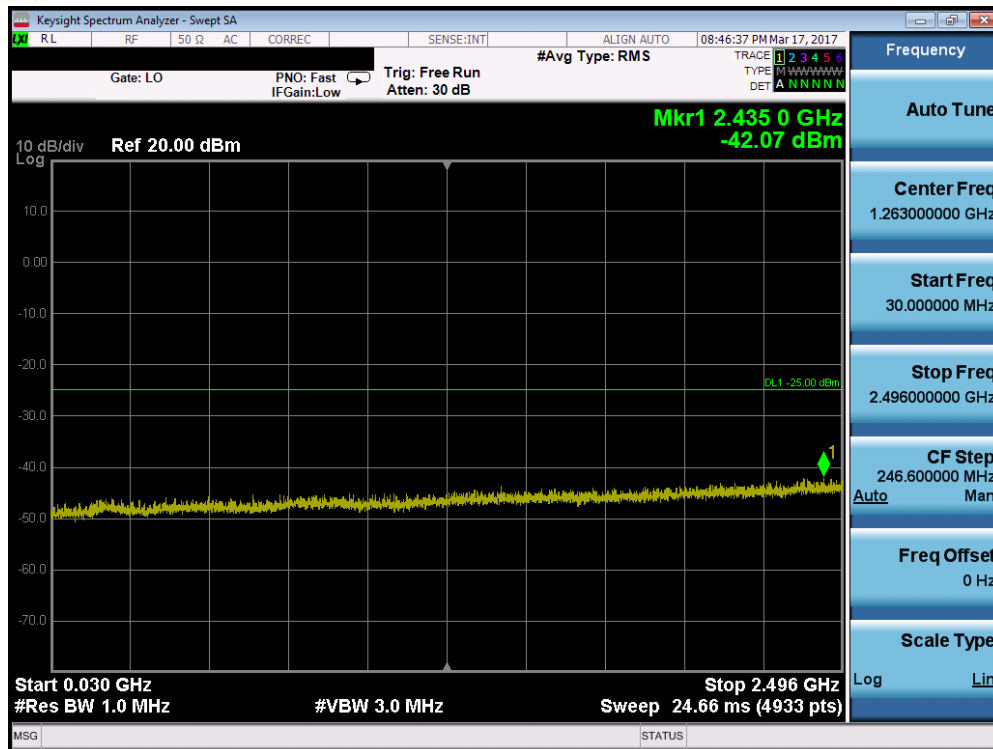
Plot 7-77. Conducted Spurious Plot (Band 41 – 10.0MHz QPSK – RB Size 1, RB Offset 0 – High Channel)
