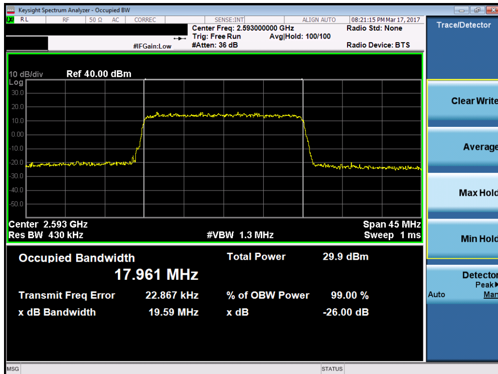
Plot 7-40. Occupied Bandwidth Plot (Band 41 – 20.0MHz 16-QAM – RB Size 100)
