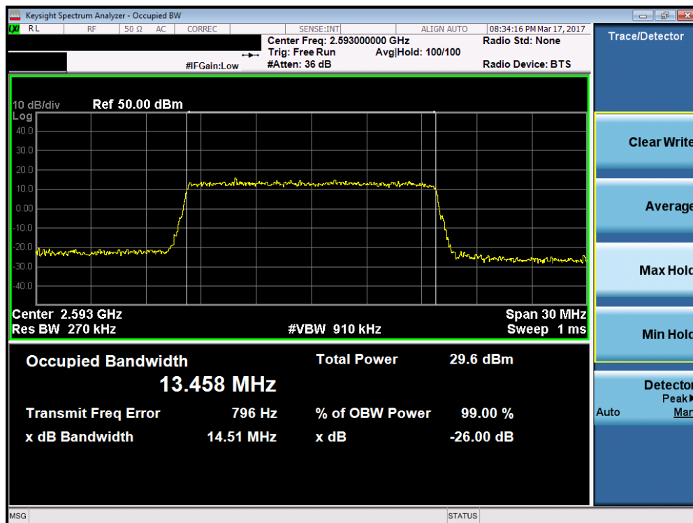
Plot 7-38. Occupied Bandwidth Plot (Band 41 – 15.0MHz 16-QAM – RB Size 75)
