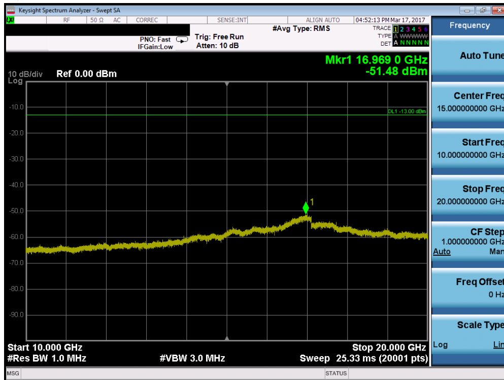
Plot 7-67. Conducted Spurious Plot (Band 4 – 15.0MHz QPSK – RB Size 1, RB Offset 0 – Mid Channel)
