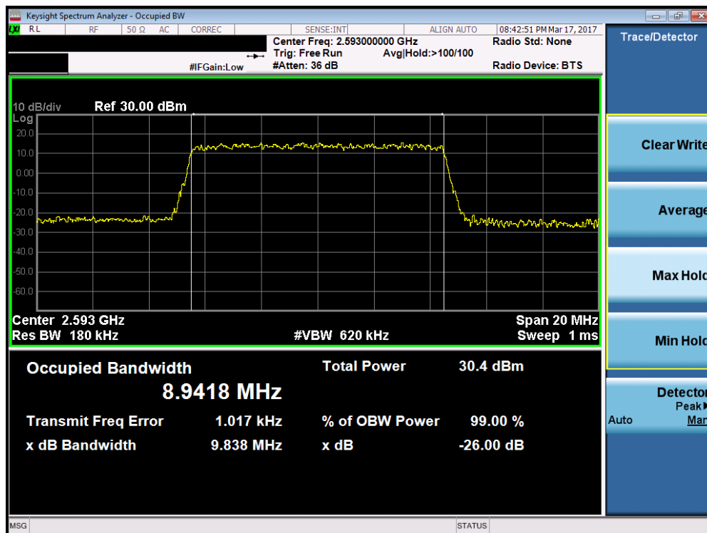
Plot 7-36. Occupied Bandwidth Plot (Band 41 – 10.0MHz 16-QAM – RB Size 50)
