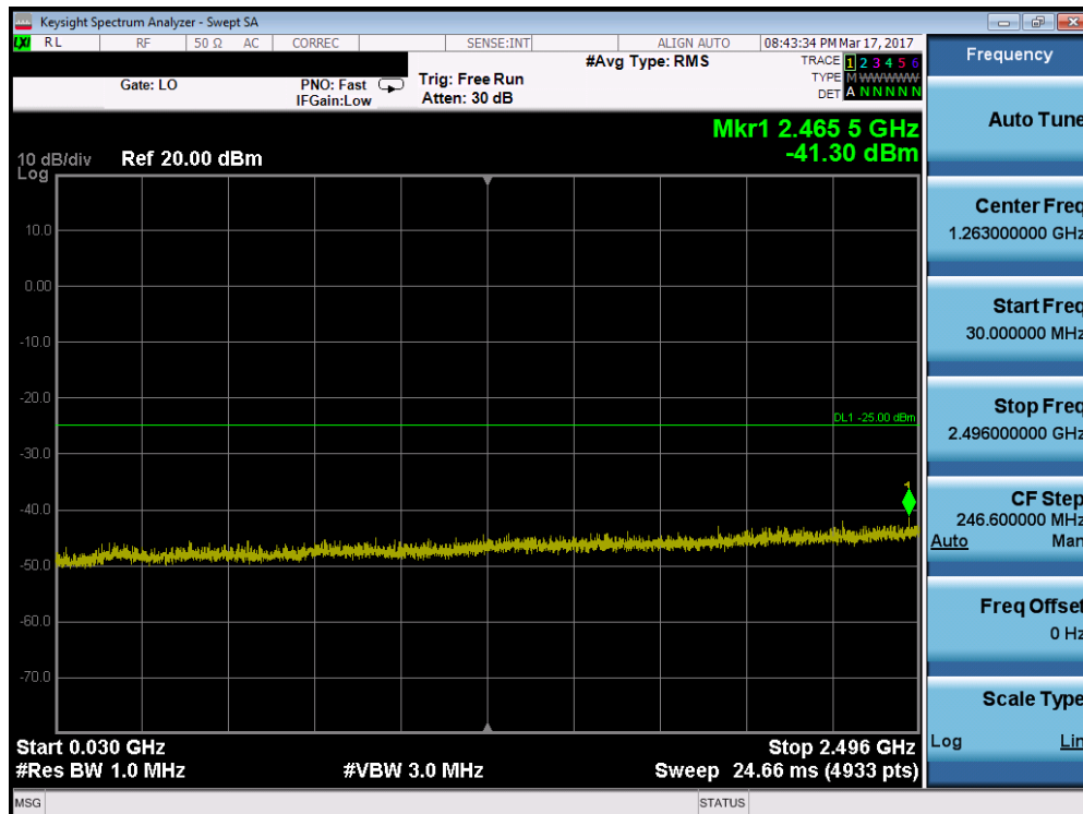
Plot 7-74. Conducted Spurious Plot (Band 41 – 10.0MHz QPSK – RB Size 1, RB Offset 0 – Mid Channel)
