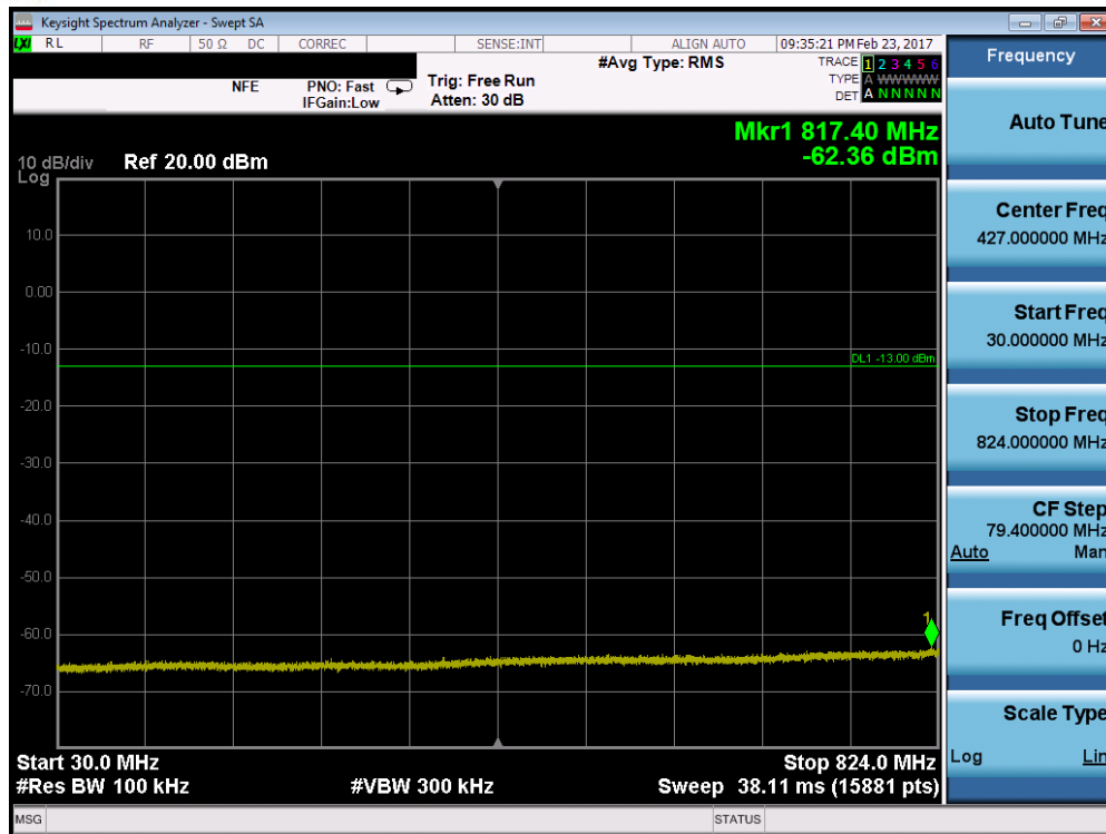
Plot 7-59. Conducted Spurious Plot (Band 5 – 5.0MHz QPSK – RB Size 1, RB Offset 0 – High Channel)
