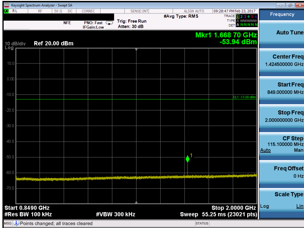
Plot 7-57. Conducted Spurious Plot (Band 5 – 5.0MHz QPSK – RB Size 1, RB Offset 0 – Mid Channel)
