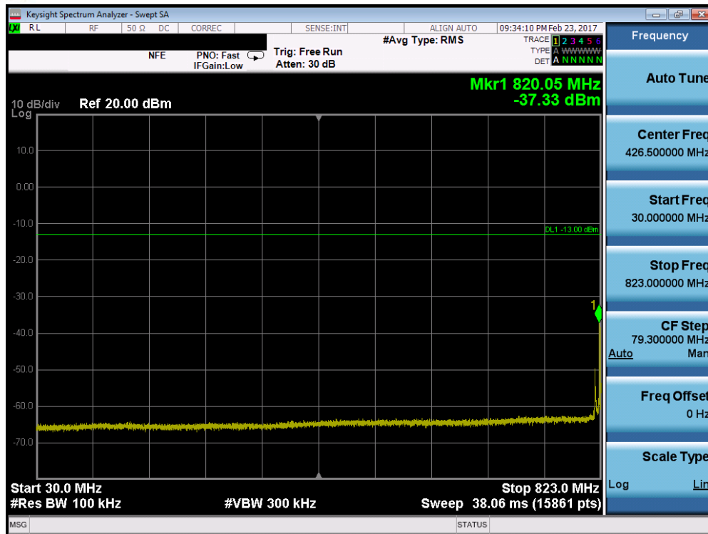
Plot 7-53. Conducted Spurious Plot (Band 5 – 5.0MHz QPSK – RB Size 1, RB Offset 0 – Low Channel)
