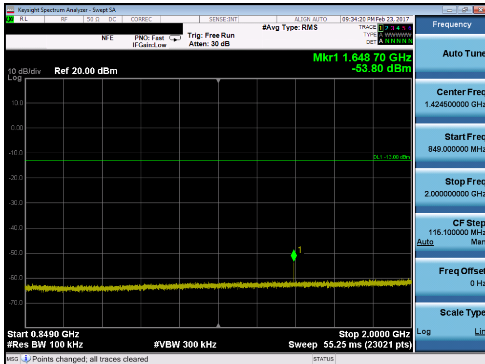
Plot 7-54. Conducted Spurious Plot (Band 5 – 5.0MHz QPSK – RB Size 1, RB Offset 0 – Low Channel)
