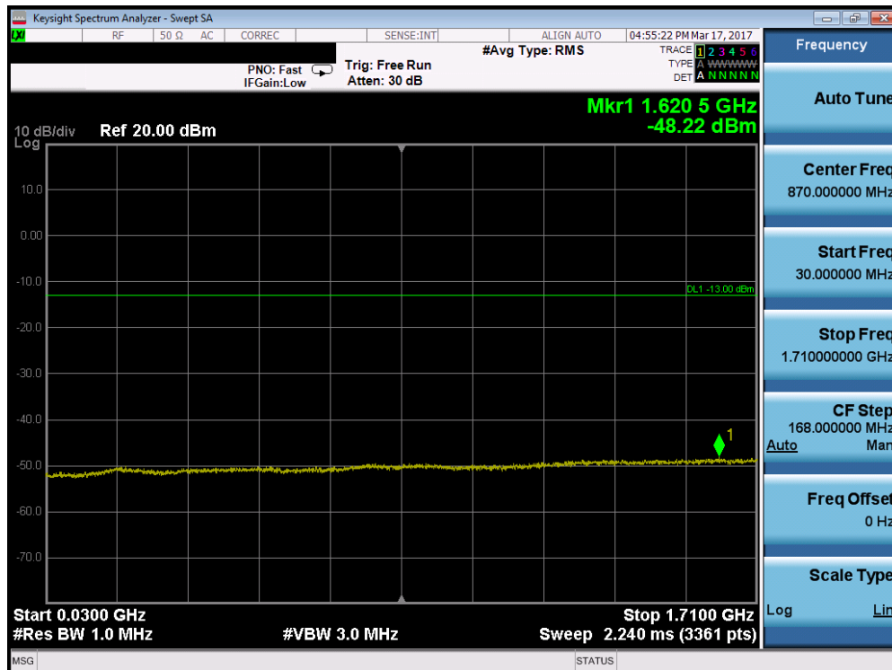
Plot 7-68. Conducted Spurious Plot (Band 4 – 15.0MHz QPSK – RB Size 1, RB Offset 0 – High Channel)
