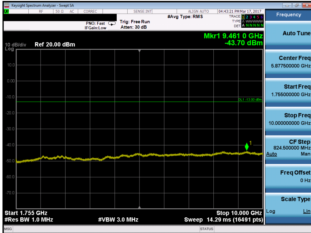
Plot 7-63. Conducted Spurious Plot (Band 4 – 15.0MHz QPSK – RB Size 1, RB Offset 0 – Low Channel)
