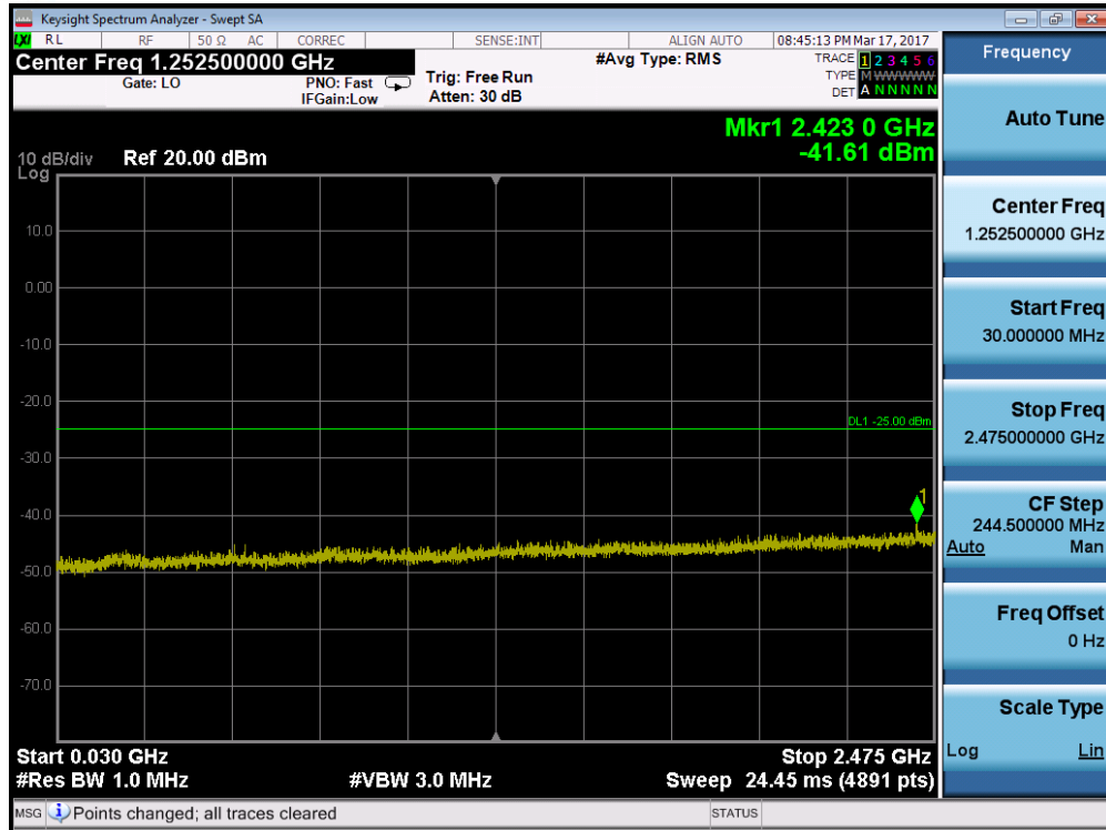
Plot 7-71. Conducted Spurious Plot (Band 41 – 10.0MHz QPSK – RB Size 1, RB Offset 0– Low Channel)
