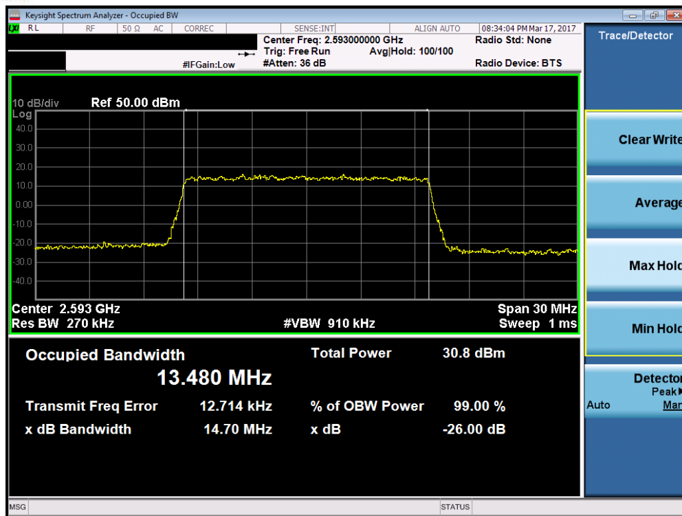
Plot 7-37. Occupied Bandwidth Plot (Band 41 – 15.0MHz QPSK – RB Size 75)
