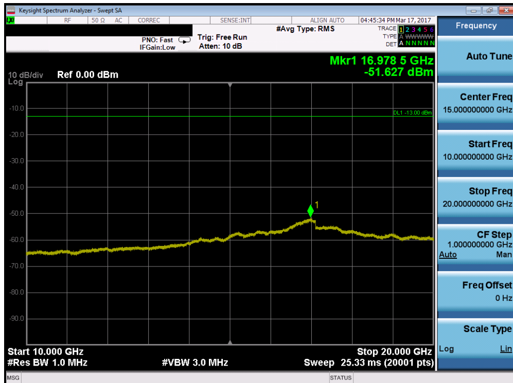
Plot 7-64. Conducted Spurious Plot (Band 4 – 15.0MHz QPSK – RB Size 1, RB Offset 0 – Low Channel)
