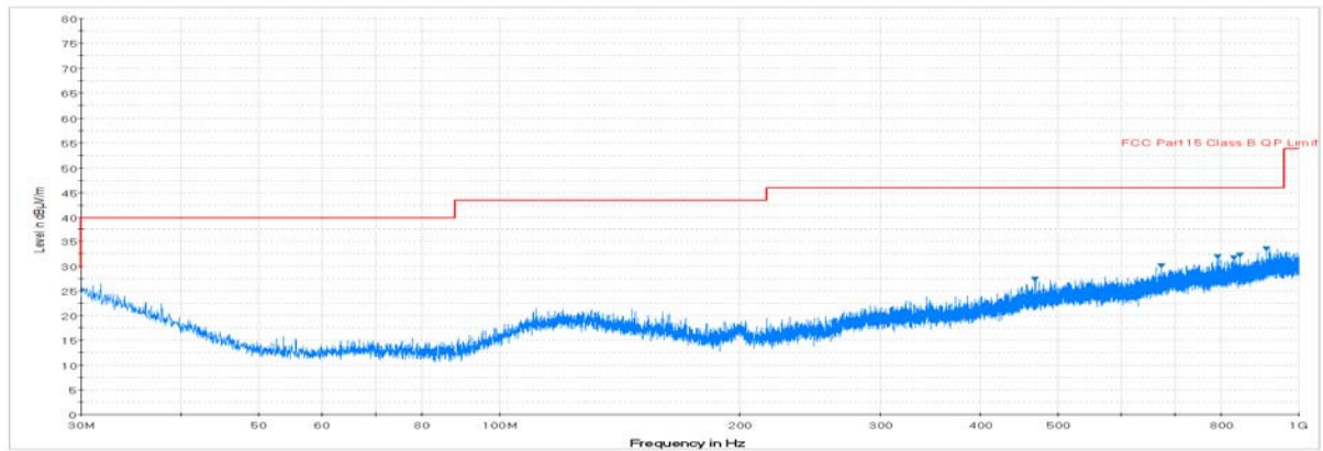
Plot 7-95. Radiated Spurious Plot below 1GHz (Pol. H)
