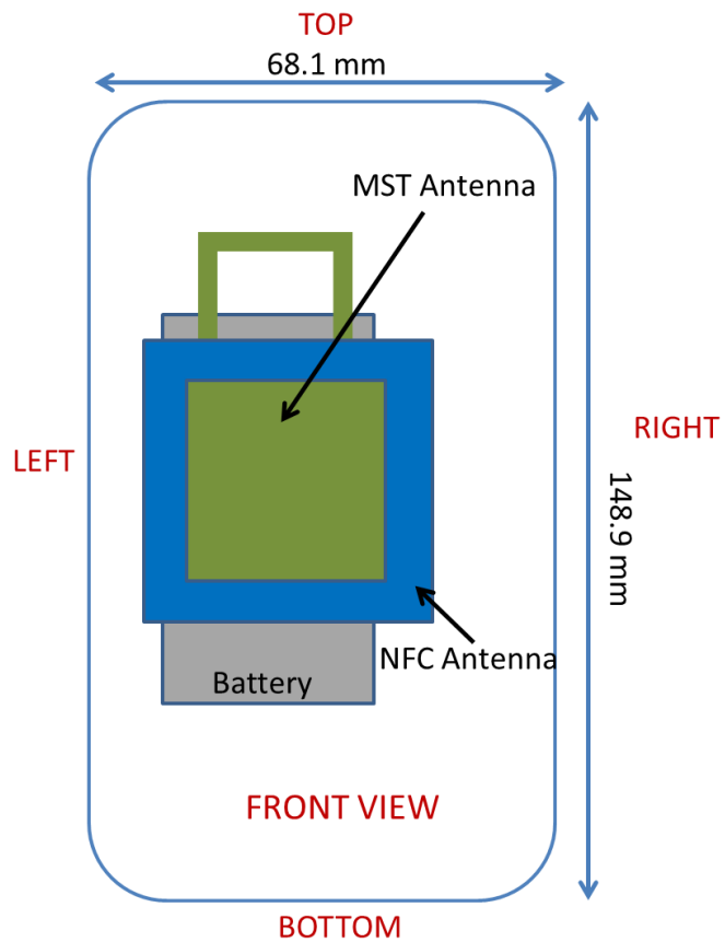
Figure F-2 NFC and MST Antenna Locations
