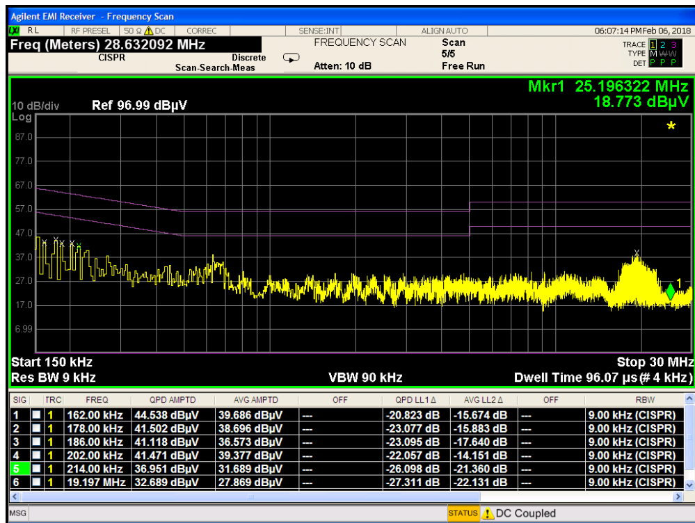
Plot 7-9. Line-Conducted Test Plot (N) RFID Antenna Terminated in 50Ω
