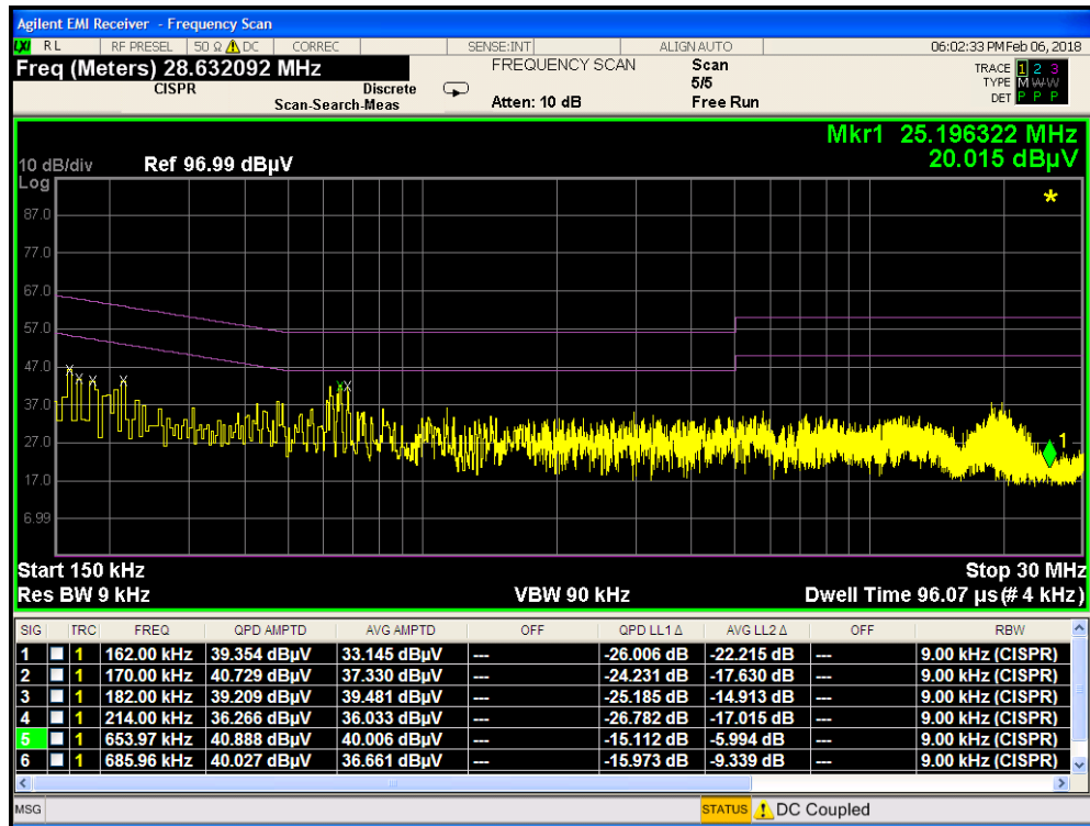
Plot 7-8. Line-Conducted Test Plot (L1) RFID Antenna Terminated in 50Ω
