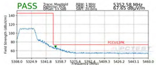
Plot 7-235. Radiated Upper Band Edge Plot (Peak – UNII Band 2A)
