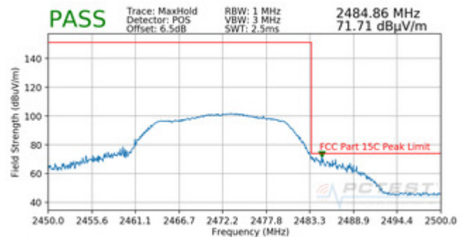
Plot 7-88. Radiated Restricted Upper Band Edge Measurement (Peak)
