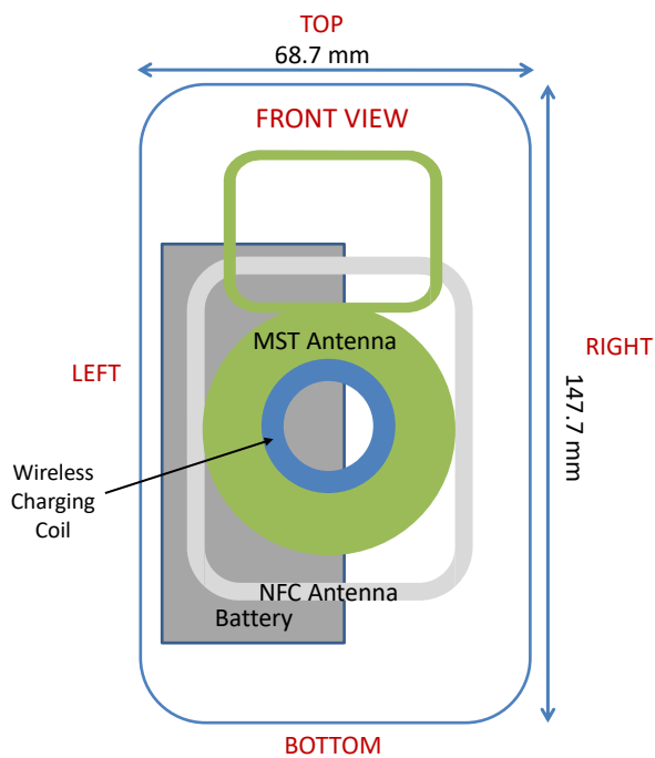
Figure F-2 NFC Antenna Locations
