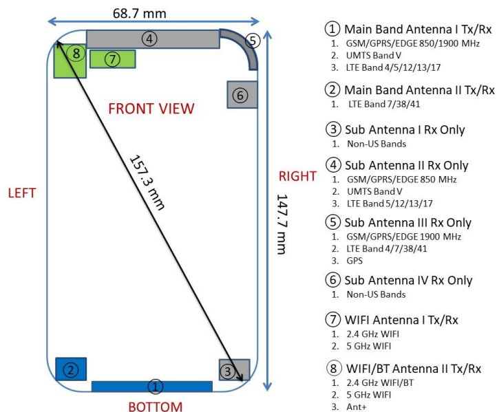
Figure F-1 DUT Antenna Locations
