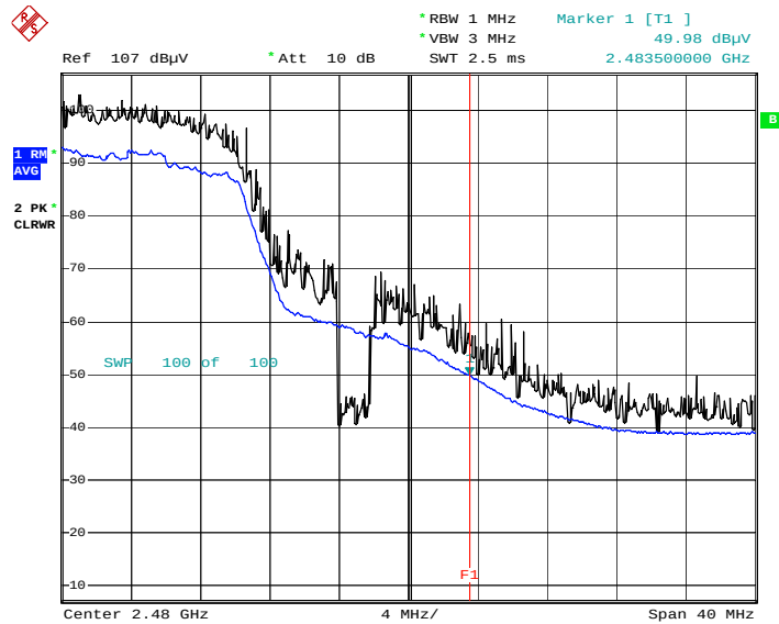
Radiated Restricted Band Edges plot – Average Reading (802.11g Ch.11)
