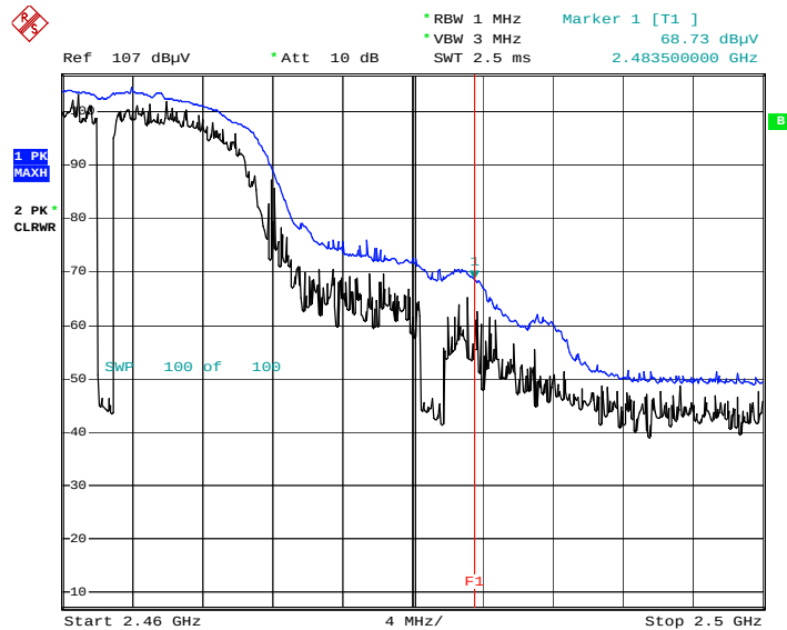
Radiated Restricted Band Edges plot – Peak Reading (802.11g Ch.11)
