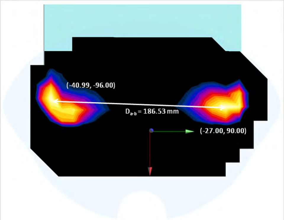
Figure 10-5 Peak SAR Locations for Body Back Side at 0.0 cm GPRS 1900 and 2.4 GHz WLAN MIMO
