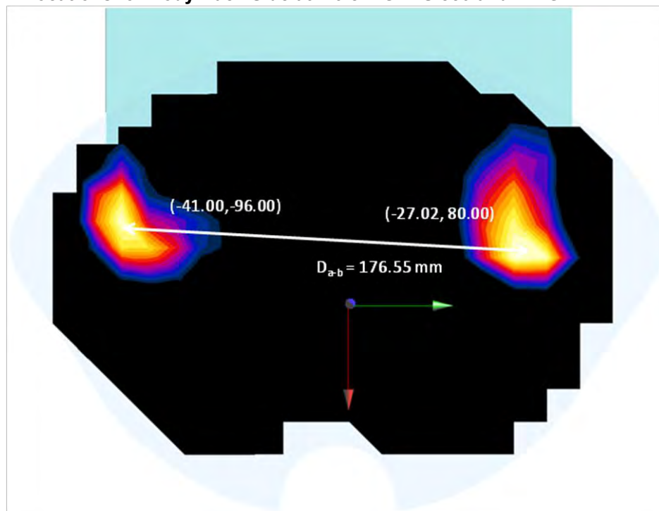
Figure 10-6 Peak SAR Locations for Body Back Side at 1.6 cm GPRS 850 and 2.4 GHz WLAN Antenna 1
