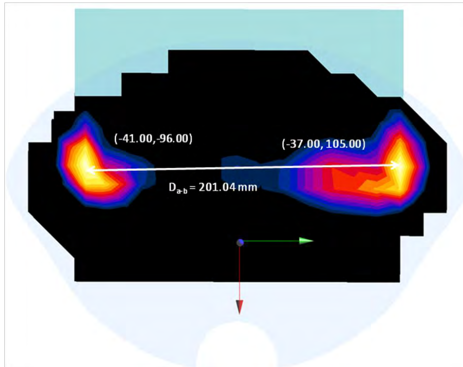
Figure 10-7 Peak SAR Locations for Body Back Side at 1.6 cm GPRS 1900 and 2.4 GHz WLAN Antenna 1
