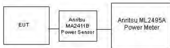
Figure 7-3 Power Measurement Setup for Bandwidths < 50 MHz
