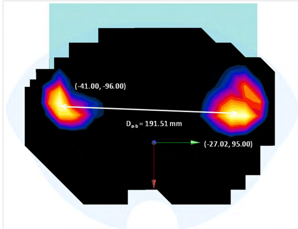
Figure 10-2 Peak SAR Locations for Body Back Side at 0.0 cm GPRS 850 and 2.4 GHz WLAN Antenna 2
