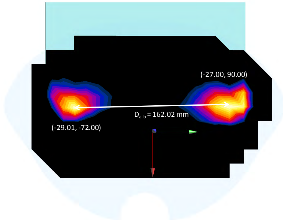
Figure 10-4 Peak SAR Locations for Body Back Side at 0.0 cm GPRS 1900 and 2.4 GHz WLAN Antenna 2
