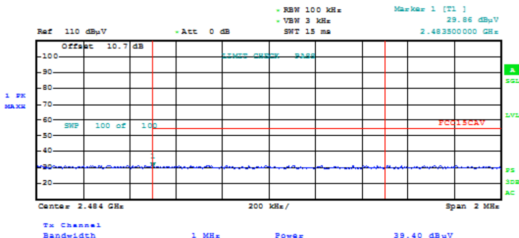
Plot 6-18. Radiated Restricted Upper Band Edge Measurement (Average)
