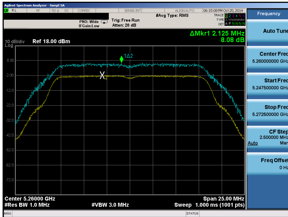
Plot 6-124. Peak Excursion Ratio Plot (802.11a (UNII Band 2A) – Ch. 52)
