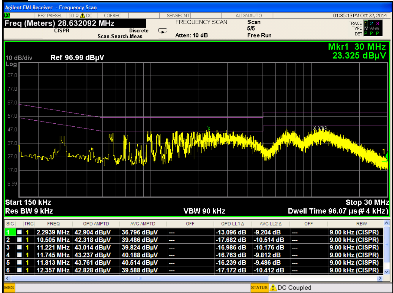
Plot 6-192. Line Conducted Plot with 802.11a UNII Band 1 (L1)
