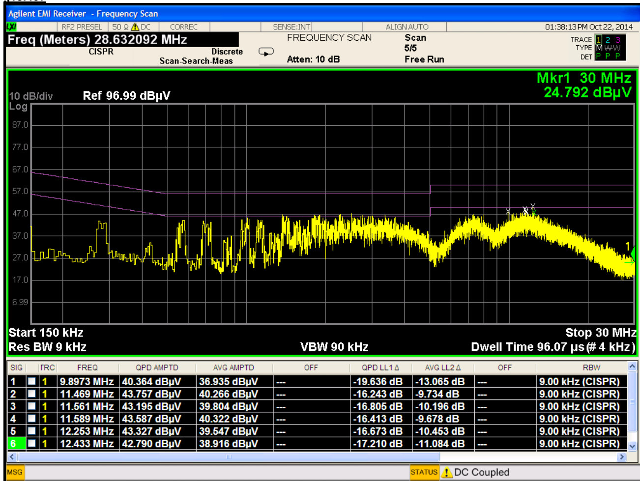
Plot 6-194. Line Conducted Plot with 802.11a UNII Band 2A (L1)
