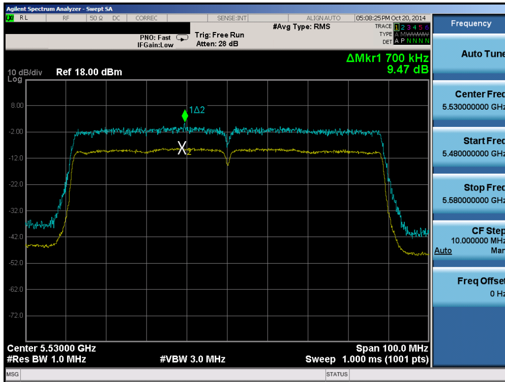
Plot 6-131. Peak Excursion Ratio Plot (80MHz BW 802.11ac (UNII Band 2C) – Ch. 106)
