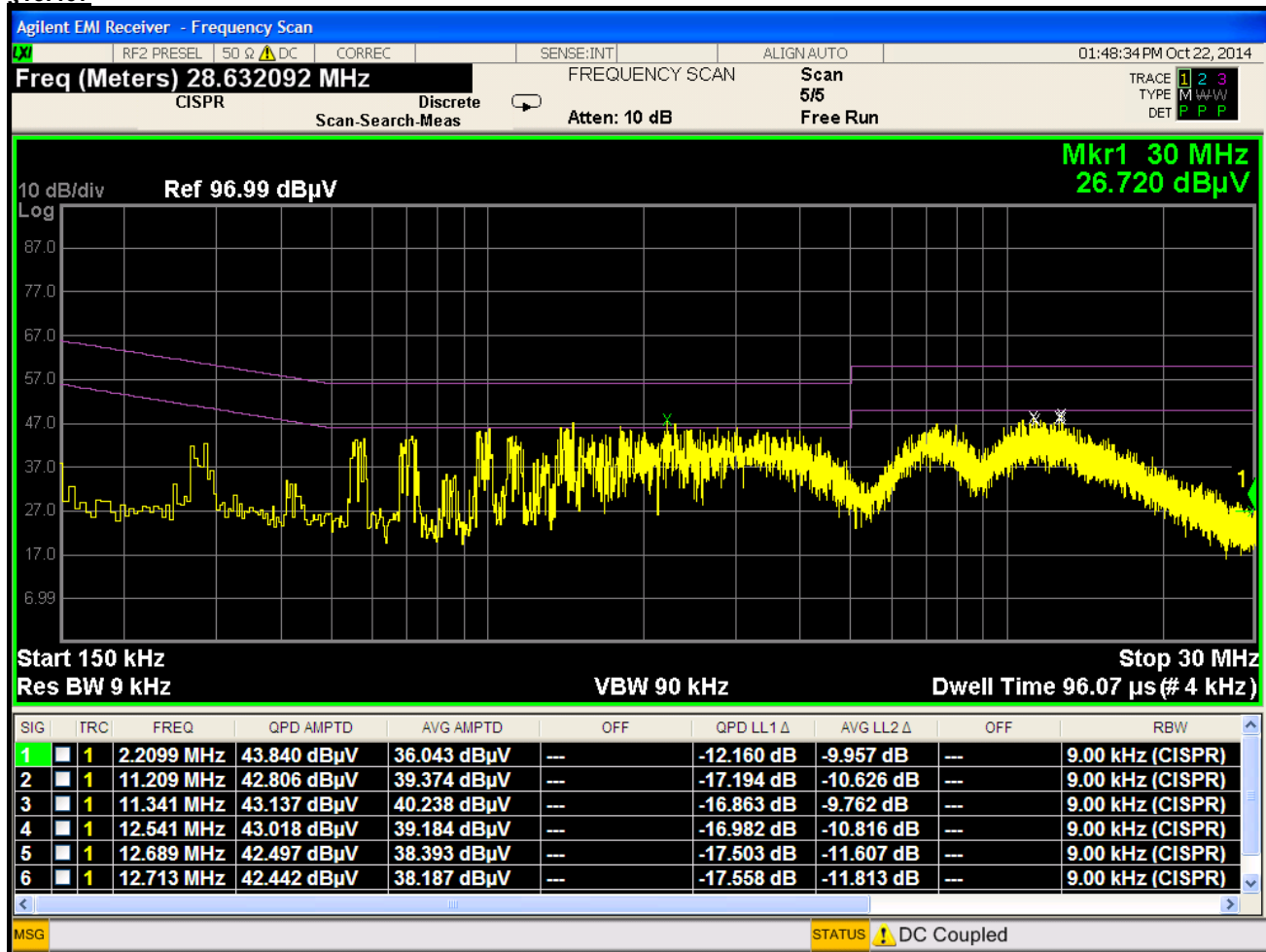
Plot 6-196. Line Conducted Plot with 802.11a UNII Band 2C (L1)
