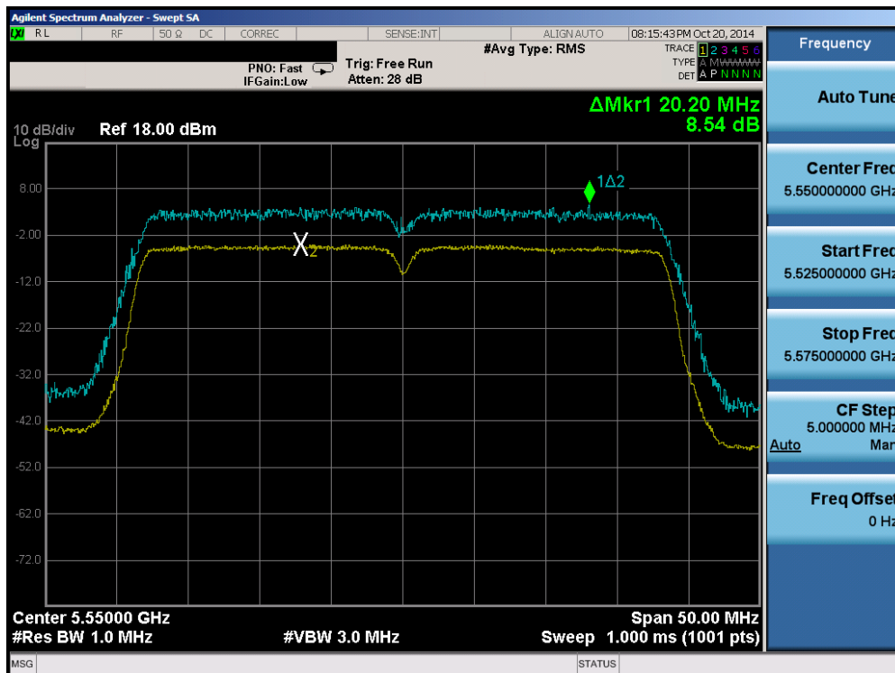
Plot 6-126. Peak Excursion Ratio Plot (40MHz BW 802.11n (UNII Band 2C) – Ch. 110)
