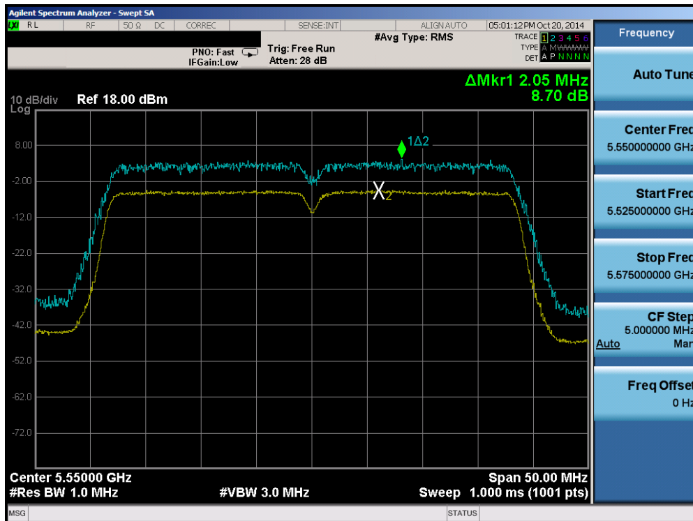
Plot 6-130. Peak Excursion Ratio Plot (40MHz BW 802.11n (UNII Band 2C) – Ch. 110)
