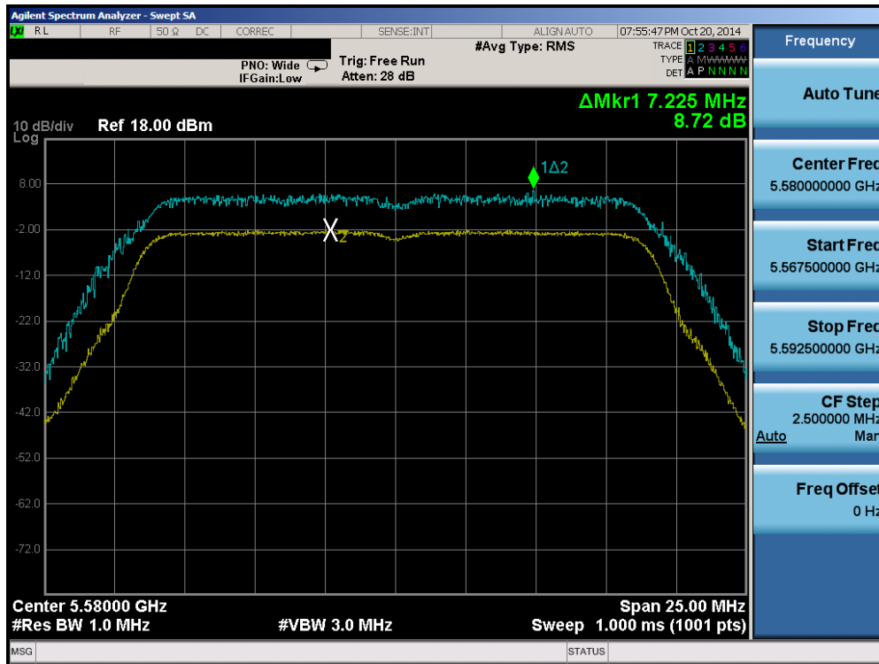
Plot 6-125. Peak Excursion Ratio Plot (20MHz BW 802.11n (UNII Band 2C) – Ch. 116)
