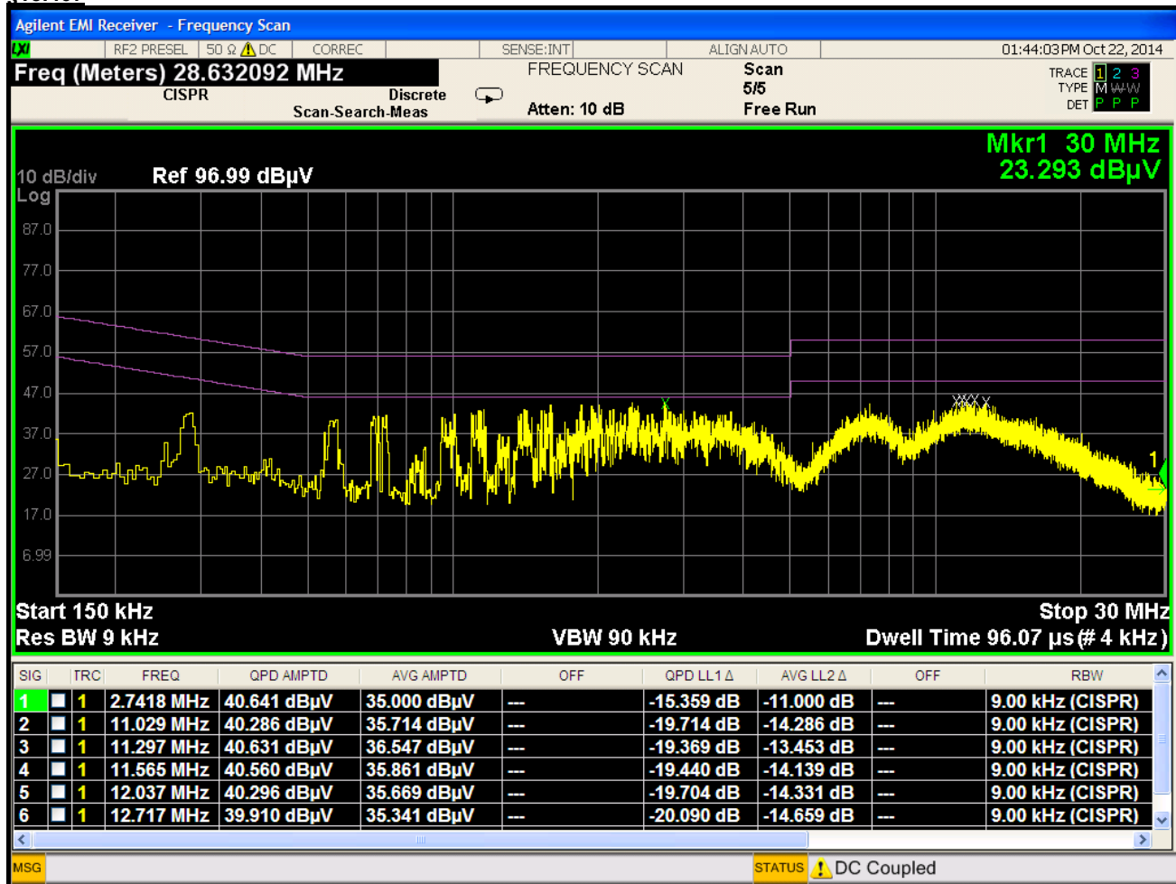
Plot 6-197. Line Conducted Plot with 802.11a UNII Band 2C (N)
