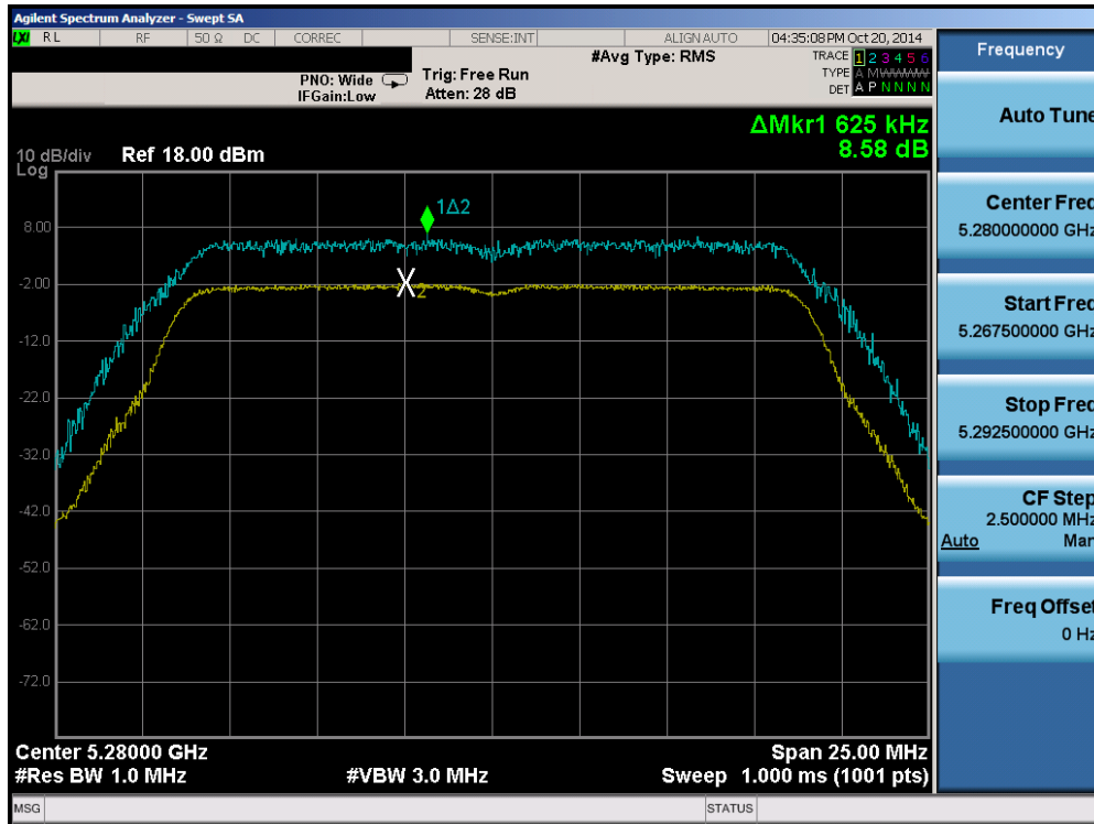
Plot 6-129. Peak Excursion Ratio Plot (20MHz BW 802.11n (UNII Band 2A) – Ch. 56)
