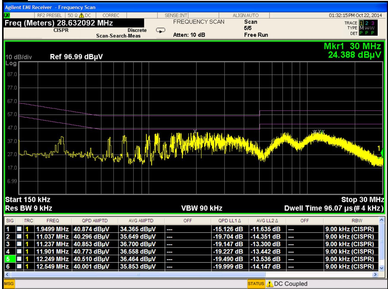
Plot 6-193. Line Conducted Plot with 802.11a UNII Band 1 (N)
