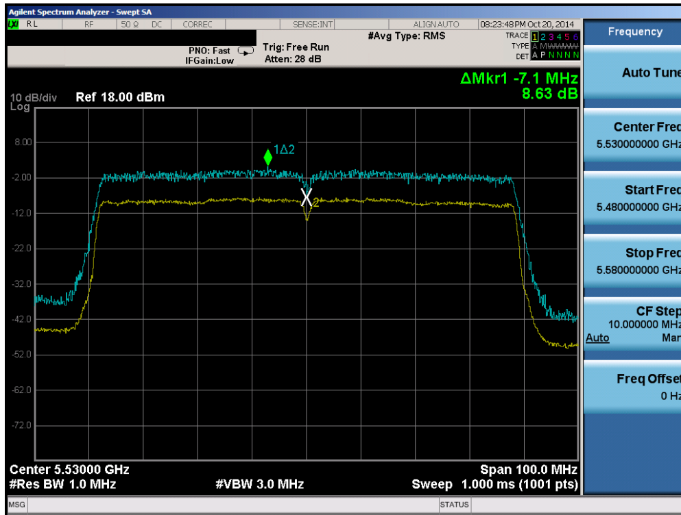
Plot 6-127. Peak Excursion Ratio Plot (80MHz BW 802.11ac (UNII Band 2C) – Ch. 106)
