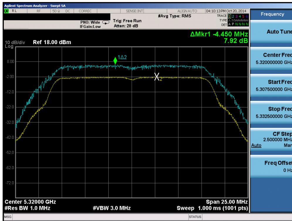
Plot 6-128. Peak Excursion Ratio Plot (802.11a (UNII Band 2A) – Ch. 64)
