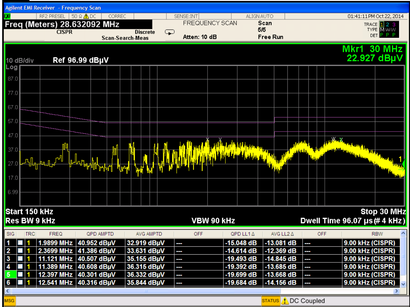
Plot 6-195. Line Conducted Plot with 802.11a UNII Band 2A (N)
