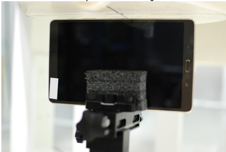
SAR Test Setup Photo 6: Right Edge at 0.5 cm
