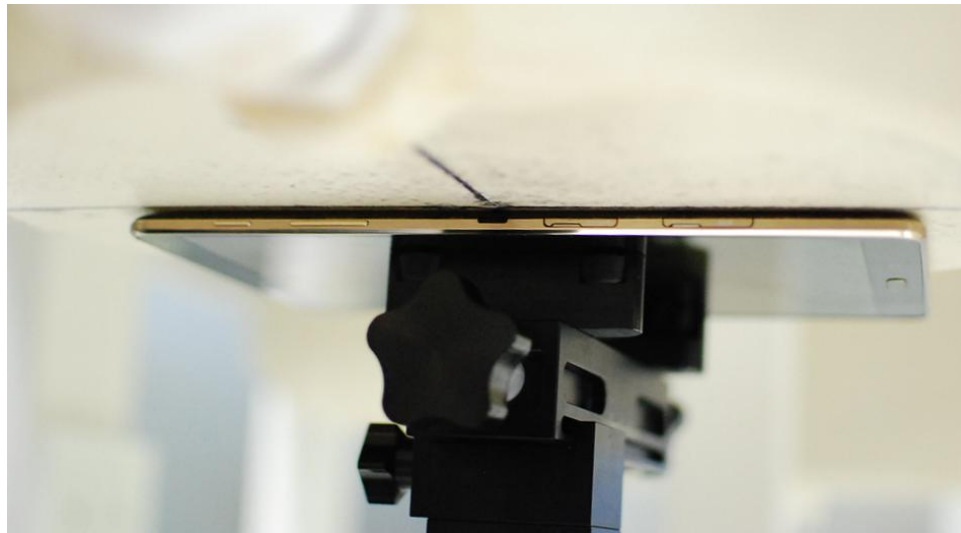
SAR Test Setup Photo 2: Back Side at 0.0 cm
